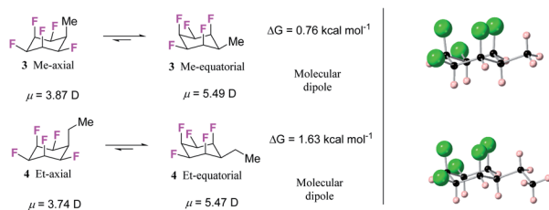
Fig. 4 (a) Calculated (M06L-D3/aug-cc-pVTZ level) equilibrium energies between axial/equatorial conformers of alkyl substituted all-cis 1,2,3,4,5,-pentafluorocyclohexanes 3 and 4 ; (b) solid state X-ray structures of 3 (upper) and 4 (lower). In each case the equatorial conformer is favoured.
