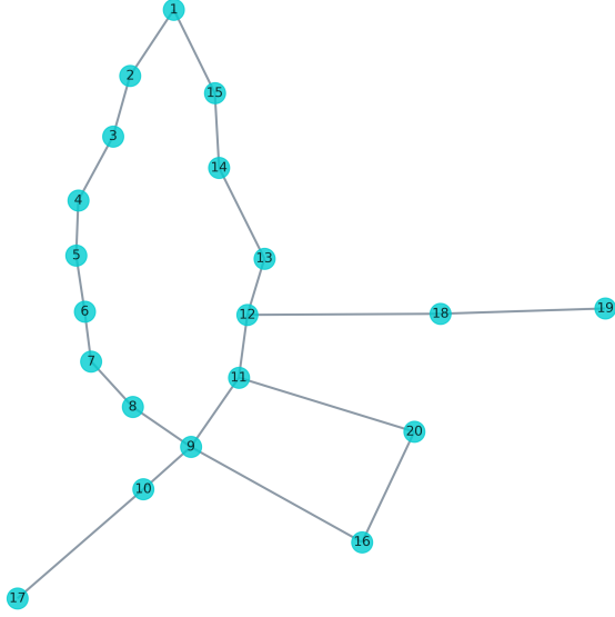
Fig. 2: New York Tunnels problem layout. Node 1 is the reservoir/source of water
