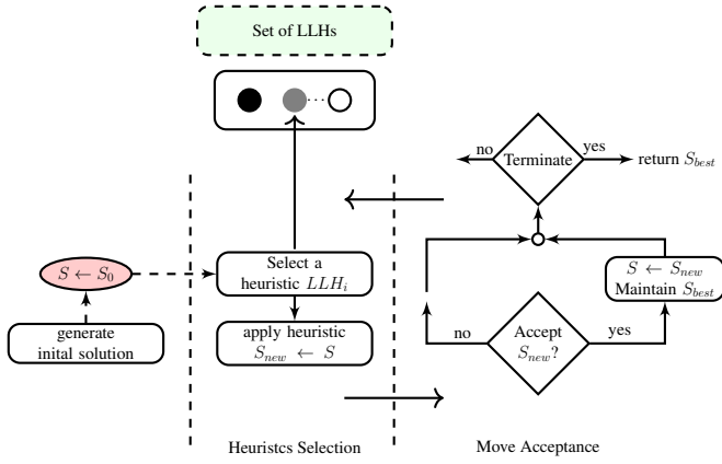
Fig. 1: A selection hyper-heuristic framework
