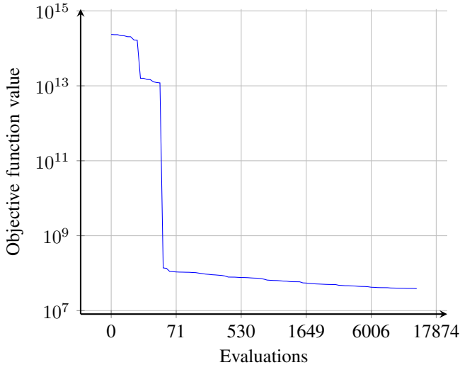
Fig. 4: Improvement of cost in terms of objective function value
