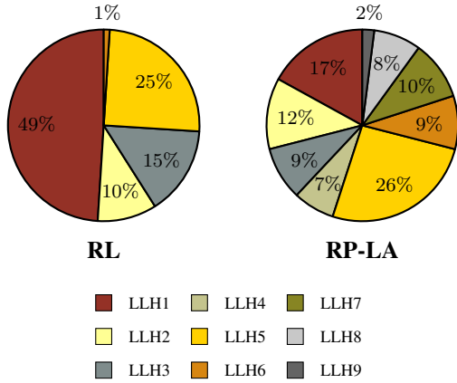
Fig. 3: Utilisation rate of each low level heuristics
