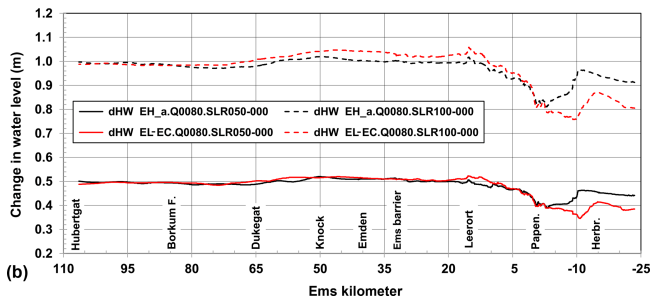
Figure 10. (a) Highest water levels along a longitudinal profile in the Ems estuary during EH_a (black lines) and EL (red lines) for SLR = 0 cm (solid lines), SLR = 50 cm (dotted lines) and SLR = 100 cm (dashed lines) for an open storm surge barrier and Q = 80 \text{ m}^3 \text{ s}^{-1} . (b) Differences in the highest water levels between simulations with and without SLR along the Ems estuary during EH_a (black lines) and EL (red lines) for Q = 80 \text{ m}^3 \text{ s}^{-1} (dashed lines for SLR = 100 cm, solid lines for SLR = 50 cm). The storm surge barrier is open.
