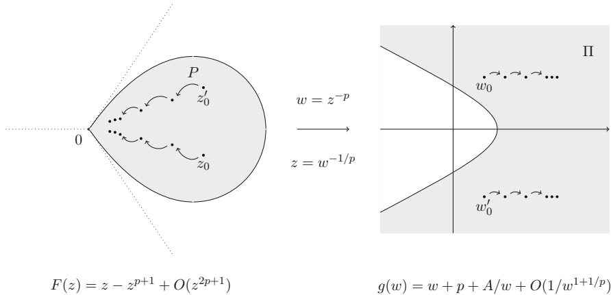
Fig. 3 Conjugate orbits: on the left two orbits in P under F and on the right the corresponding orbits in \Pi under g (in this figure, p = 3 )
