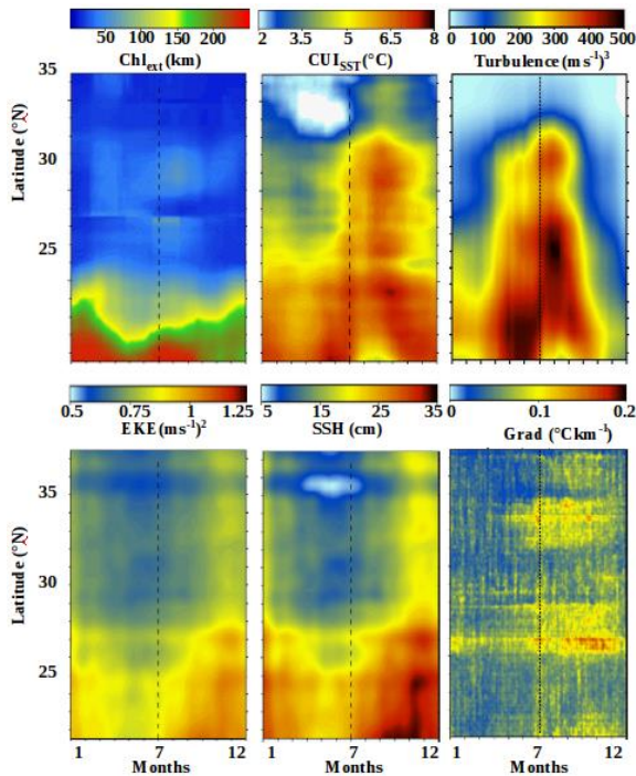
Fig.4. Hovmoller diagrams of the seasonal variability off the mesoscale indices along the Moroccan Atlantic coast
