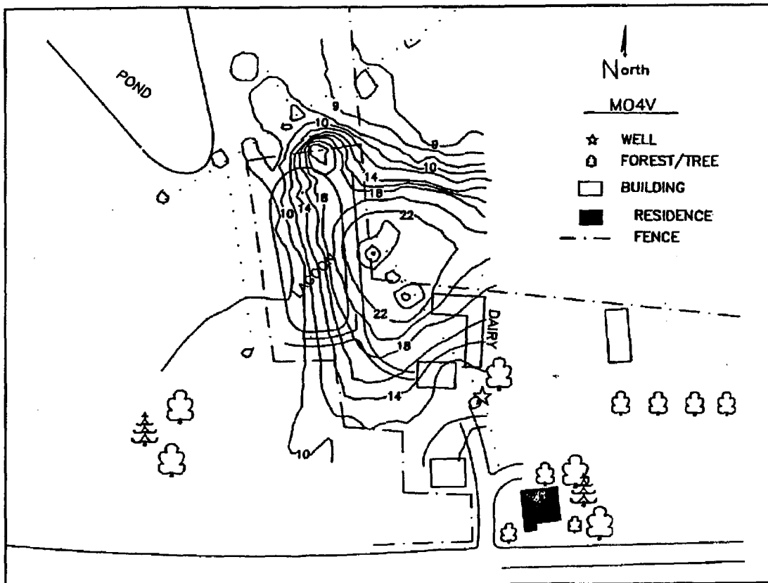
Figure 1. Survey of deep (vertical dipole) EM conductivities in mS/m at MO-4.
