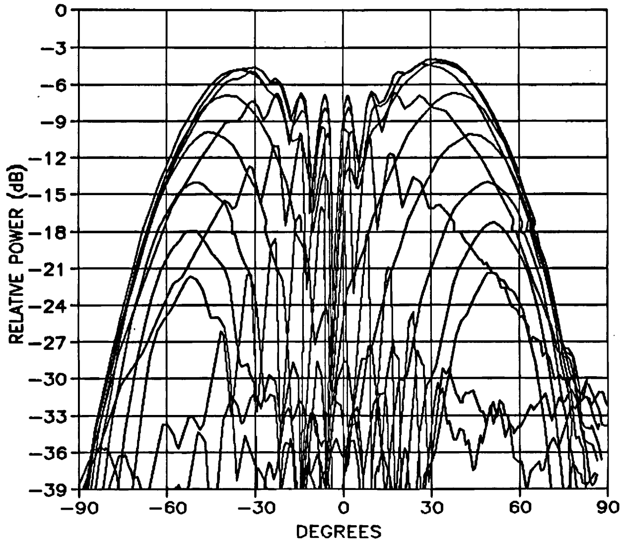
Figure 4. Display of azimuth antenna cut data for Contractor WEST.
