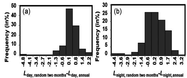
Fig. 3 — (a) & (b): Frequency histogram of calculated error from long-term annual average value for L_{day} and L_{night} for random two months' noise monitoring strategy for industrial zone.
