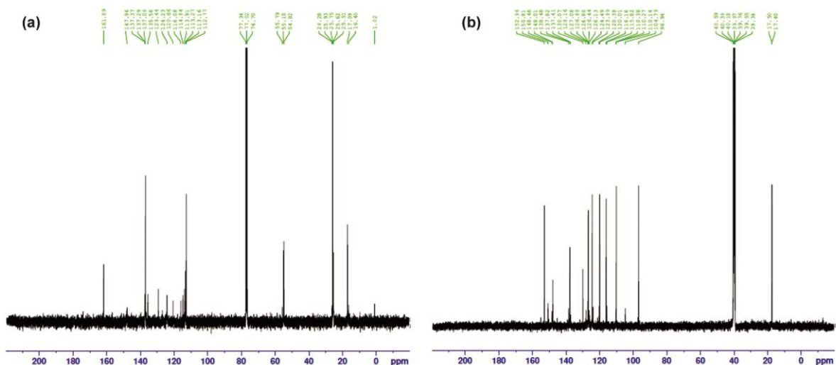
Fig. 2 — 13 C-NMR spectra of (a) L 1 and (b) L 2
