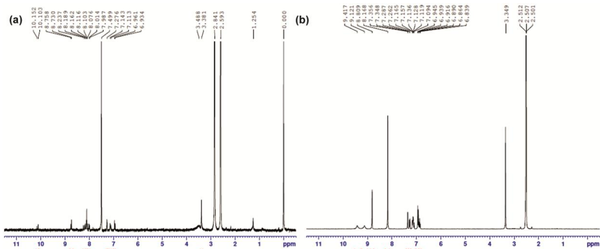
Fig. 1 — 1 H-NMR spectra of (a) L 1 and (b) L 2
