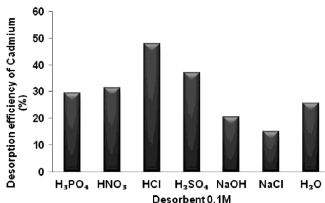
Fig. 9 — Desorption of cadmium from metal loaded biosorbent S. myriocystum .
