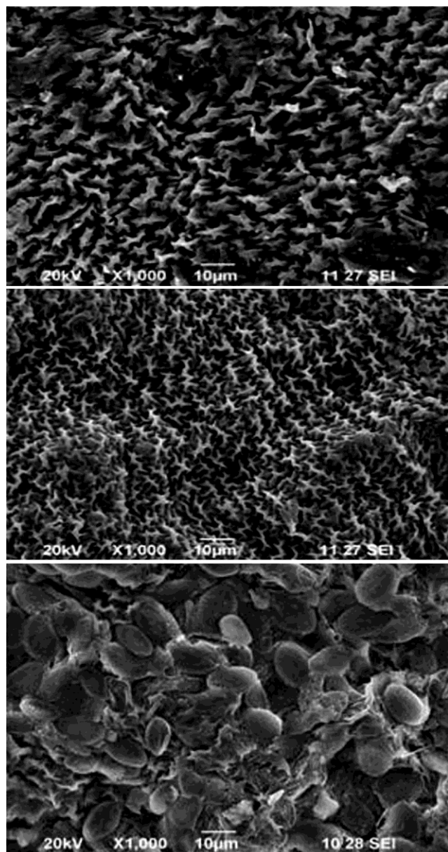
Fig. 7. (a) Scanning electron micrographs of S. myriocystum before metalbiosorption. (b) Energy dispersive X-ray (EDAX) spectrum of S. myriocystum before metalbiosorption, (b) Scanning electron micrographs of S. myriocystum after pretreatment with HCl. (b) Energy dispersive X-ray (EDAX) spectrum of S. myriocystum after pretreatment with HCl & (c) Scanning electron micrographs of S. myriocystum after \text{Cd}^{2+} biosorption. (b) Energy dispersive X-ray (EDAX) spectrum of S. myriocystum after \text{Cd}^{2+} biosorption.
