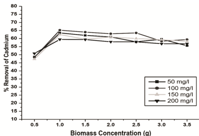
Fig. 2 — Effect of biomass concentration on \text{Cd}^{2+} biosorption efficiency (initial concentration 50, 100, 150, 200 mg/L, pH 5, contact time 30 min, agitation speed 150 rpm, temp 37^\circ\text{C} , adsorbent dose 0.5 – 3.5 g/L). 200 mg/L, pH 5, contact time (10 min to 180 min), agitation speed 150 rpm, temp 37^\circ\text{C} , 200 mg/L, pH 5, contact time 90 min, agitation speed 150 rpm, temp 20\text{--}50^\circ\text{C} , adsorbent dose 1.0 g/L).
