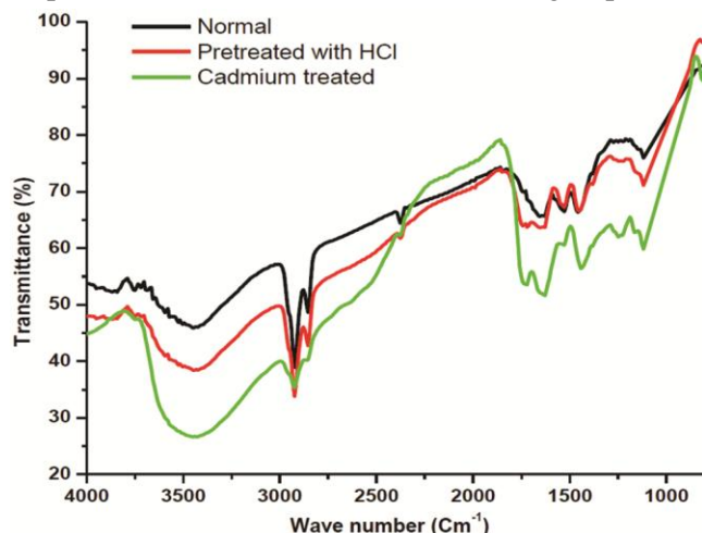
Fig. 8 — FT-IR spectrum of normal, pretreated and cadmium treated biomass.
