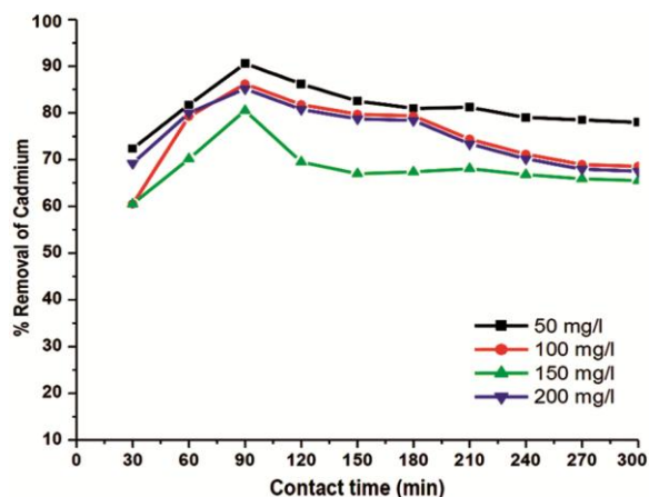
Fig. 3 — Effect of contact time on \text{Cd}^{2+} biosorption efficiency (initial concentration 50, 100, 150, adsorbent dose 1.0 g/L).
