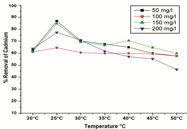
Fig. 4 — Effect of temperature on \text{Cd}^{2+} biosorption efficiency (initial concentration 50, 100, 150, adsorbent dose 1.0 g/L).
