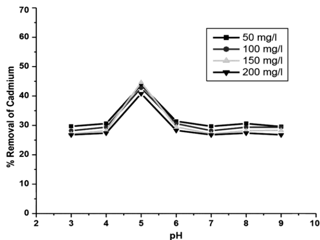
Fig. 1 — Effect of solution pH on Cd 2+ biosorption efficiency (initial concentration 50, 100, 150, 200 mg/L, pH 3-9, contact time 30 min, agitation speed 150 rpm, temp 37°C, adsorbent dose 0.5 g/L).
