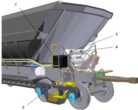
Simulation model of a iron ore carriage
