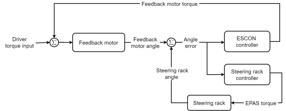
Closed-loop angular control strategy
