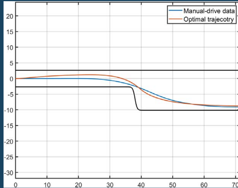
Manual vs. optimal trajectory
