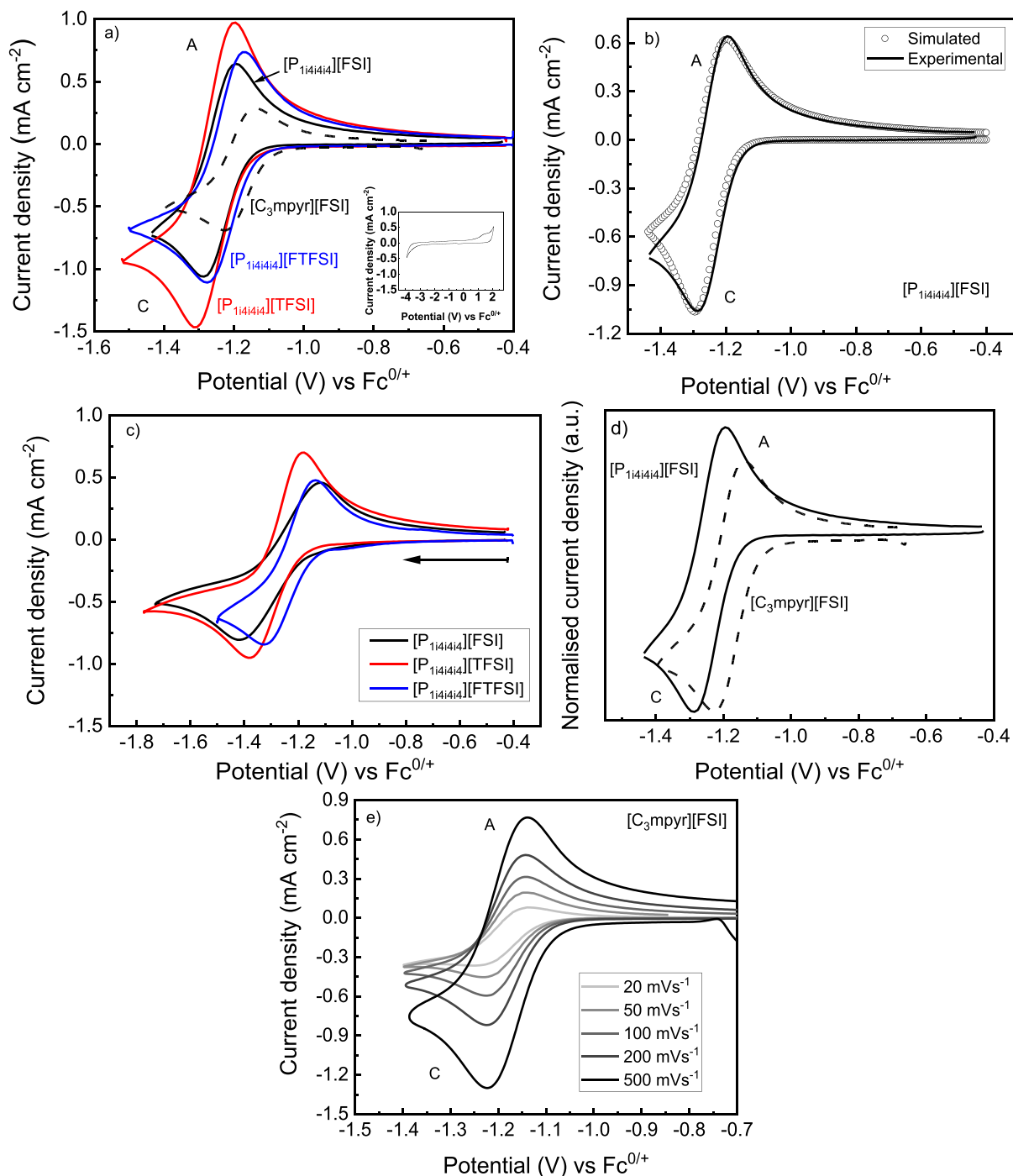
Fig. 1. Cyclic voltammograms obtained in O_2 -saturated for a) [P_{1141414}]^+ -ILs at a GC electrode (inset: electrochemical window [P_{1141414}]^+[FSI] ), b) experimental and simulated data for [P_{1141414}]^+[FSI] , c) [P_{1141414}]^+ -based ILs at a Au electrode, d) normalised cyclic voltammograms and e) scan rate dependence in [C_3mpyr]^+[FSI] at a GC electrode. Temperature: 60 °C, Scan rate: 100 mV s^{-1} .
