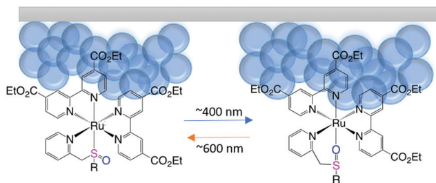
Scheme 1 Schematic illustration showing the reversible photoisomerization of Ru(deeb) 2 PySO-R, (R = iPr) attached to a mesoporous surface.
