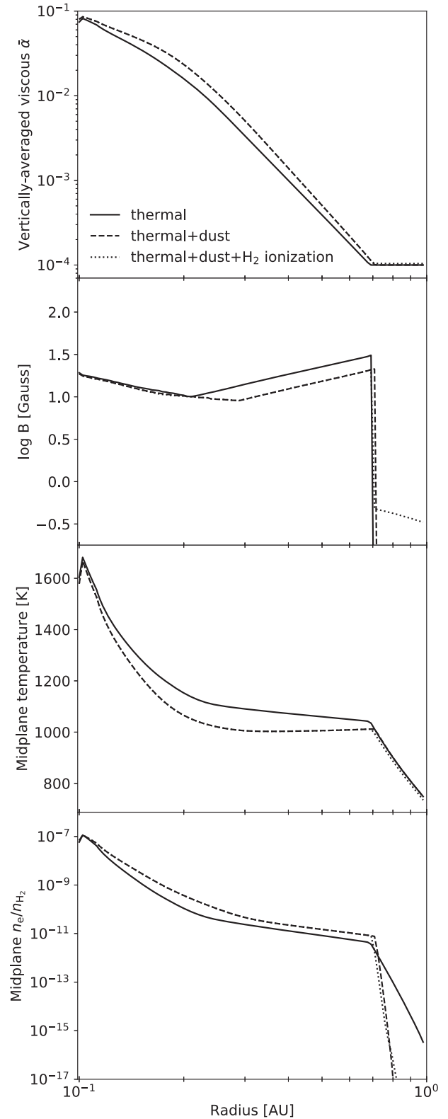
Figure 10. Vertically averaged viscous parameter ( \bar{\alpha} ), MRI-generated magnetic field strength ( B ), mid-plane temperature, and the mid-plane free electron fraction ( n_e/n_{\text{H}_2} ) as functions of radius, for a model with thermal ionization only, a model with thermal ionization and dust effects, and a model which also includes realistic non-thermal sources of ionization of \text{H}_2 ( \zeta = \zeta_{\text{R}} + \zeta_{\text{CR}} + \zeta_{\text{X}} ). The disc structure is quantitatively similar in all three models; however, the main sources of ionization in the models with dust are thermionic and ion emission. See Section 3.2.1.
