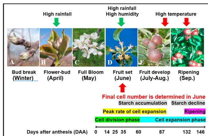
Fig. 8. The influence of preharvest weather (rainfall, humidity and temperature) during specific stages of growth and fruit development of apples. Bud break occurs during winter (November to March) (A), flower bud during April (B), full bloom during May (C), fruit set during June (D), fruit development during July–August (E) and ripening in September (F). The cell division phase occurs after full bloom (from May to June) and the cell enlargement phase occurs from fruit set to ripening (June–September).
