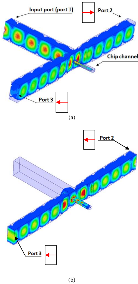
Fig. 1. E-field distribution of a) signal division when exciting port 1 or combination of signals injected in port 2 and 3 with 180 degrees phase difference and b) in-phase excitation of port 2 and 3 with signal of equal amplitude and phase. The red arrows correspond to the E-field orientation in each port.
