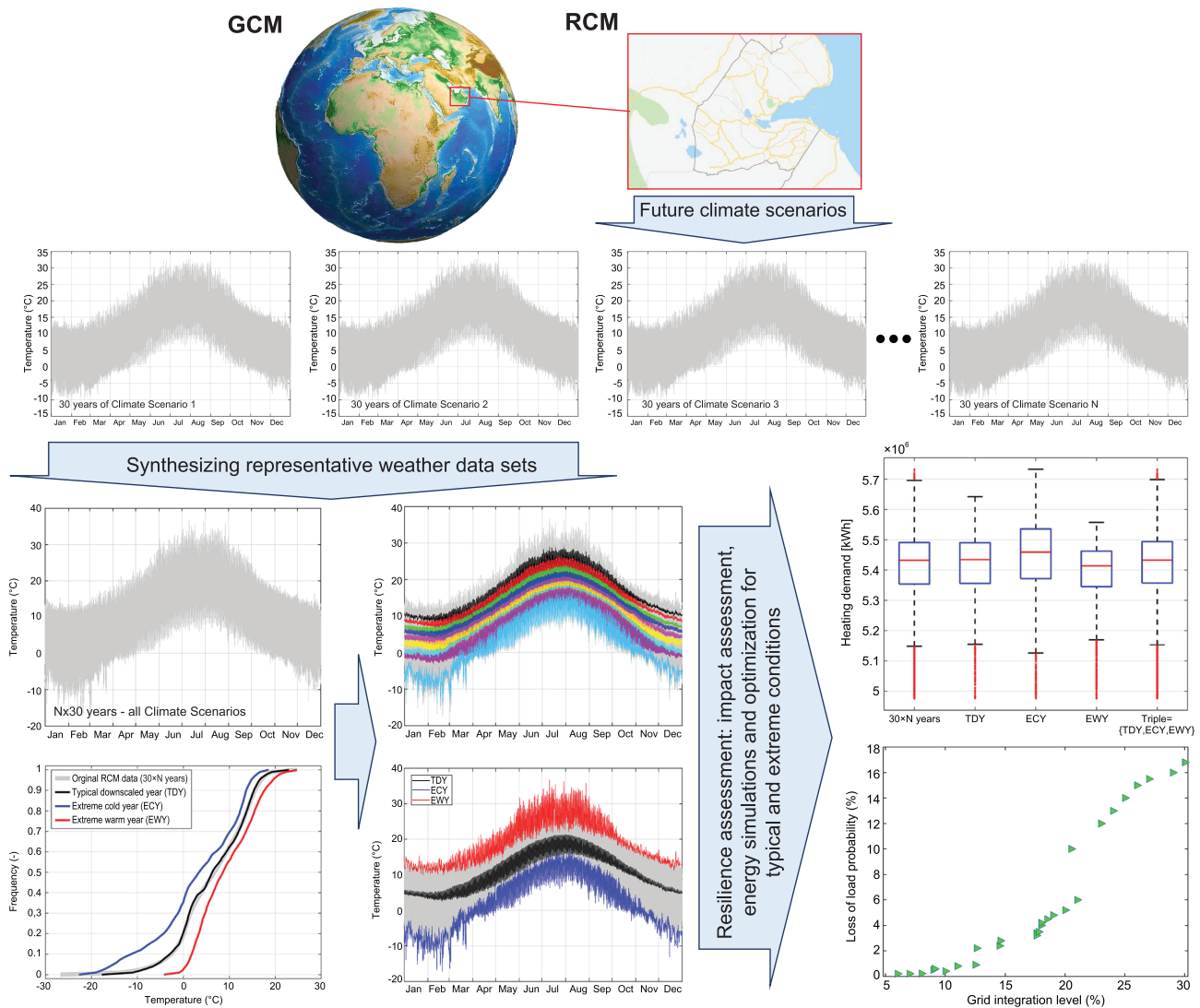
Figure 7. Assessing the climate resilience of urban energy systems demands consideration of several future climate scenarios (as well as scenarios to represent the variable conditions in urban areas). Representative weather data sets can be synthesized out of climate models to reduce the computation load without underestimating extreme conditions. For a system design, it is possible to combine several climate scenarios (to cover climate uncertainties) and synthesize typical and extreme scenarios (three weather data sets) as well as probabilistic sequences (e.g. seven data sets for the percentiles of 5–10–20–30–20–10–5%), to be used in energy simulations and to optimize urban energy systems (more details are available in Refs [9,10]).
