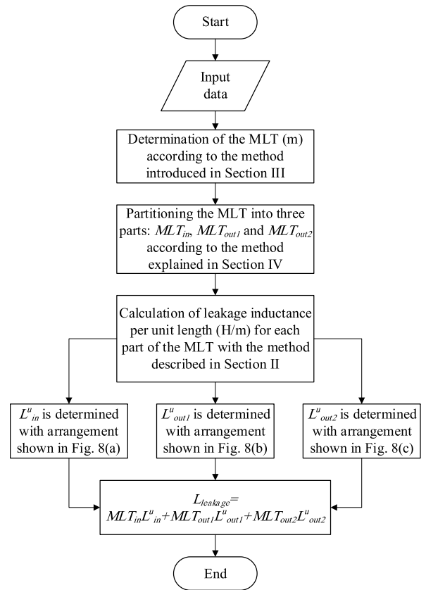
FIGURE 9. The proposed method used for calculation of the leakage inductance.
