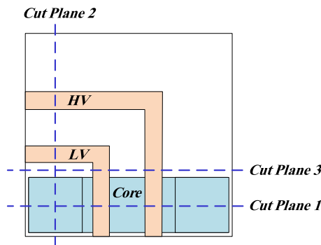
FIGURE 14. Cut planes in the corner of the model (from top view) for demonstrating the distribution of the leakage field in different regions.
