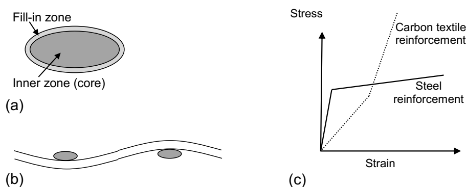
Figure 5. (a) Conceptual figure of a yarn, based on (Hartig, J., 2008). (b) Yarns running in waves above and below transverse yarns. Schematic, based on (Brameshuber, 2006). (c) Idealized stress versus strain for a carbon textile reinforcement compared to traditional steel reinforcement. From (Schladitz et al. , 2012).
