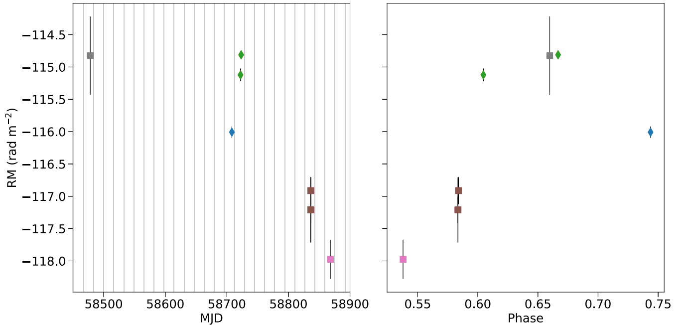
Figure 5. Measured RMs for FRB 20180916B from this work (diamonds), CHIME/FRB Collaboration et al. (2019a), and Chawla et al. (2020; squares). The RMs are corrected for the ionospheric contribution and plotted with 1\sigma error bars. Left: plot as a function of time (in MJD), where vertical lines represent phase zero of the different activity cycles of the source. Right: plot as a function of the source activity phase. The different colors of the data points represent different source cycles.
