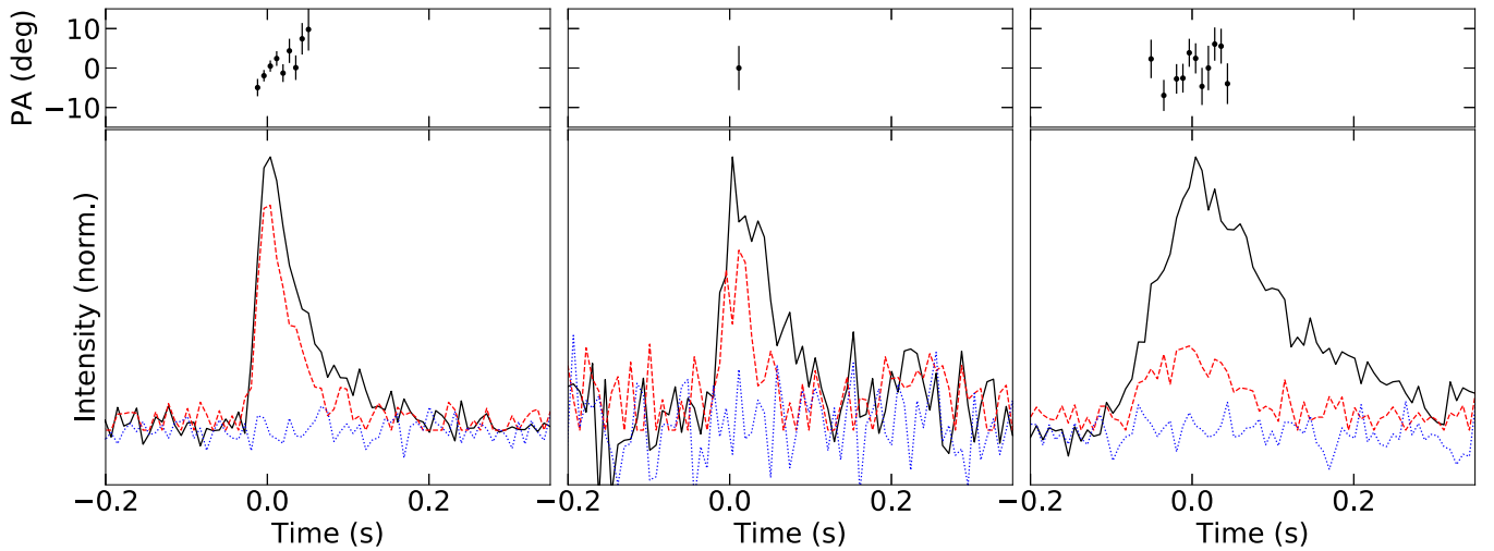
Figure 4. Polarization profiles obtained for the three LOFAR bursts with available CV data and sufficient S/N. The black curve is the total intensity, the red dashed curve is the linear polarization after correcting for Faraday rotation, and the blue dotted curve is the circular polarization. For clarity, the profiles have all been normalized to have unitary peak intensities and are plotted with a time resolution of 7.8125 ms. The PA curves are reported in the top panel of each profile and rotated by an arbitrary angle in order to be centered around zero.
