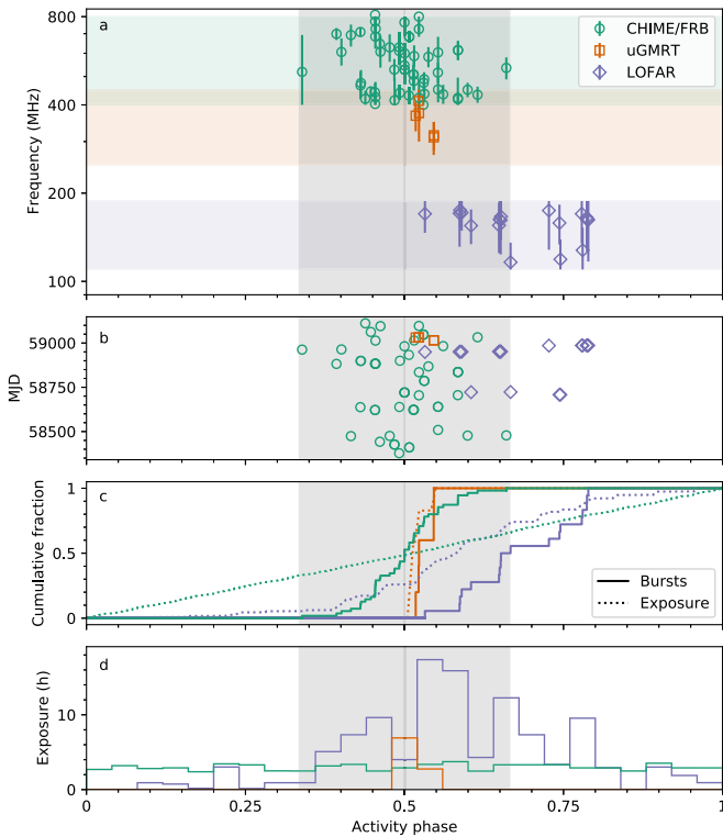
Figure 9. Activity phases of CHIME/FRB (green circles), uGMRT (orange squares), and LOFAR (purple diamonds) bursts folded on the 16.33 day activity period of FRB 20180916B. Panel (a) shows the activity phase of the bursts vs. observing frequency. For each burst, the spectral width is indicated by the error bars. Panel (b) shows the burst MJDs vs. activity phase. The cumulative fraction of the number of bursts and the exposure are shown against activity phase in panel (c), while panel (d) displays the exposure as a histogram. The color coding is identical in the three panels. Whereas the CHIME/FRB exposure is almost uniform with activity phase, the exposure of the LOFAR observations is focused predominantly on the CHIME/FRB activity window. As the number of uGMRT observations is limited, the phase of the bursts is dominated by the phase of the observations.
