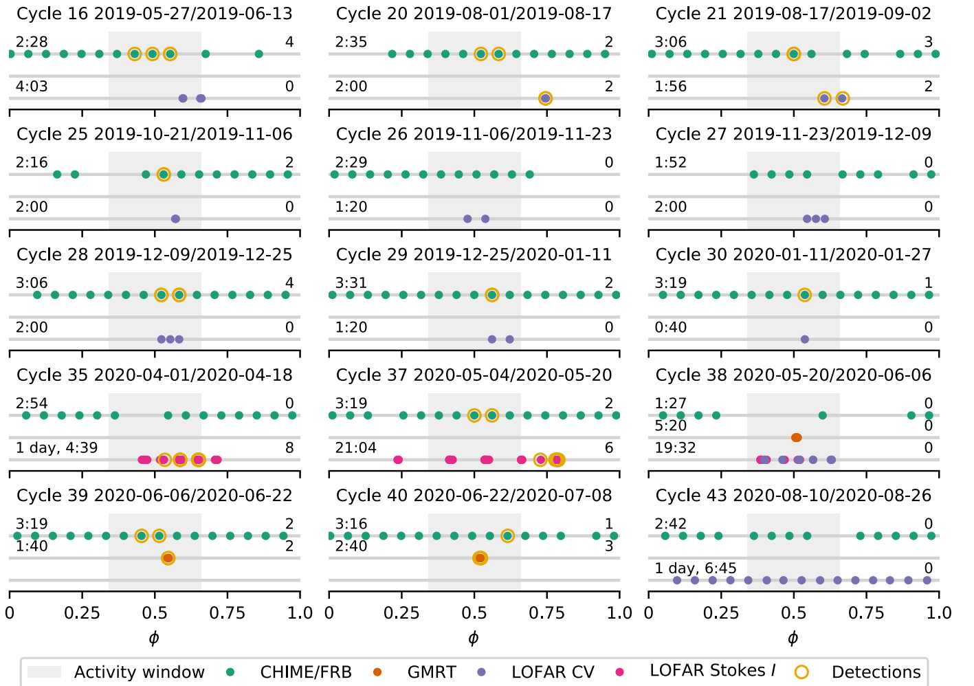
Figure 1. Summary of per-cycle observations for CHIME/FRB (top row in each panel), uGMRT (middle row in each panel), and LOFAR (bottom row in each panel), as a function of activity phase. In each row, the text on the left shows the total observing time (in hours and minutes), and the text on the right shows the total number of bursts detected in the cycle for the respective telescopes. Only cycles in which uGMRT and LOFAR were observing are shown. Note that the new CHIME/FRB detections reported here are in Cycle 32 and later and that not all of them are shown in this figure. Cycle 1 is the first cycle in which CHIME/FRB detected a burst from the source, with \phi_0 = 58,369.40 MJD, such that \phi = 0.5 is the mean of the folded phases of the CHIME/FRB bursts. Here “CV” stands for complex voltage data.
