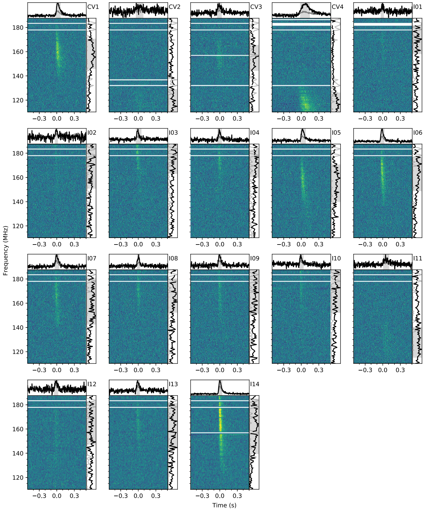
Figure 2. Dynamic spectra of bursts detected with LOFAR. All bursts are dedispersed to DM = 348.772 \text{ pc cm}^{-3} , the best-fit DM from Nimmo et al. (2021). These dynamic spectra have been averaged to a time resolution of 3.93 ms and a frequency resolution of 0.781 MHz, and the average bandpass of the off-pulse region has been subtracted. The color scale is set to be the same in all panels. The horizontal white bars indicate parts of the spectra where RFI was masked. Time-averaged spectra are shown on the right-hand side of each panel (black), as well as the fraction of averaged frequency and time points that were masked to excise RFI (light gray). The gray band in these panels denotes the burst FWHM in frequency. The top of each panel shows the frequency-averaged pulse profile over the spectral envelope of the burst (black) and the entire band (110–188 MHz; gray), with the burst FWHM denoted by the gray band. Events labeled “CVn” are from CV data, while those labeled “In” are from total intensity data.
