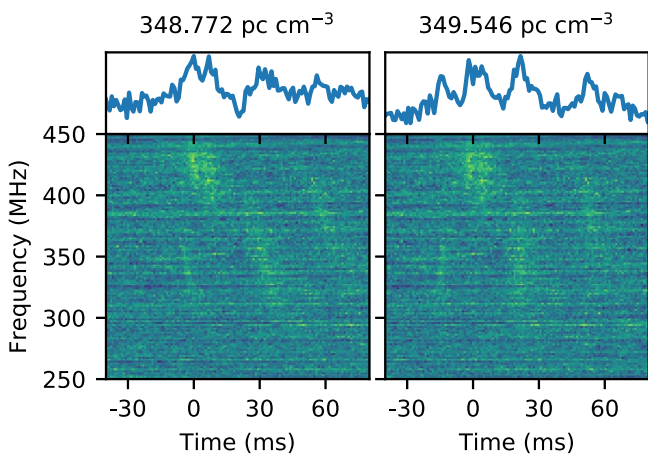
Figure 7. Burst G5 dedispersed to the best-fit DM from Nimmo et al. (2021; left) and the optimum DM from aligning the subbursts (right; see main text).
