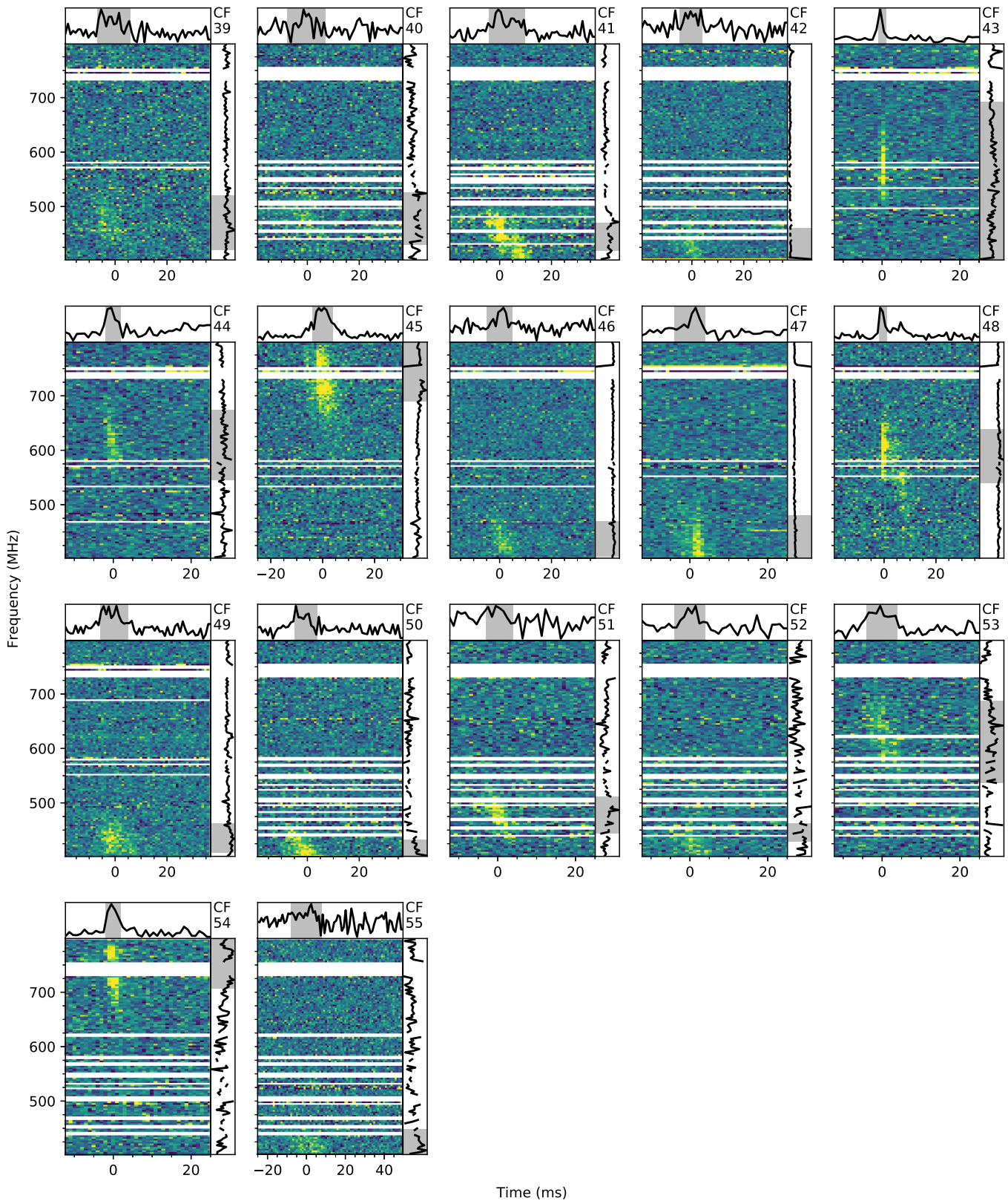
Figure 8. Dynamic spectra of bursts detected with CHIME/FRB. These dynamic spectra have a time resolution of 0.98304 ms and have been averaged to a frequency resolution of 3.125 MHz. Otherwise, the plot features are the same as in Figure 2.
