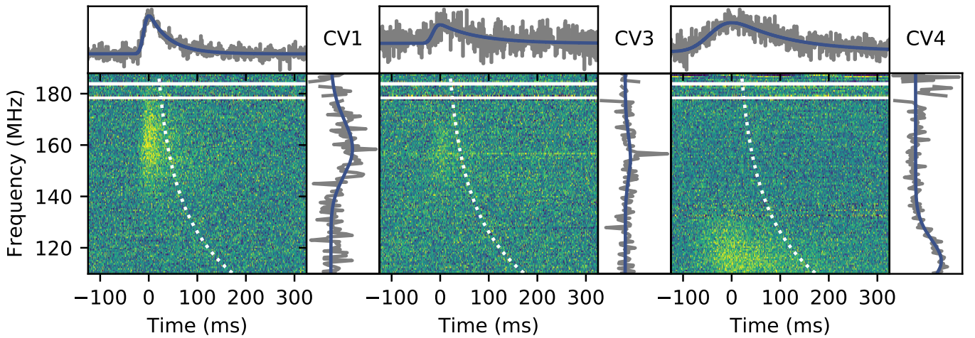
Figure 3. Least-squares burst model fits to LOFAR bursts CV1, CV3, and CV4 after coherent dedispersion. The model (solid blue line; Table 2) is overlaid on the band-averaged time series (top panels) and time-averaged spectra (right panels). A fiducial scattering timescale of 50 ms (referenced at 150 MHz) is plotted on top of the dynamic spectra (white dotted line). The horizontal white bars indicate parts of the spectra where RFI was masked.
