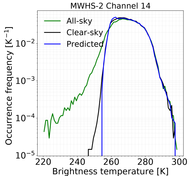
Figure 3. The distribution of point estimates (“Predicted”) obtained from QRNN-single 89 + 150 GHz for MWHS-2 channel 14. The corresponding distributions for all-sky and clear-sky simulations are also shown.
