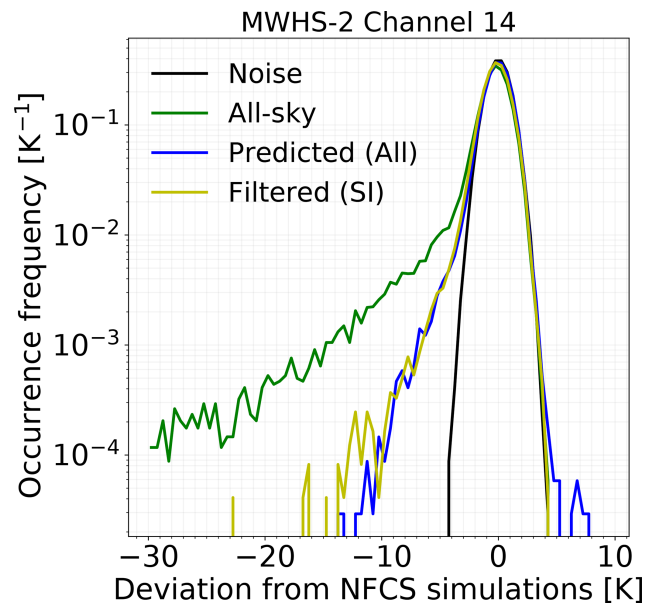
Figure 4. The error distribution for deviations of point estimates from NFCS simulations. The results are from QRNN-single experiment 89 + 150 GHz and MWHS-2 channel 14. Noise is also plotted for reference. The label “All-sky” represents the all-sky simulations; “Predicted (All)” denotes the predicted point estimates. The error distribution achieved with scattering index (SI) filtering is also shown (Filtered (SI)).
