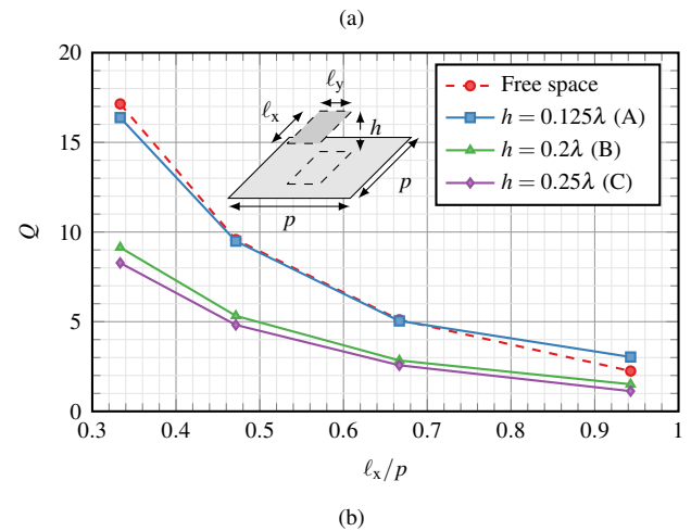
Figure 3. (a) Q-factor-predicted -10 -dB fractional bandwidth for rectangular plates of varying aspect ratios over a ground plane when \lambda = 2p and l_x l_y = p^2/9 . (b) The corresponding Q-factors as a function of l_x for heights marked in (a) with (A), (B), and (C).
