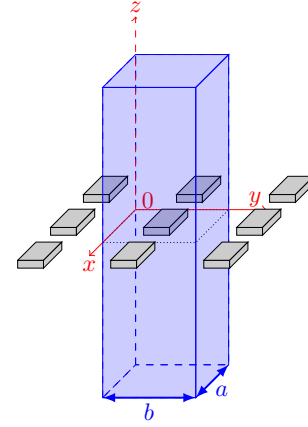
Figure 1. An example of an array geometry for current density optimization. The optimization is performed over all possible electrical current densities on the surface of an array element (cuboid in this example) within a unit cell.
