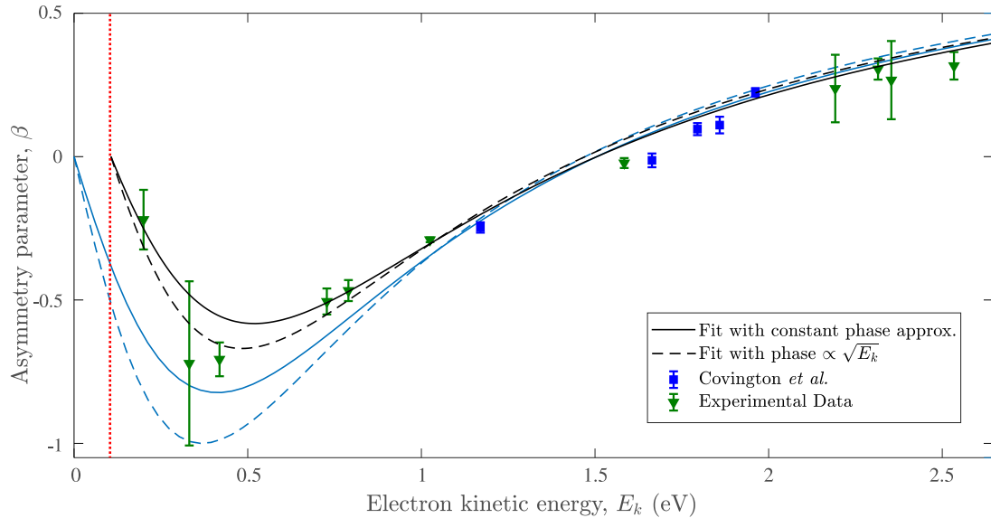
FIG. 5. Plot of the experimental asymmetry parameters as a function of the photoelectron energy. Green inverted triangles represent the measured values. The blue squares represent the previous results of Covington et al. [17]. The solid and dashed black lines are the results of fitting the measured data \beta_{\text{meas}} to Eq. (5) using a constant phase approximation and a phase proportional to \sqrt{E_k} , respectively. The dotted vertical red line marks the condition x^2 = 1 which represents the detection limit imposed by the kinematic effect. Finally, Eq. (3) is plotted in blue (gray) using the parameters extracted from the respective black fitting curves for both phase models (the solid line for the constant phase approximation and the dashed line for the model with a phase proportional to \sqrt{E_k} model). The Covington data points were not used in the fit.
