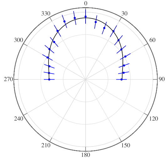
FIG. 4. Measured photoelectron yields as a function of the angle of polarization of the laser light with a photon energy of 3.06 eV. The solid line, which is a fit using Eq. (1), produces a value of the asymmetry parameter of \beta = 0.31 \pm 0.04 . This value needs to be corrected for effects associated with kinematics and the finite spread in acceptance angles. For more details, see the text.
