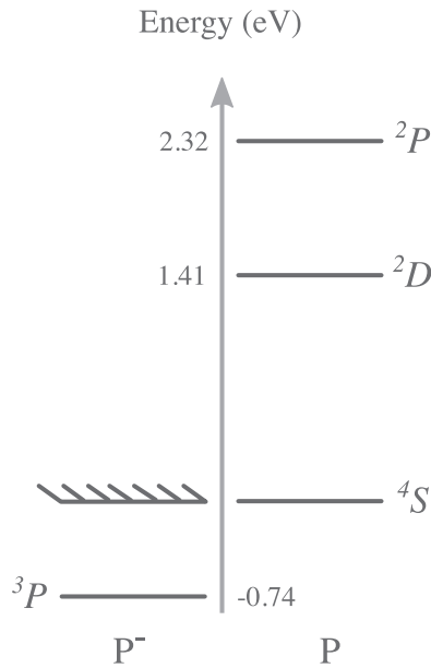
FIG. 1. Energy diagram of P^- and the lowest levels of P .
