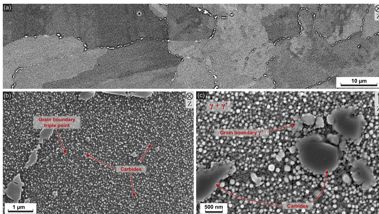
Fig. 6. Microstructure of fully heat-treated LPBF Haynes 282. (a) BSE-SEM micrograph; (b) SE-SEM micrograph showing grain boundary triple point; (c) SE-SEM micrograph showing grain boundary phases.
