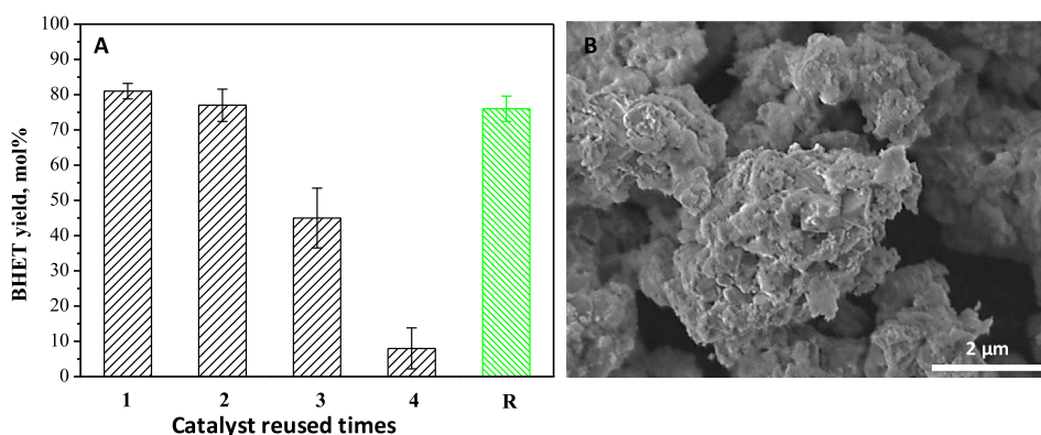
Fig. 6. The catalytic efficiency of the Mg-Al-O@Fe 3 O 4 micro particles in the glycolysis of PET when the catalyst was reused up to 4 times and R represents the regenerated catalyst. B is the SEM image of deactivated Mg-Al-O@Fe 3 O 4 micro catalyst after reusing for 4 times.
