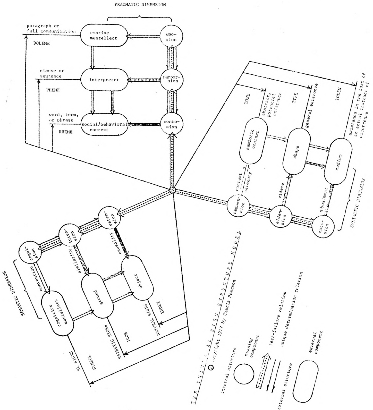
Fig. 1. The Universal Sign Structure Model
