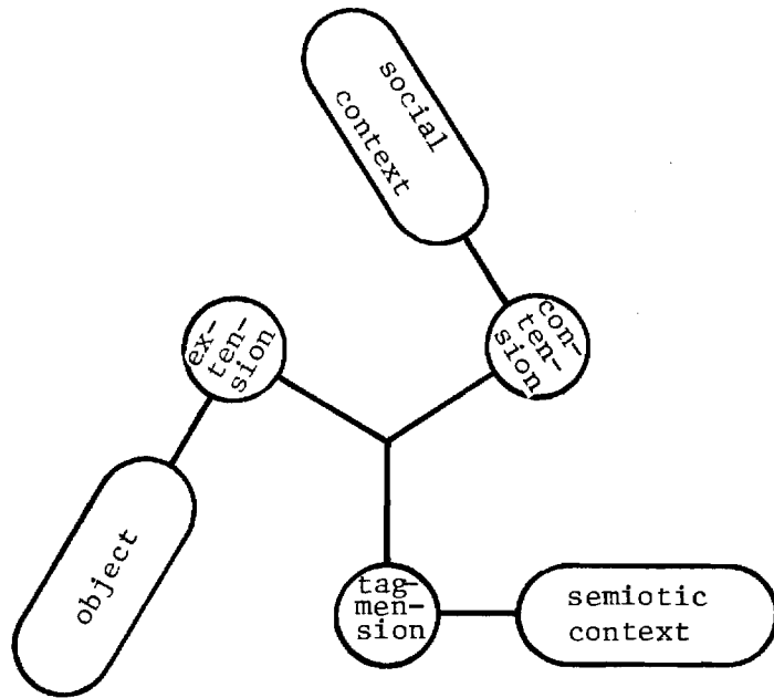
Fig. 2. The Minimum Semiotic Structure
