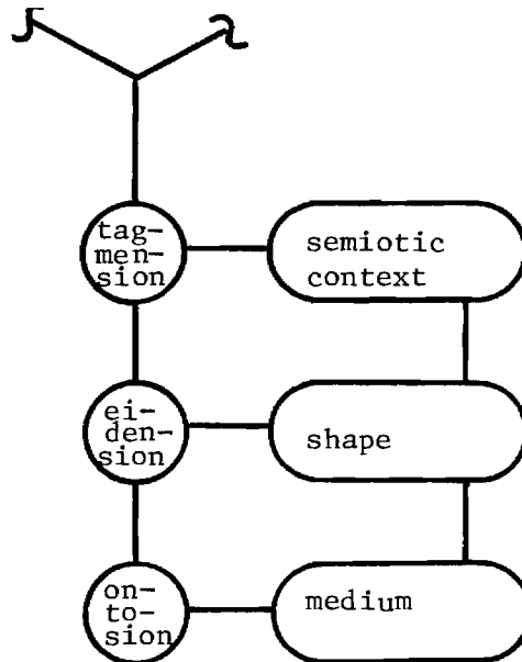
Fig. 13. Structure of Communication
