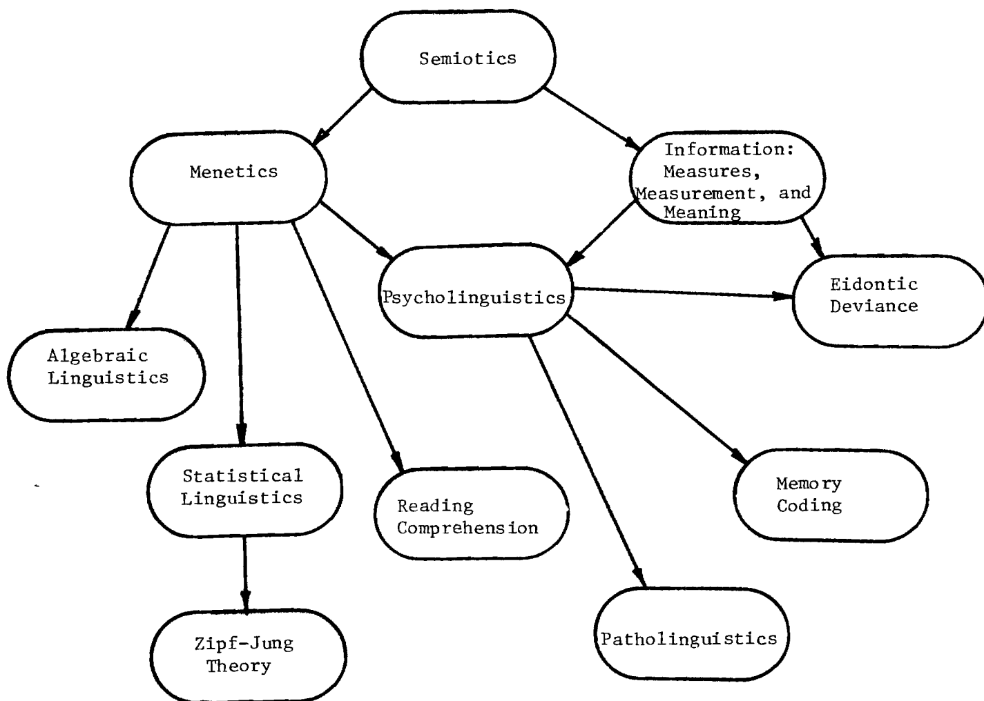
Fig. 19 Bibliographic Subset Lattice for Semiotics
