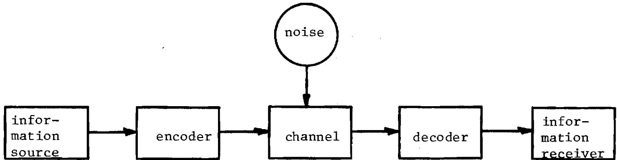
Fig. 16. The Communication Model
