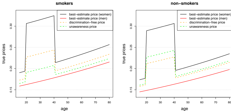
FIGURE 3. True model: (left) smokers and (right) non-smokers with solid black and red lines giving the best-estimate prices for women and men, respectively. The dotted orange lines show the discrimination-free prices and the dotted green lines show the unawareness prices, for an alternative assumption on \mathbb{P}(D = \text{woman} \mid \text{smoker}) .
