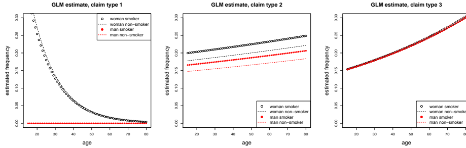
FIGURE 8. GLM estimated regression functions \hat{\lambda}_1^{\text{GLM}}(\mathbf{X}, D) (left), \hat{\lambda}_2^{\text{GLM}}(\mathbf{X}, D) (middle) and \hat{\lambda}_3^{\text{GLM}}(\mathbf{X}, D) (right).
