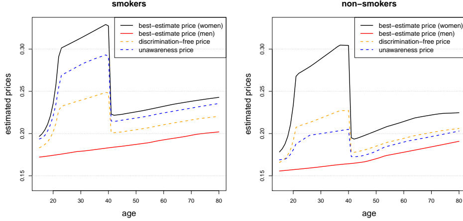
FIGURE 6. Estimated neural network model: (left) smokers and (right) non-smokers with solid black and red lines giving the best-estimate prices for women and men, respectively. The dotted orange lines show the discrimination-free prices and the dotted blue lines show the unawareness prices.
