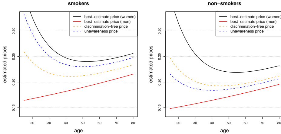
FIGURE 9. Estimated GLM: (left) smokers and (right) non-smokers with solid black and red lines giving the best-estimate prices for women and men, respectively. The dotted orange lines show the discrimination-free prices and the dotted blue lines show the unawareness prices.
