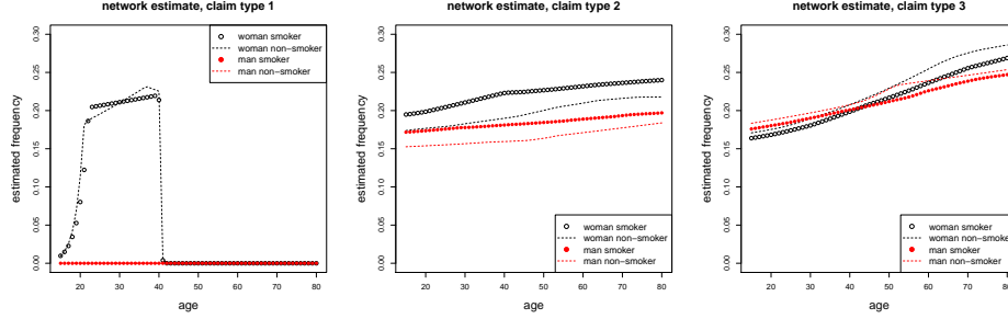
FIGURE 5. Estimated regression functions \hat{\lambda}_1(\mathbf{X}, D) (left), \hat{\lambda}_2(\mathbf{X}, D) (middle) and \hat{\lambda}_3(\mathbf{X}, D) (right) using the neural network architecture of Listing 2.
