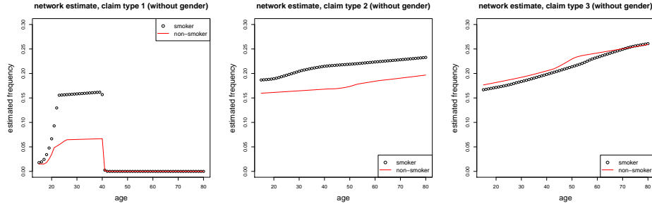
FIGURE 7. Estimated regression functions \hat{\lambda}_1(\mathbf{X}) (left), \hat{\lambda}_2(\mathbf{X}) (middle) and \hat{\lambda}_3(\mathbf{X}) (right) using neural networks and ignoring the gender information D .
