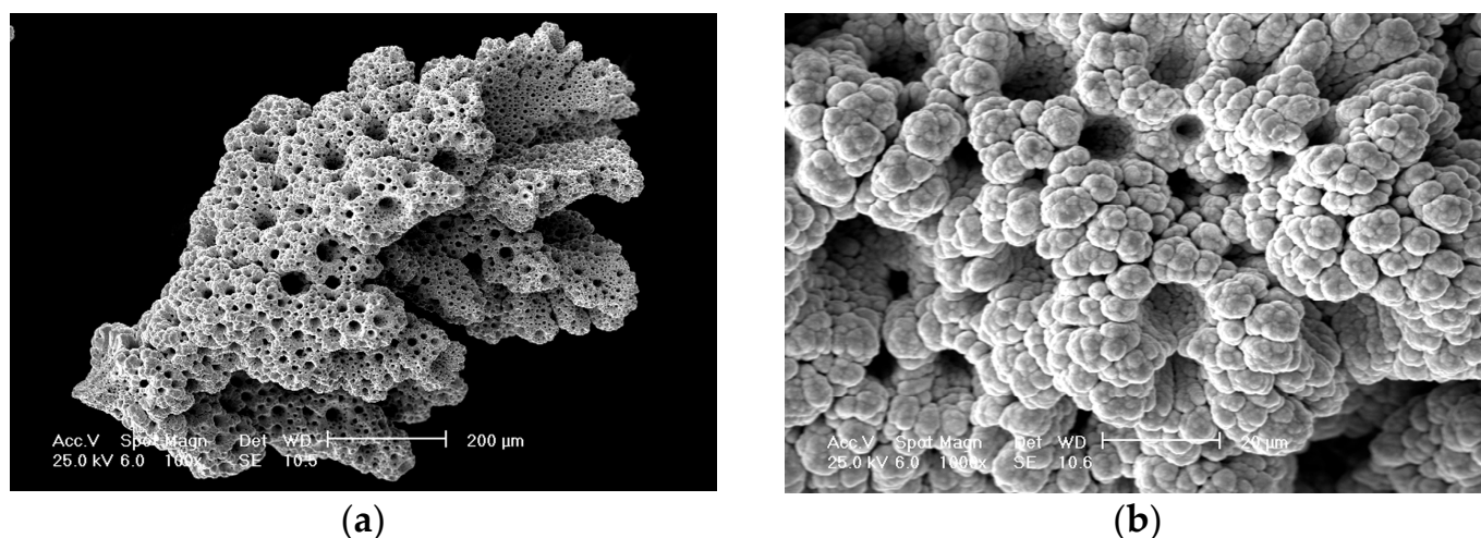
Figure 12. (a) Morphology of the spongy-like particle obtained by Ni electrodeposition from 1 \text{ M NH}_4\text{Cl} + 0.7 \text{ M NH}_4\text{OH} + 0.1 \text{ M NiCl}_2 at j of 1265 \text{ mA cm}^{-2} , and (b) detail of the particle shown under (a) [20].
