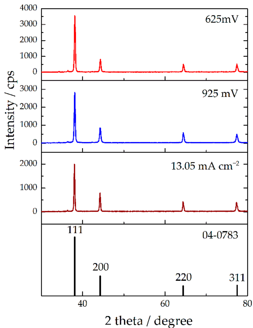
Figure 9. The XRD patterns of Ag particles obtained from the ammonium electrolyte at overpotentials of 625 and 925 mV and at a current density of 13.05 \text{ mA cm}^{-2} and Ag standard (04-0783) ([18] and reprinted from [34] with permission from Elsevier).
