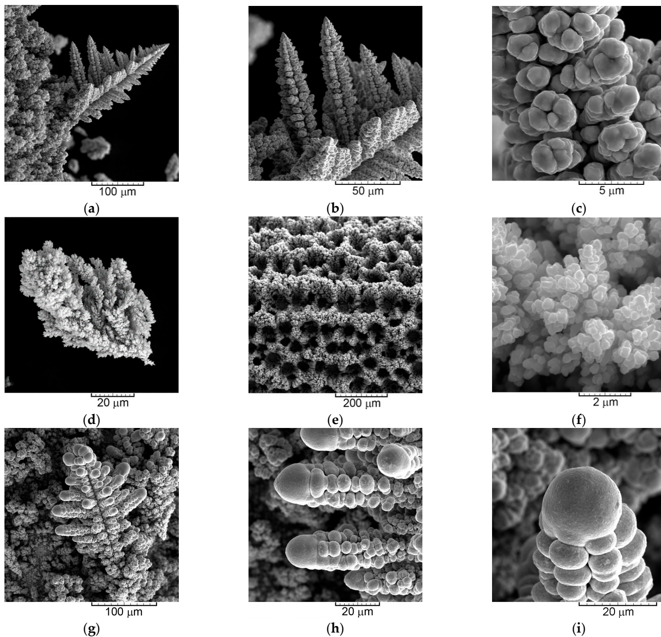
Figure 10. The powder particles produced by Cu electrodeposition from 0.10 M \text{CuSO}_4 in 0.50 M \text{H}_2\text{SO}_4 at \eta of (a–c) 625 mV and (d–f) 925 mV and at j of (g–i) 14.4 \text{ mA cm}^{-2} ([19] and reprinted from [38] with permission from Elsevier).
