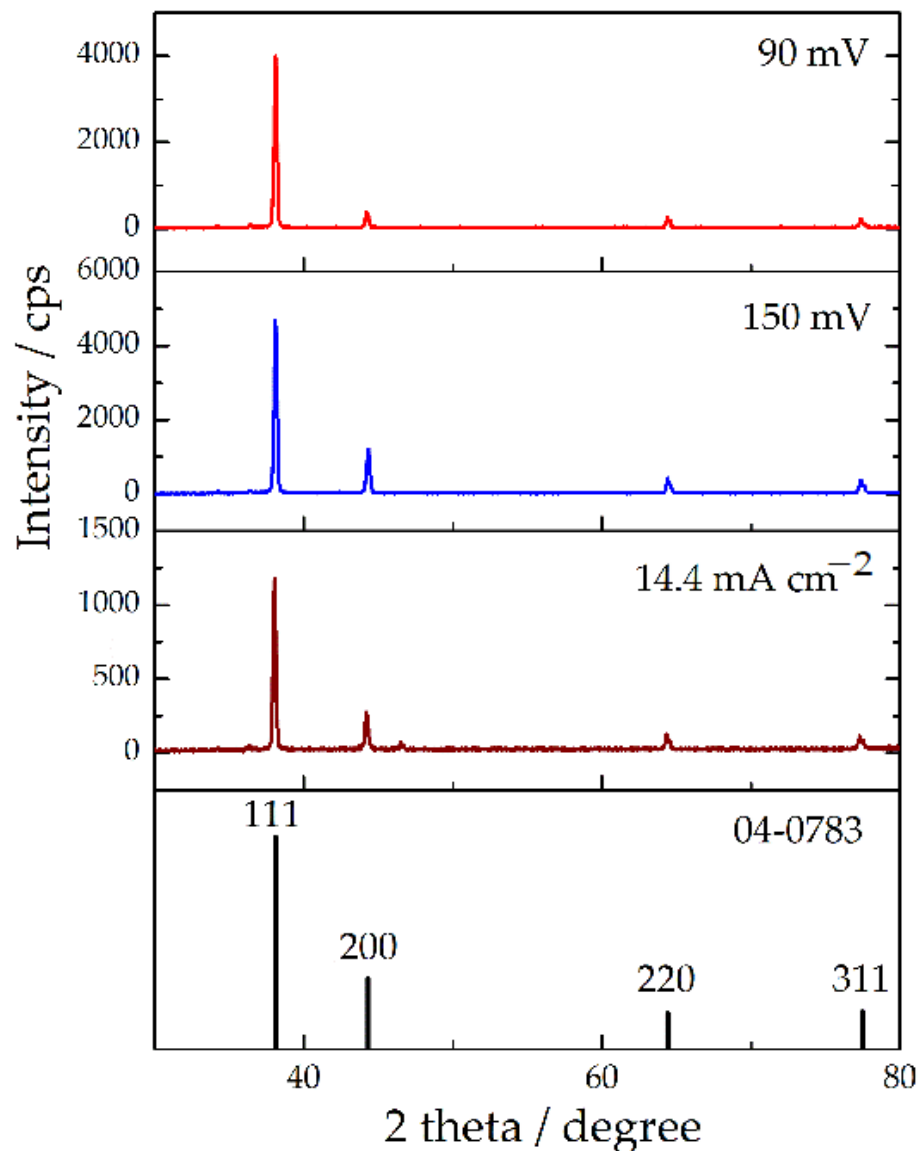
Figure 6. The XRD patterns of Ag particles obtained from the nitrate electrolyte at \eta of 90 and 150 mV and at j of 14.4 \text{ mA cm}^{-2} and Ag standard (04-0783) ([18] and reprinted from [34] with permission from Elsevier).
