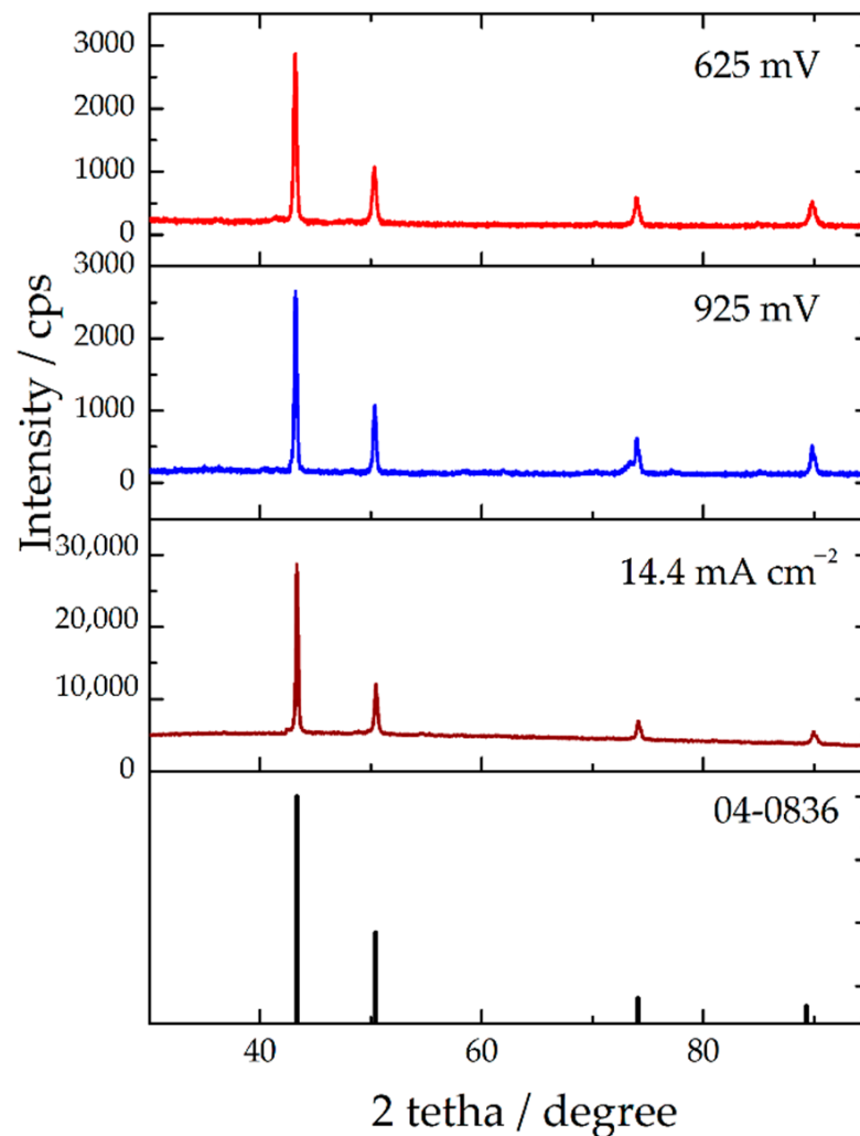
Figure 11. The XRD patterns of Cu particles obtained from the sulfate electrolyte at overpotentials of 625 and 925 mV and at a current density of 14.4 \text{ mA cm}^{-2} and Cu standard (04-0836) ([19] and reprinted from [38] with permission from Elsevier).
