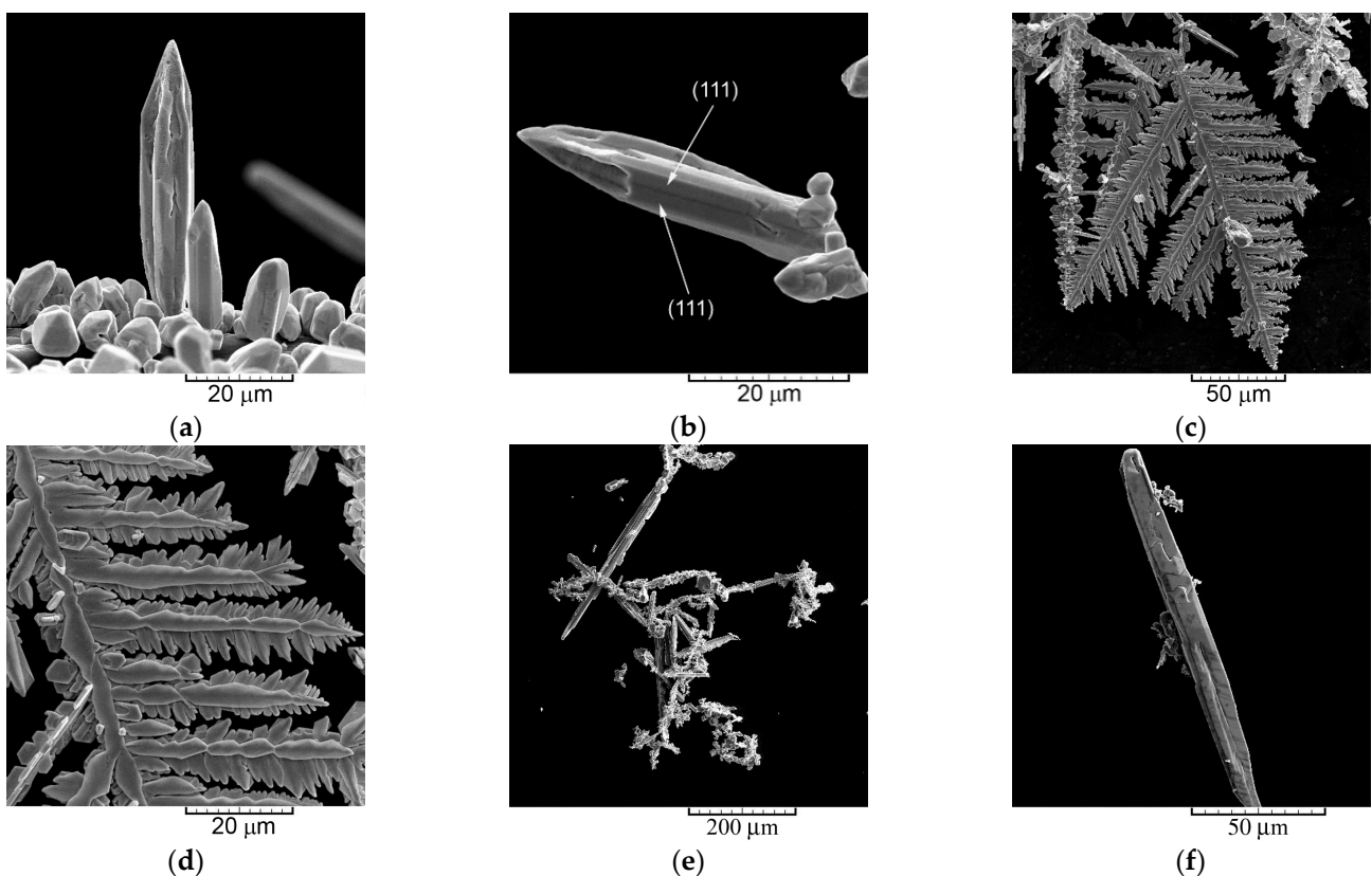
Figure 5. Morphologies of Ag powder particles produced by electrodeposition from the nitrate electrolyte (0.10 M AgNO 3 in 2.0 M NaNO 3 ) at overpotentials of (a,b) \eta = 90 mV and (c,d) \eta = 150 mV and at a current density of (e,f) j = 14.4 mA cm -2 ([18] and reprinted from [34] with permission from Elsevier).
