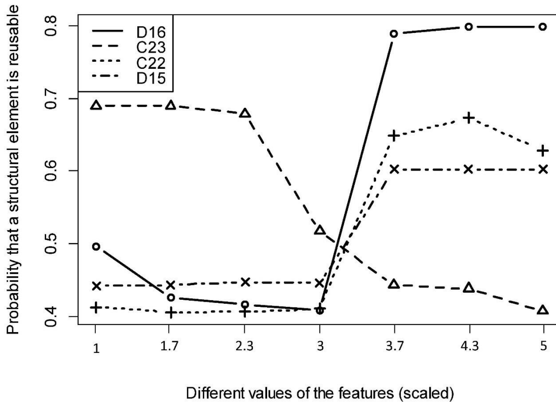
Figure 6.14 The impact of different values the features on the reusability probabilities of the elements (sensitivity analysis) for D16, C23, C22, and D15 (the top-four variables in SOC-RF BSE-RPM)
