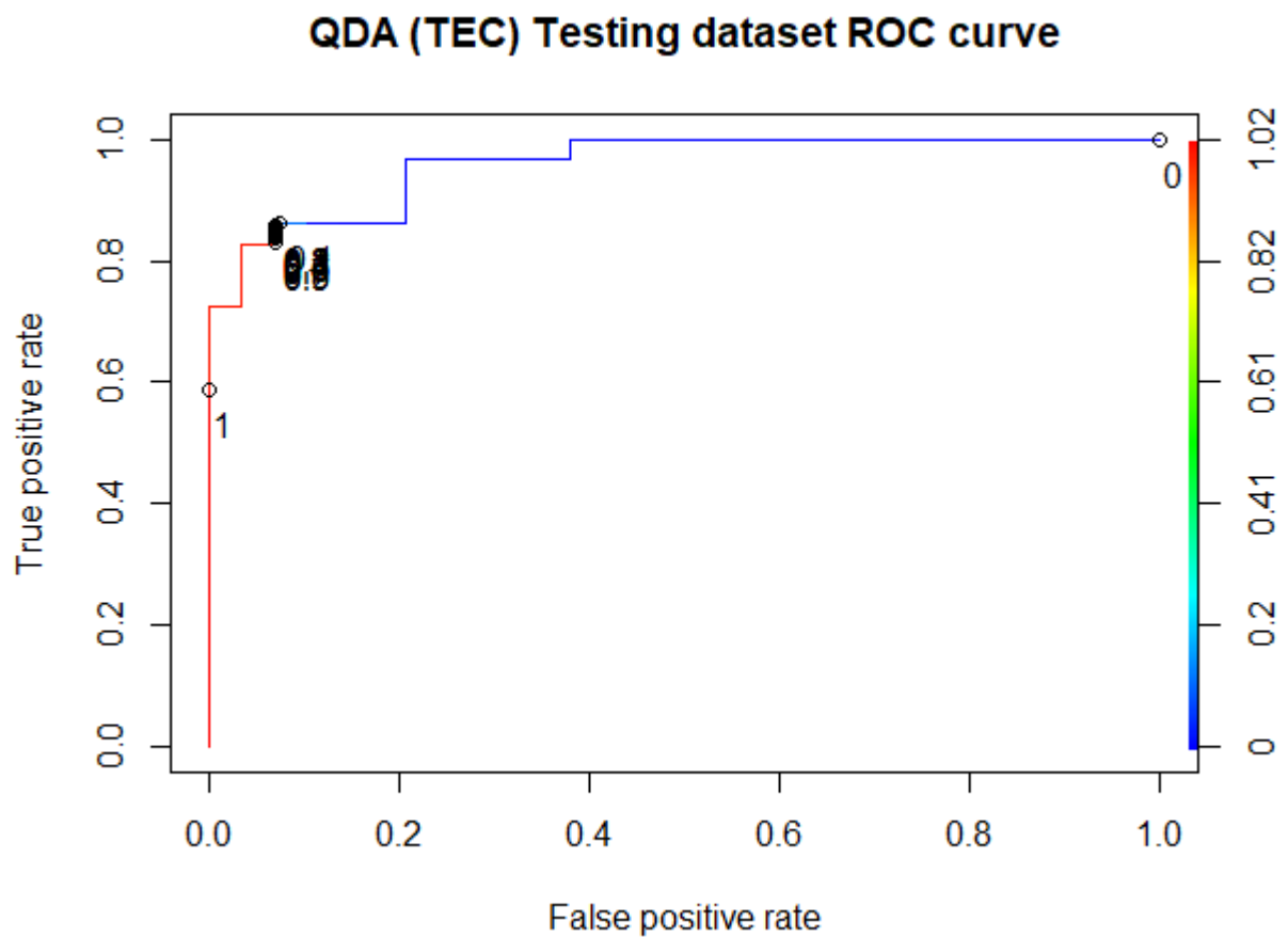
Figure F-4 The ROC curve of the QDA BSE-RPM (TEC dataset)
