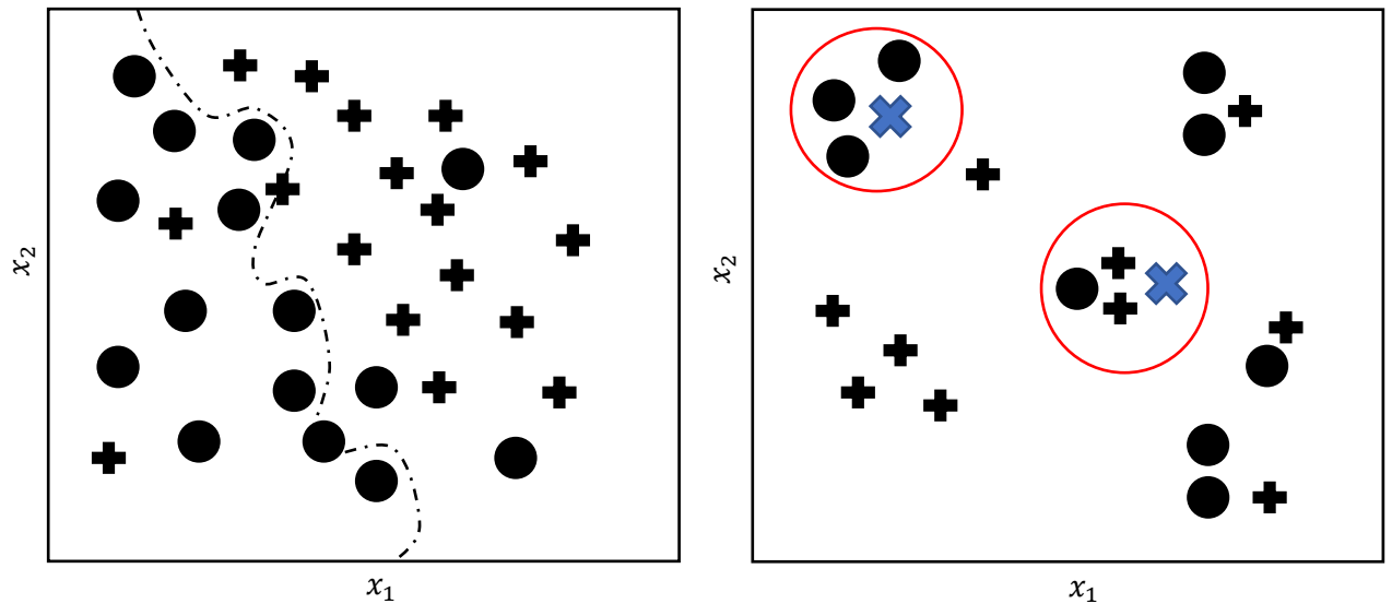
Figure 5.8 The Bayes classifier (left) and K-Nearest Neighbours (KNN) classifier (right)
