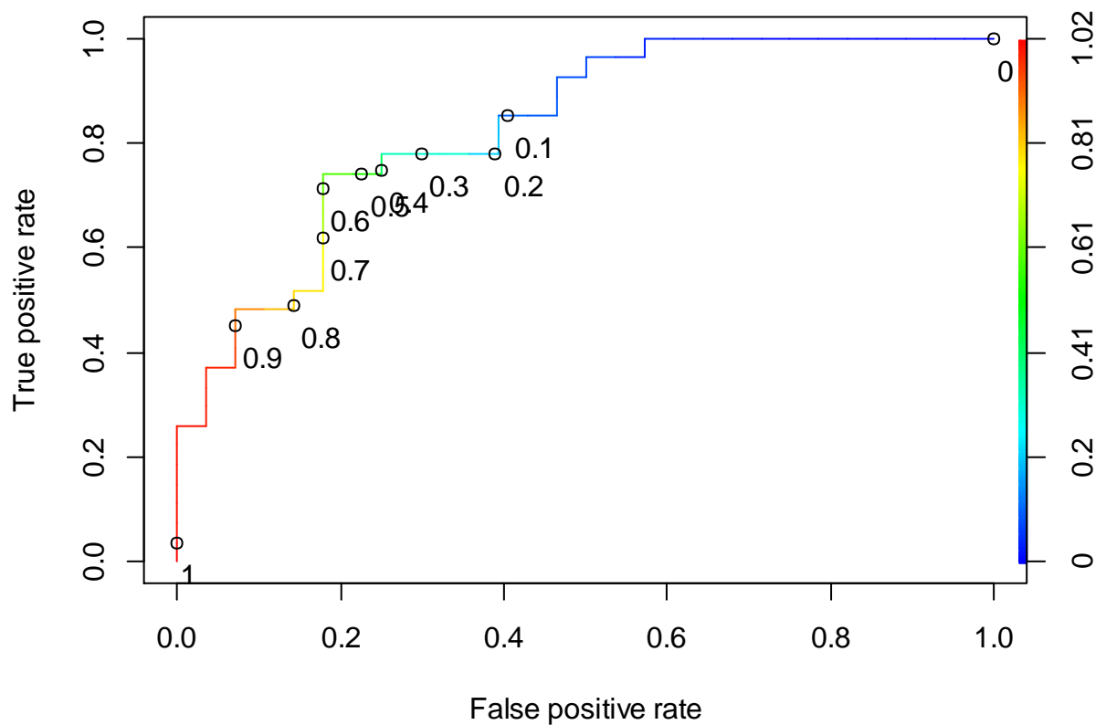
Figure F-18 The ROC curve of the QDA BSE-RPM (ECO dataset)
