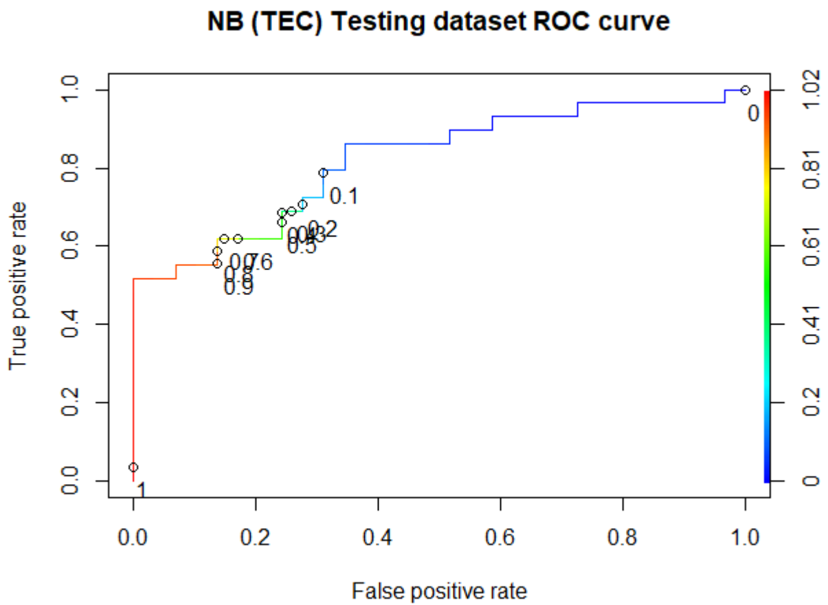
Figure F-5 The ROC curve of the NB BSE-RPM (TEC dataset)
