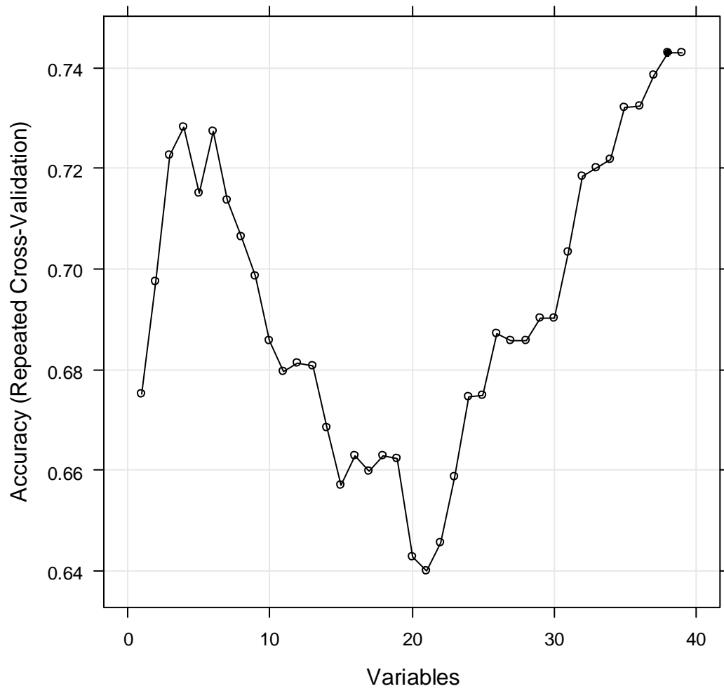
Figure 5.5 Performance of the RFE and Naïve Bayes based on the ranks of the features (TEC dataset)
