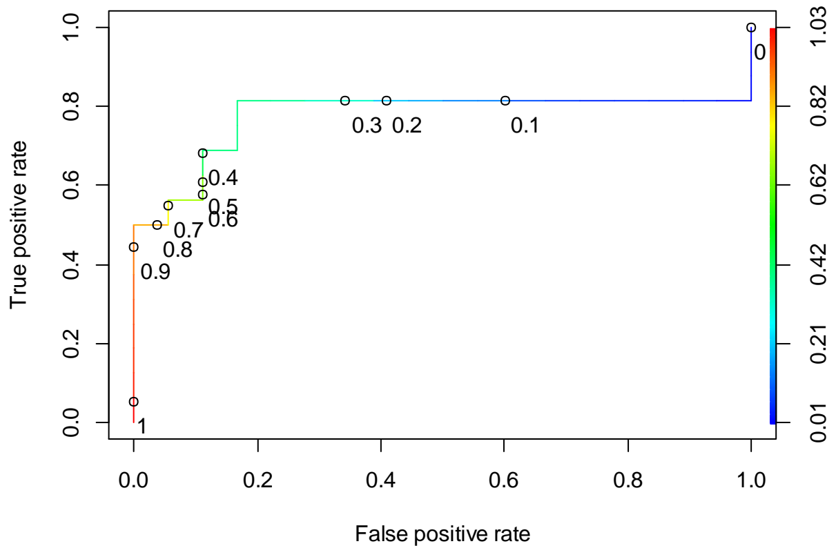
Figure F-31 The ROC curve of the LDA BSE-RPM (SOC dataset)
