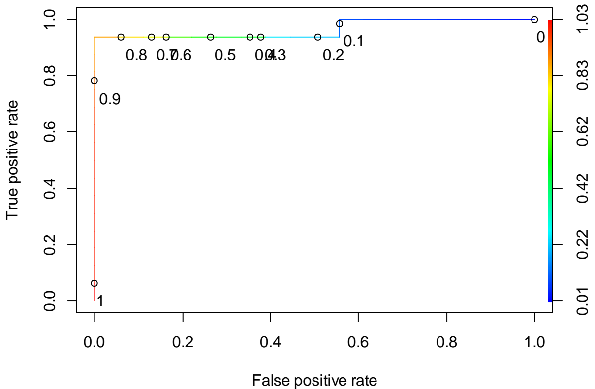
Figure F-33 The ROC curve of the NB BSE-RPM (SOC dataset)
