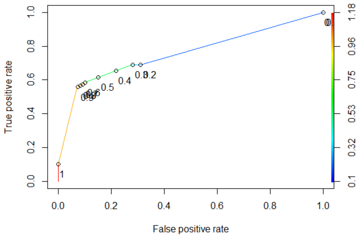
Figure F-6 The ROC curve of the DT BSE-RPM (TEC dataset)
