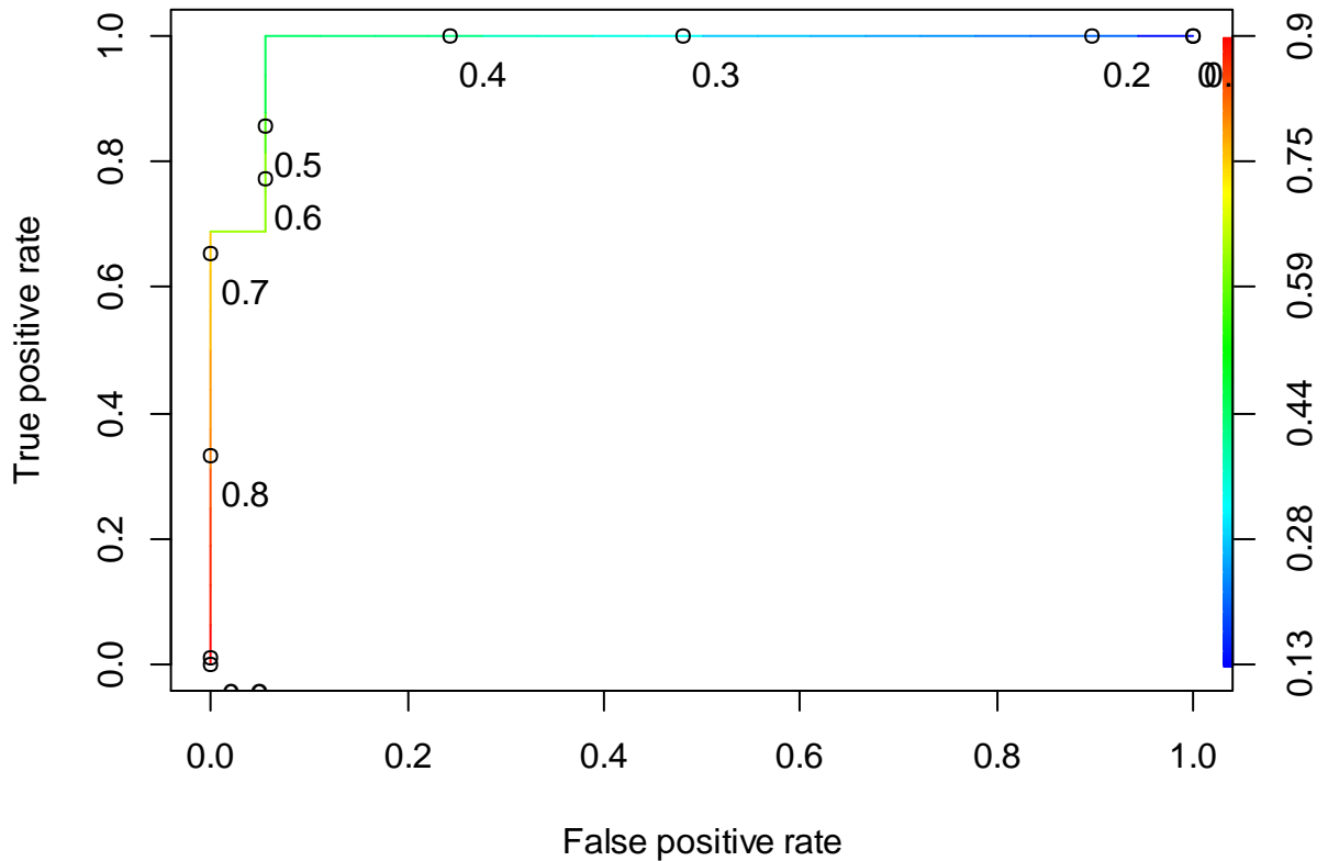
Figure F-38 The ROC curve of the BM BSE-RPM (SOC dataset)
