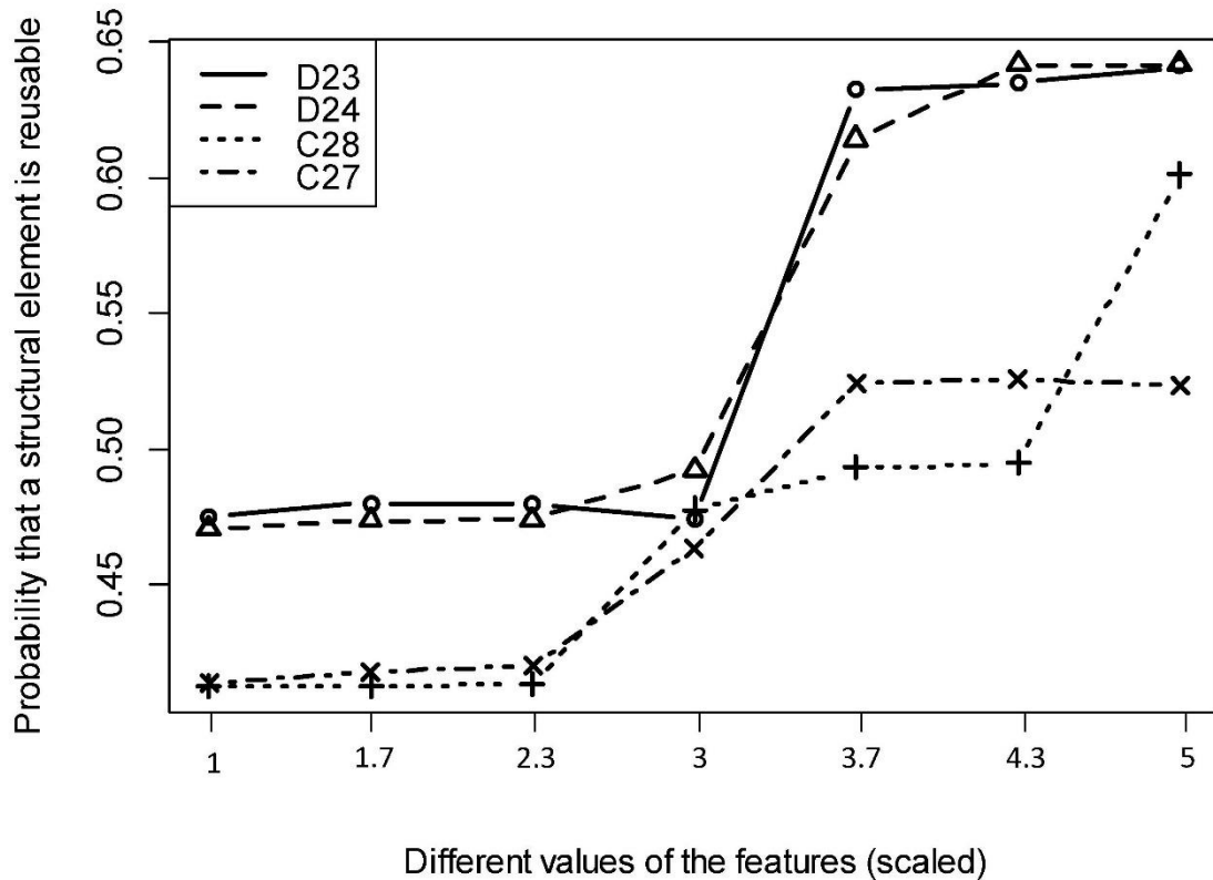
Figure 6.3 The impact of different values the features on the reusability probabilities of the elements (sensitivity analysis) for D23, D24, C28, and C27 (the top-four variables in TEC-RF BSE-RPM)
