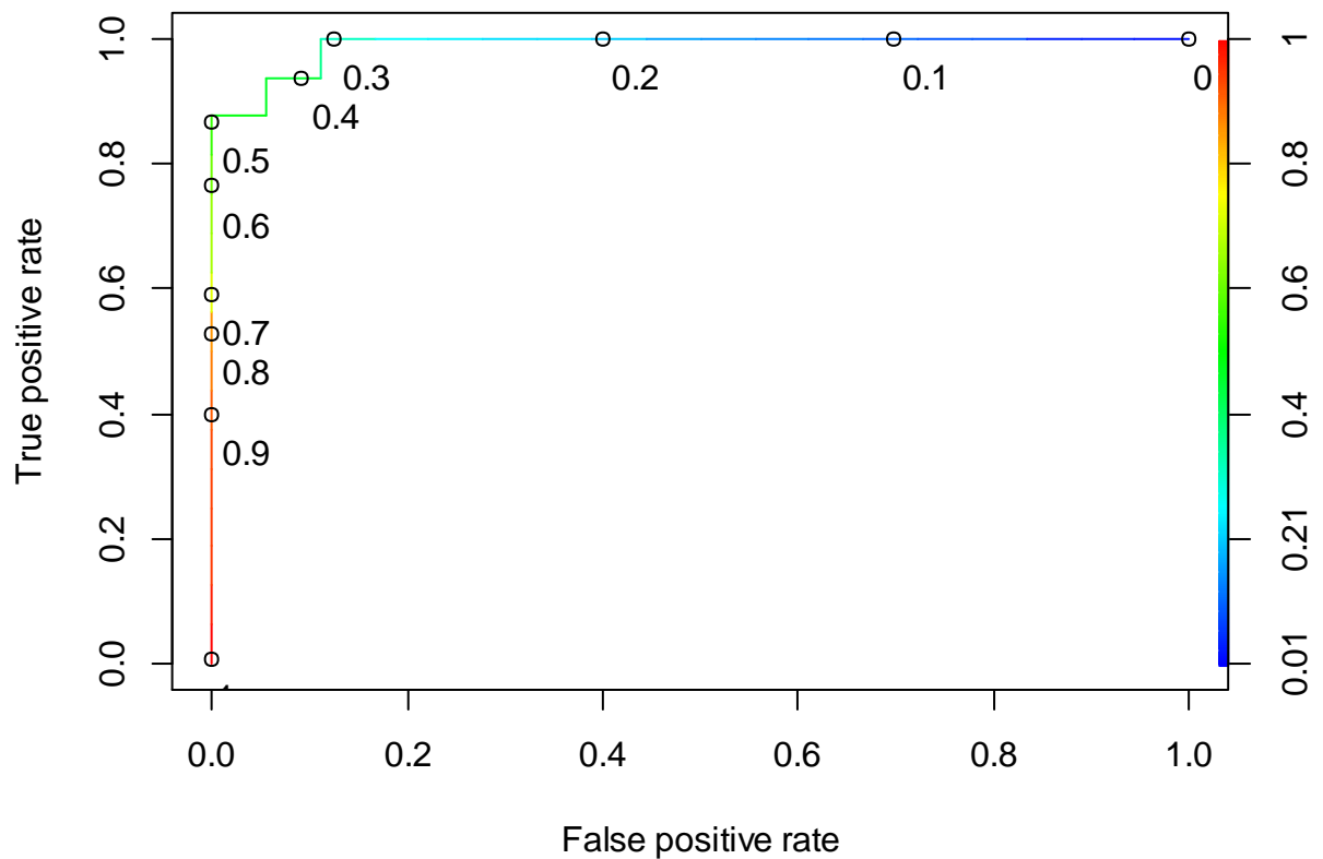
Figure F-36 The ROC curve of the RF BSE-RPM (SOC dataset)
