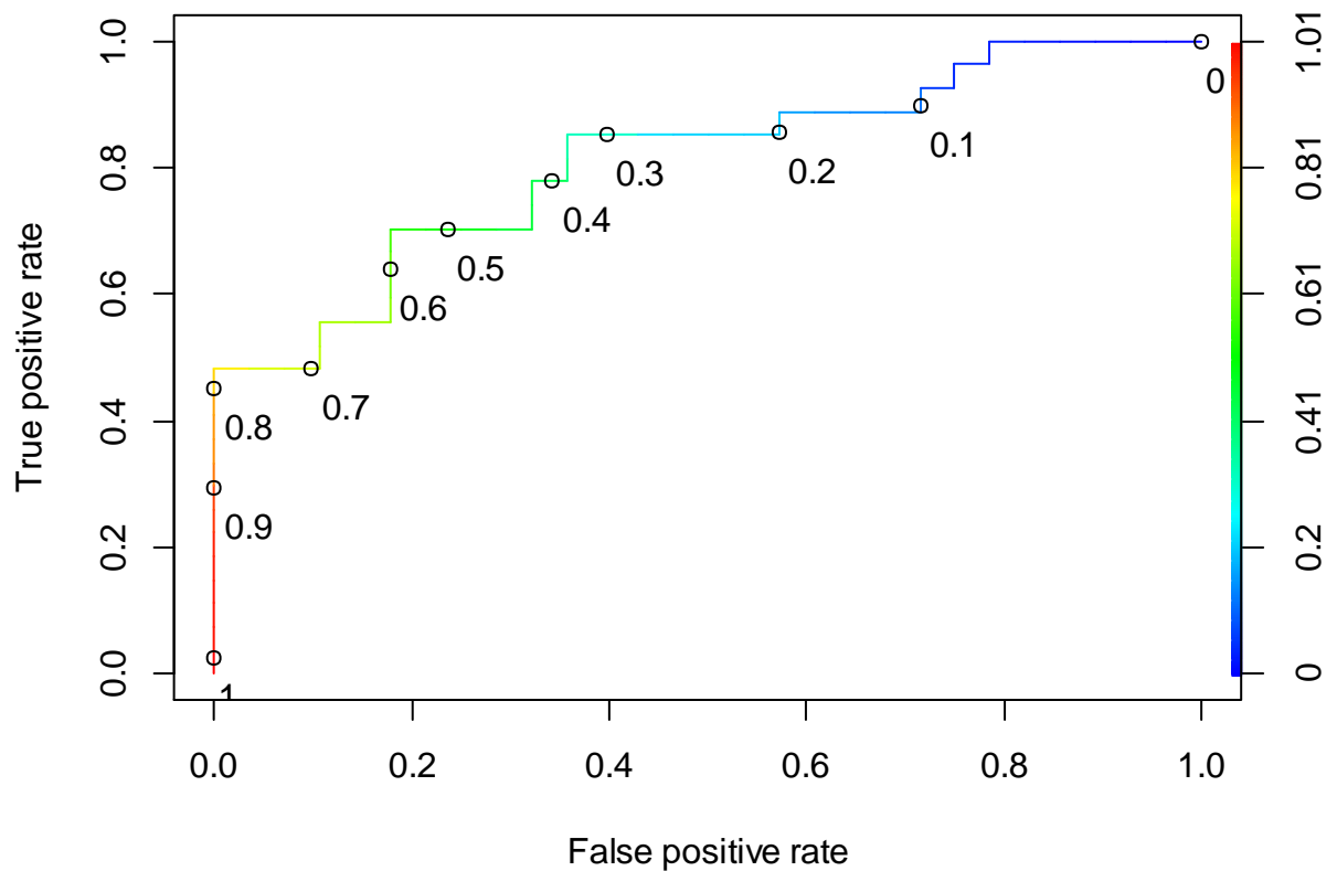
Figure F-16 The ROC curve of the LR BSE-RPM (ECO dataset)
