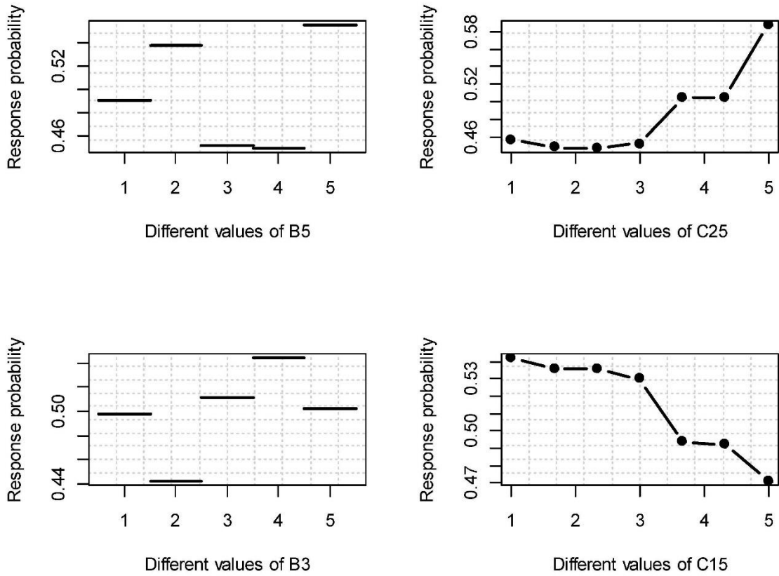
Figure 6.4 The impact of different values the features on the reusability probabilities of the elements (sensitivity analysis) for B5, C25, B3, and C15 (TEC-RF BSE-RPM)
