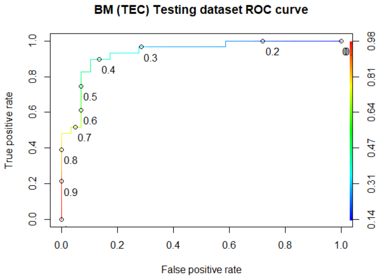
Figure F-10 The ROC curve of the BM BSE-RPM (TEC dataset)
