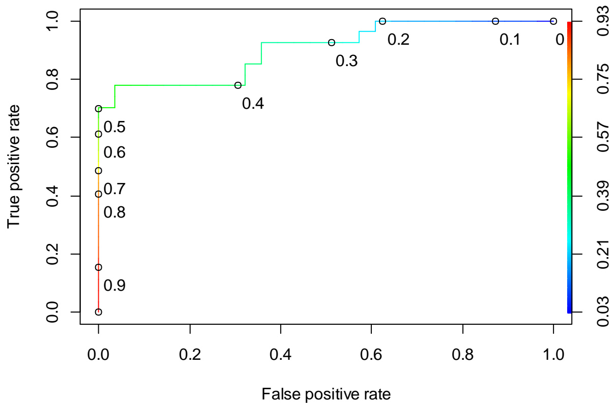
Figure F-24 The ROC curve of the BM BSE-RPM (ECO dataset)
