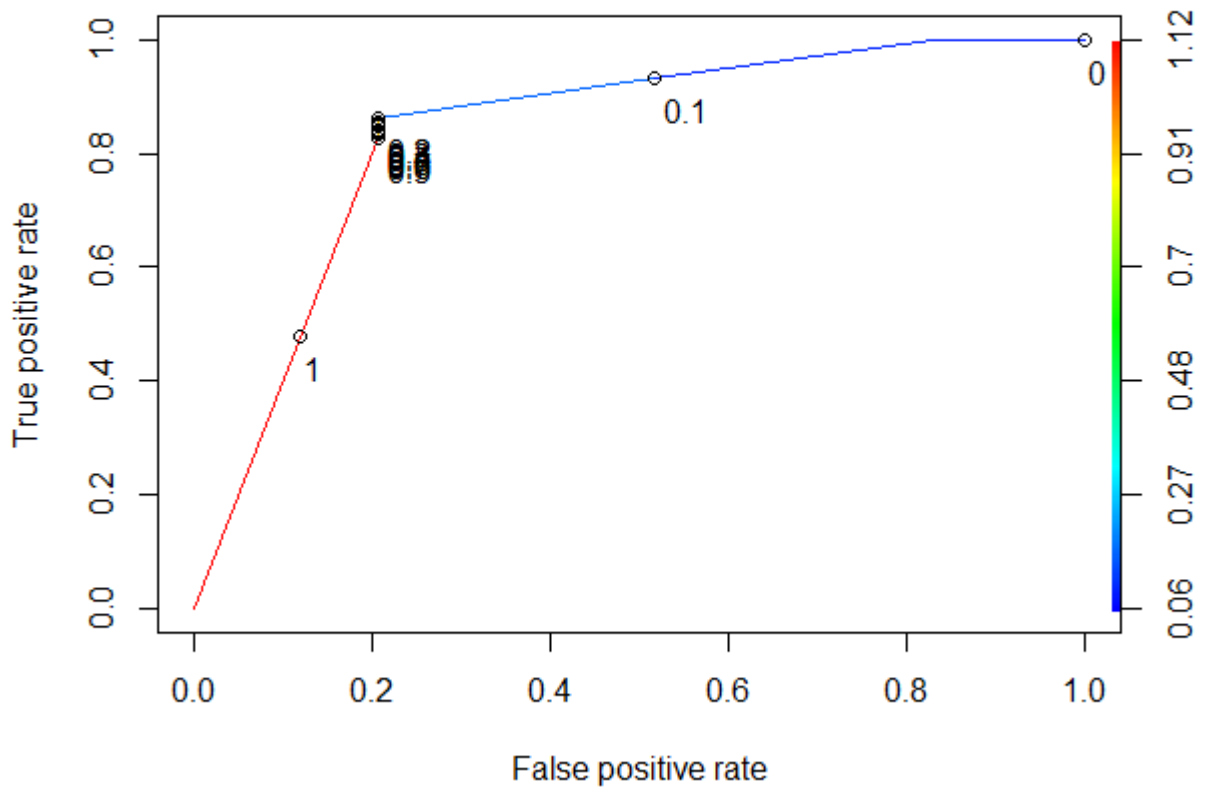
Figure F-13 The ROC curve of the PRL BSE-RPM (TEC dataset)
