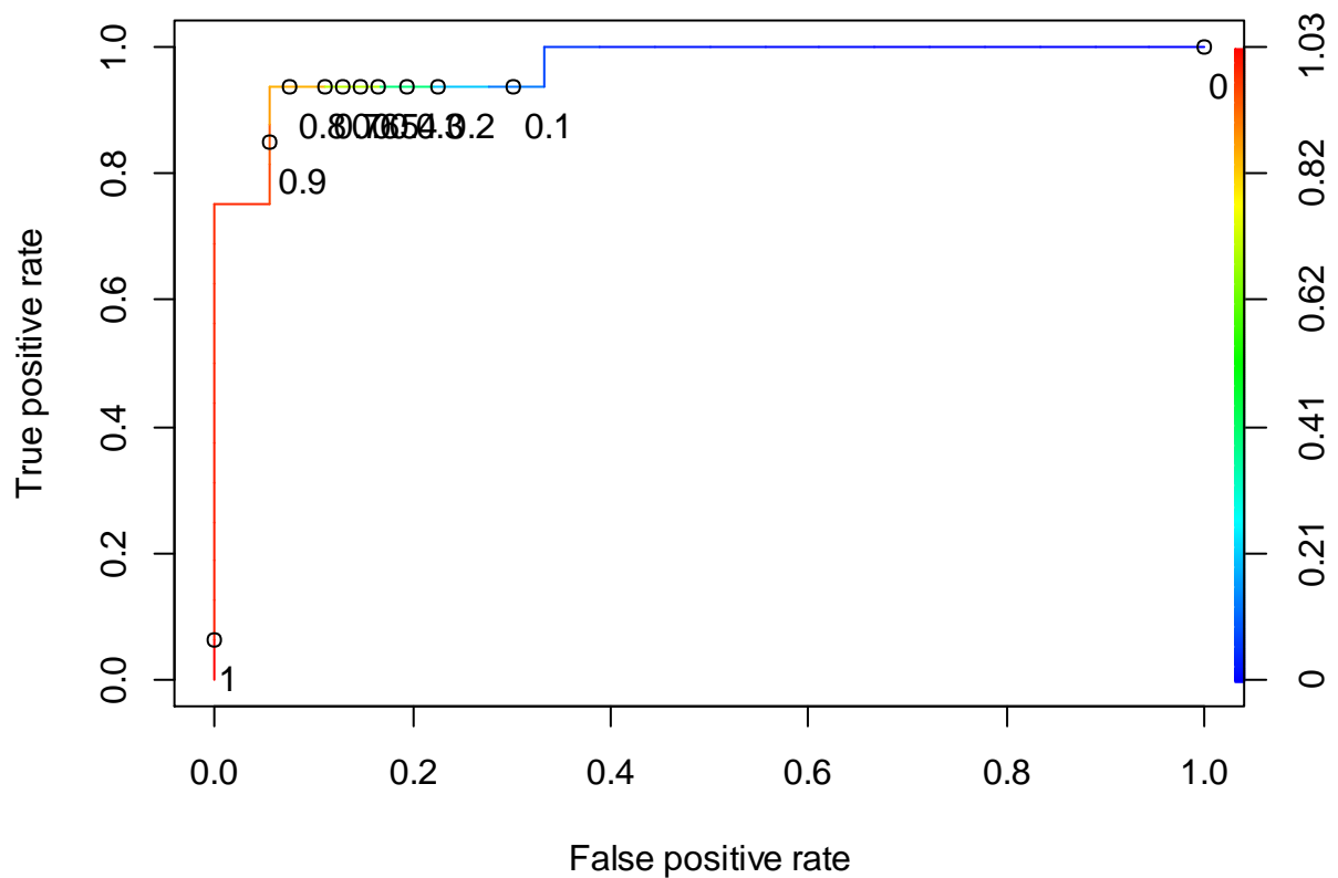
Figure F-32 The ROC curve of the QDA BSE-RPM (SOC dataset)
