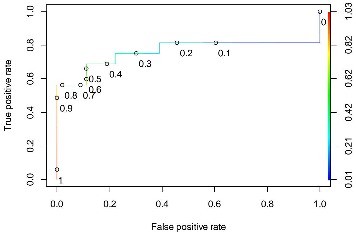
Figure F-30 The ROC curve of the LR BSE-RPM (SOC dataset)
