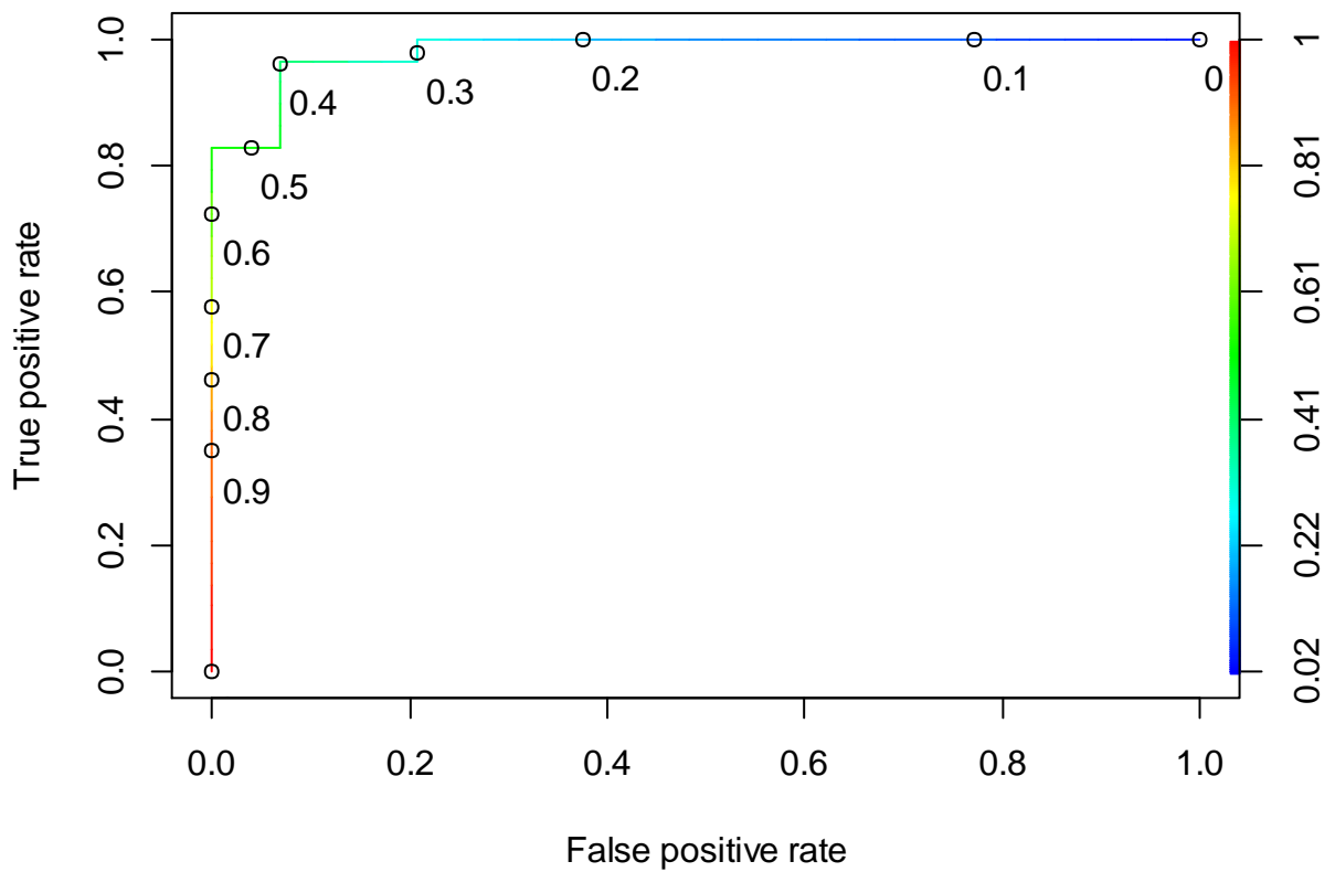
Figure F-8 The ROC curve of the RF BSE-RPM (TEC dataset)
