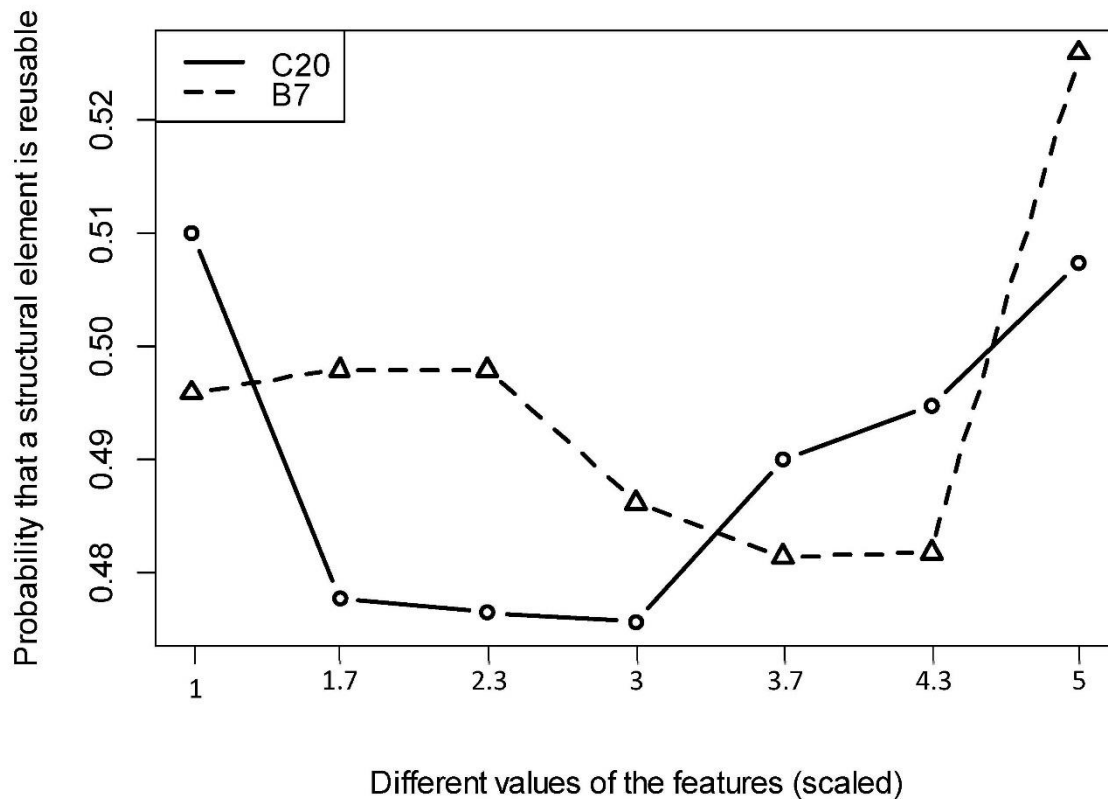
Figure 6.6 The impact of different values the features on the reusability probabilities of the elements (sensitivity analysis) for C20 and B7 (TEC-RF BSE-RPM)
