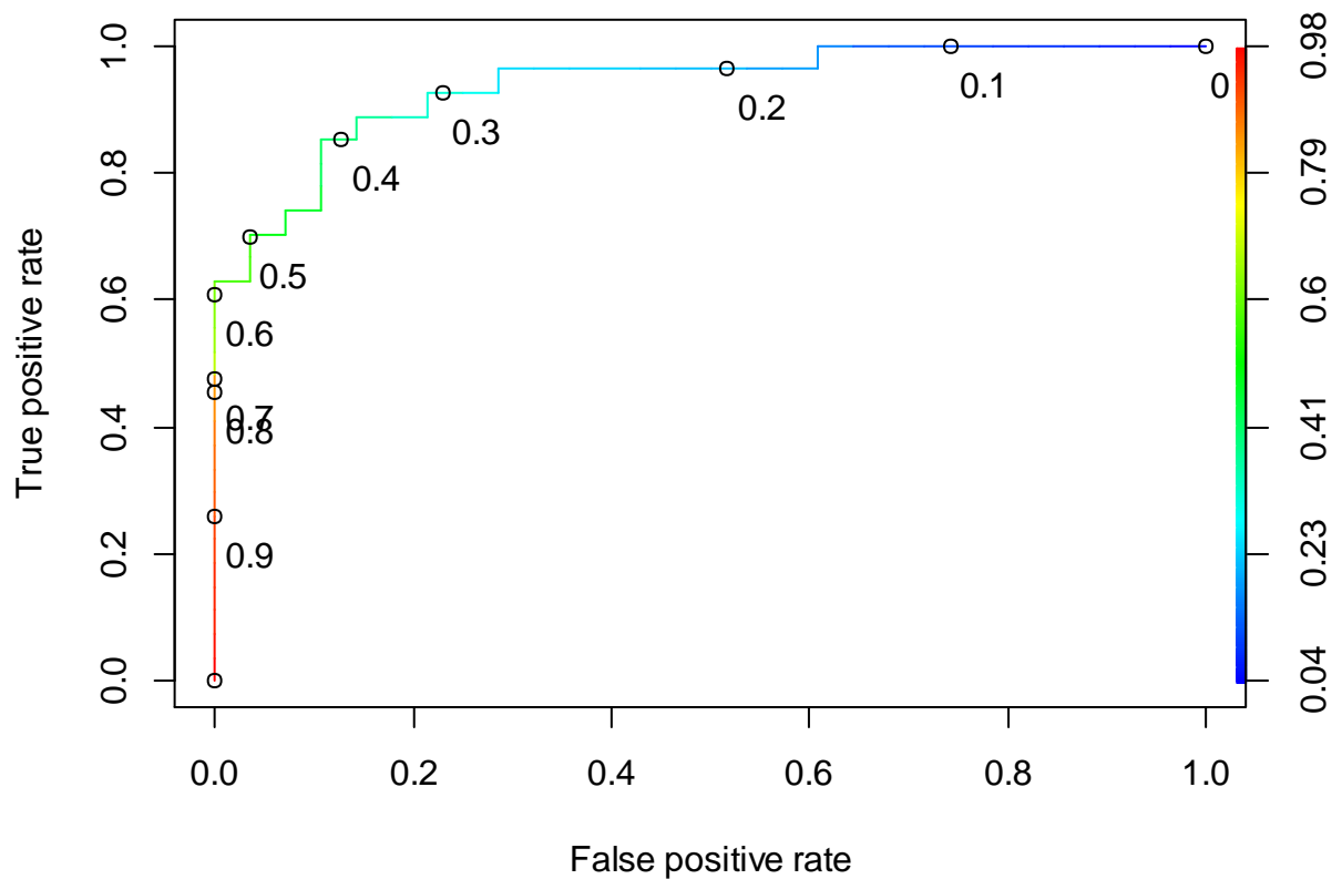
Figure F-23 The ROC curve of the AB BSE-RPM (ECO dataset)
