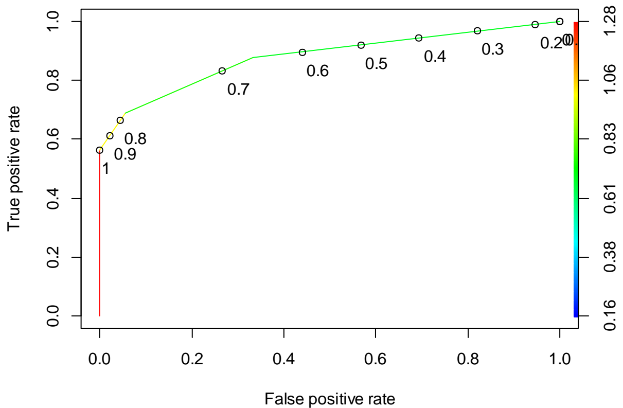
Figure F-34 The ROC curve of the DT BSE-RPM (SOC dataset)
