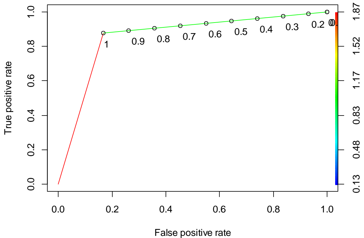
Figure F-41 The ROC curve of the PRL BSE-RPM (SOC dataset)
