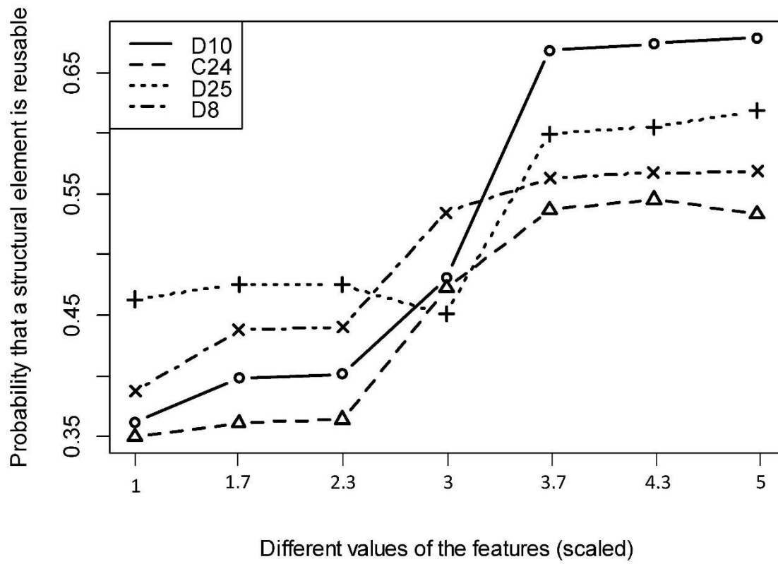
Figure 6.9 The impact of different values the features on the reusability probabilities of the elements (sensitivity analysis) for D10, C24, D25, and D8 (the top-four variables in ECO-RF BSE-RPM)
