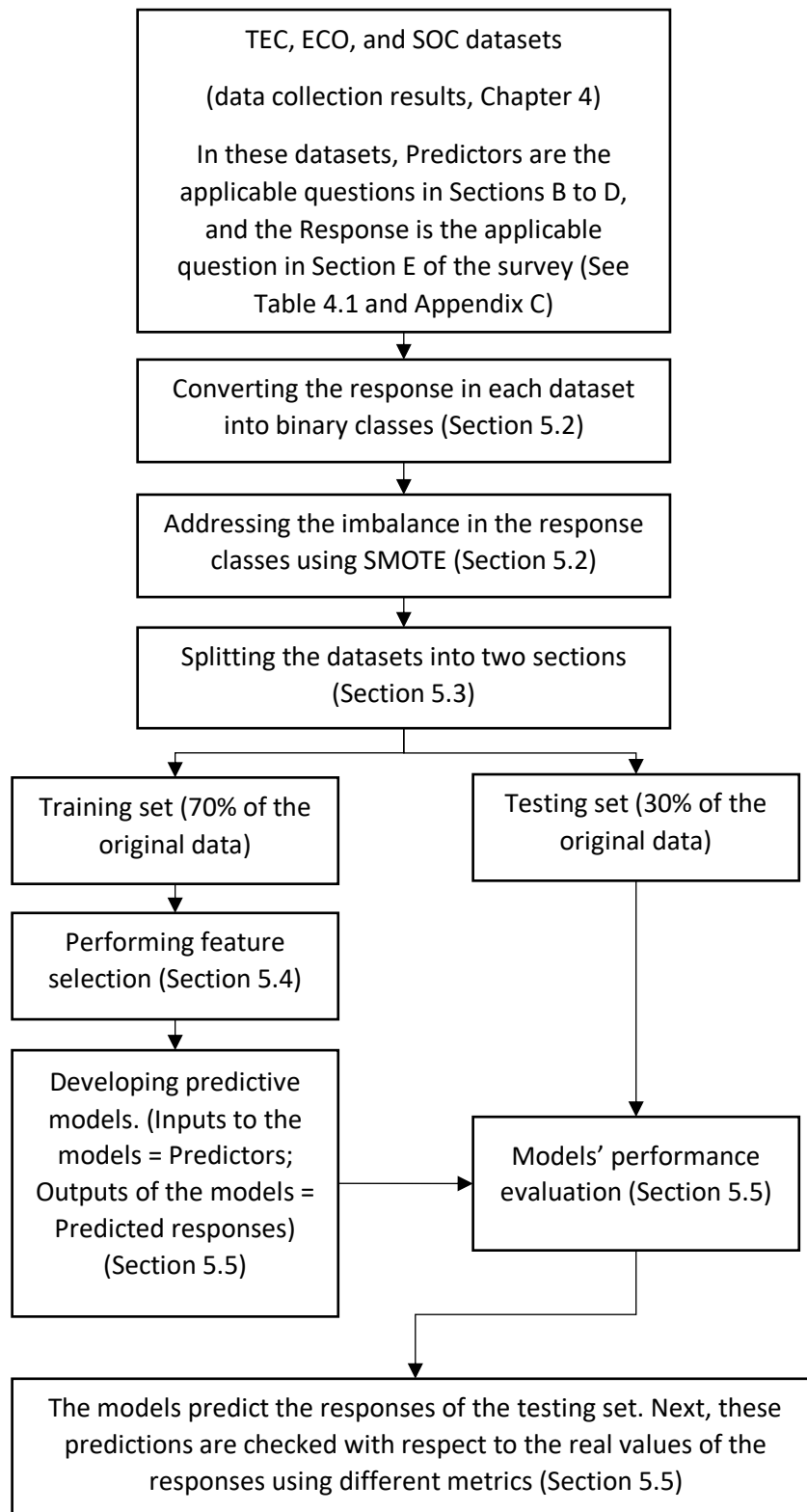
Figure 5.15 Summary of the process of developing the predictive models in Chapter 5
