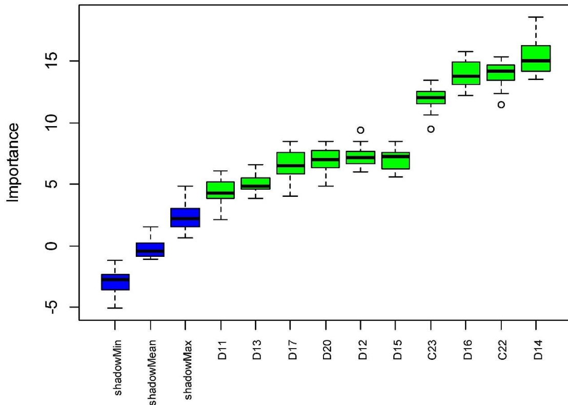
Figure 5.3 Importance of the features in the SOC dataset using the Boruta method
