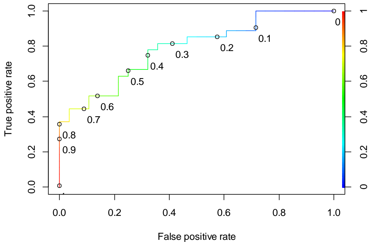
Figure F-17 The ROC curve of the LDA BSE-RPM (ECO dataset)
