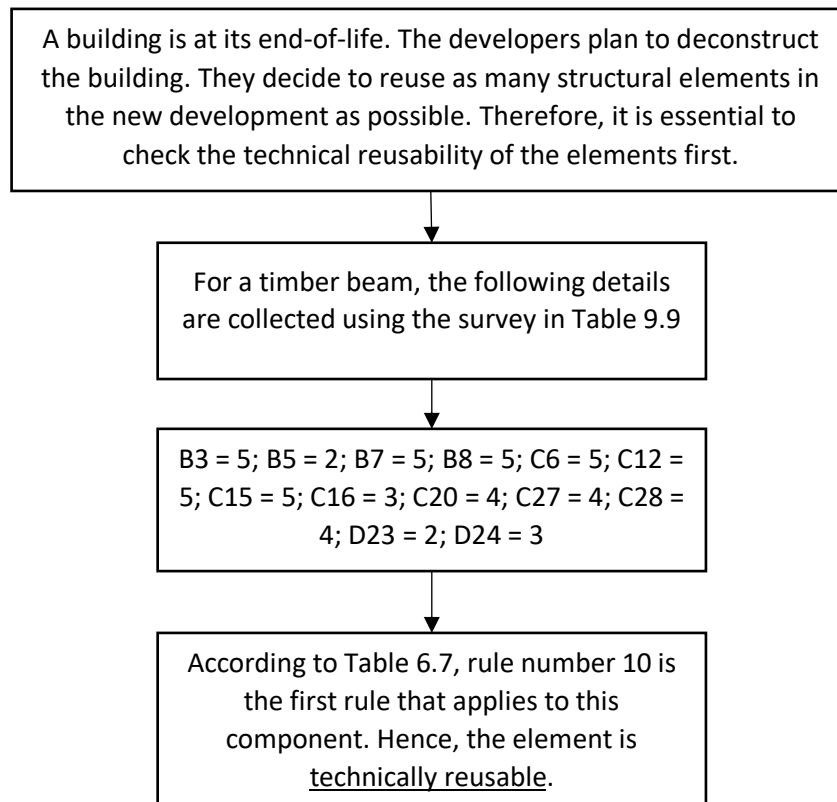
Figure 6.18 An example of using the learner presented in Table 6.7 for predicting the technical reusability of a timber beam
