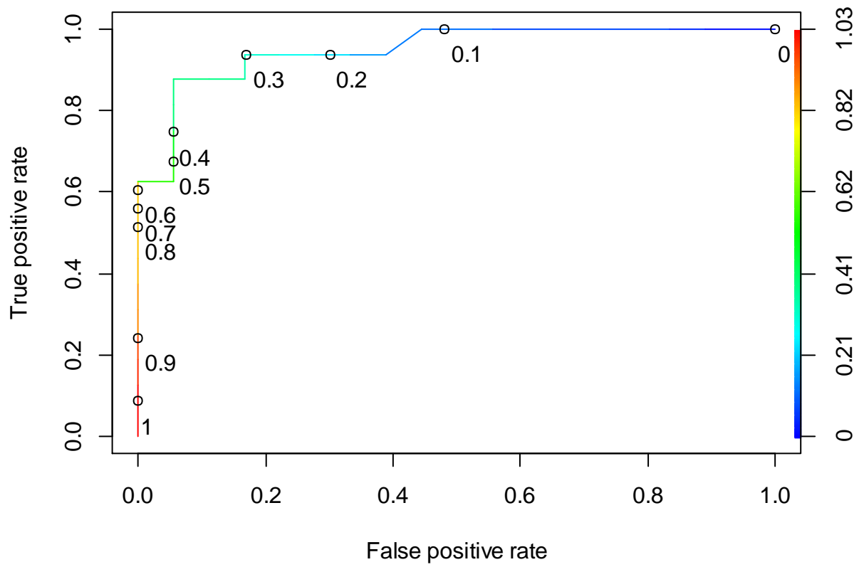
Figure F-29 The ROC curve of the KNN BSE-RPM (SOC dataset)
