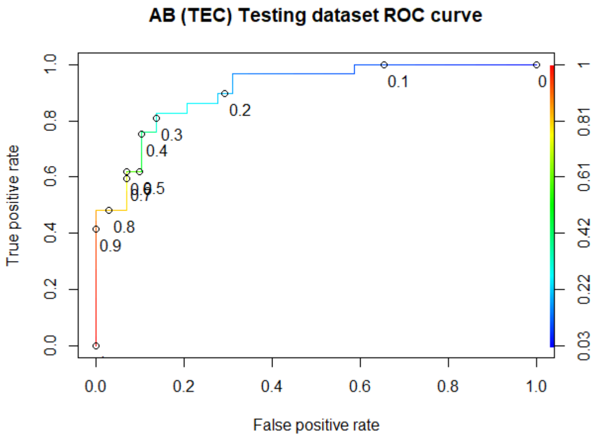
Figure F-9 The ROC curve of the AB BSE-RPM (TEC dataset)
