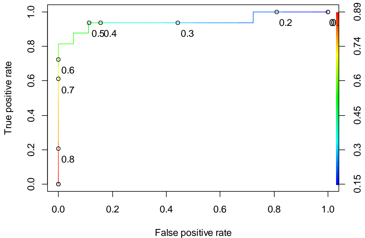
Figure F-37 The ROC curve of the AB BSE-RPM (SOC dataset)
