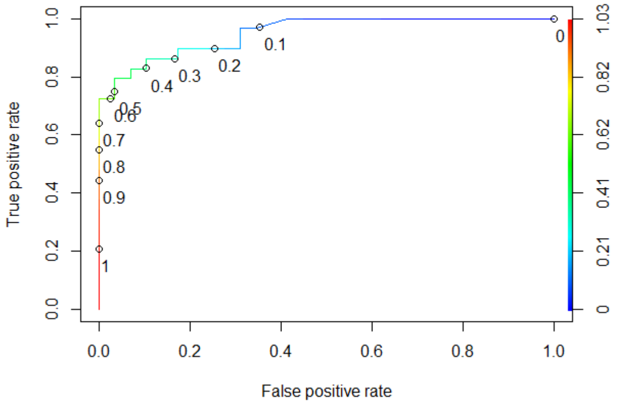
Figure F-1 The ROC curve of the KNN BSE-RPM (TEC dataset)
