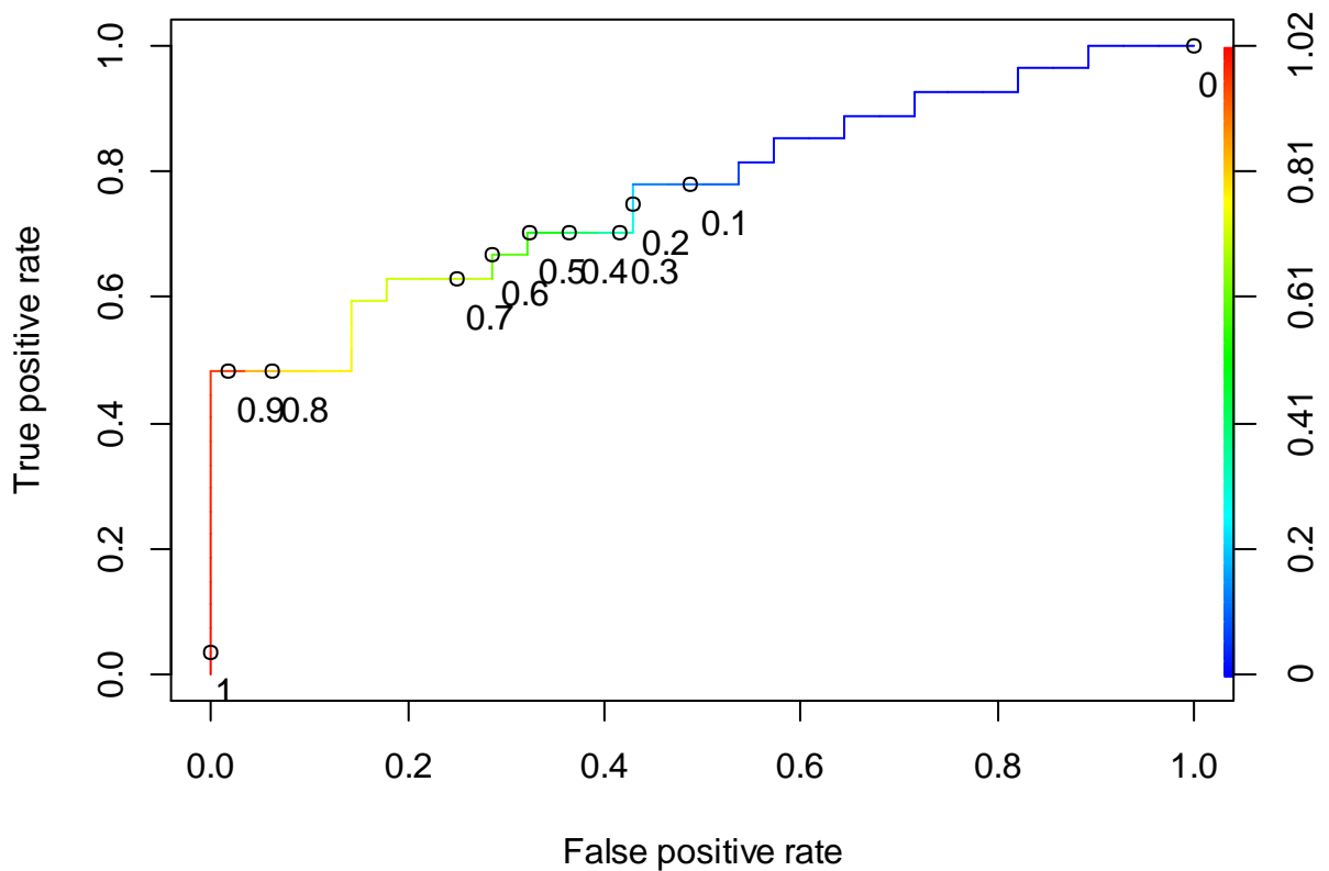
Figure F-19 The ROC curve of the NB BSE-RPM (ECO dataset)
