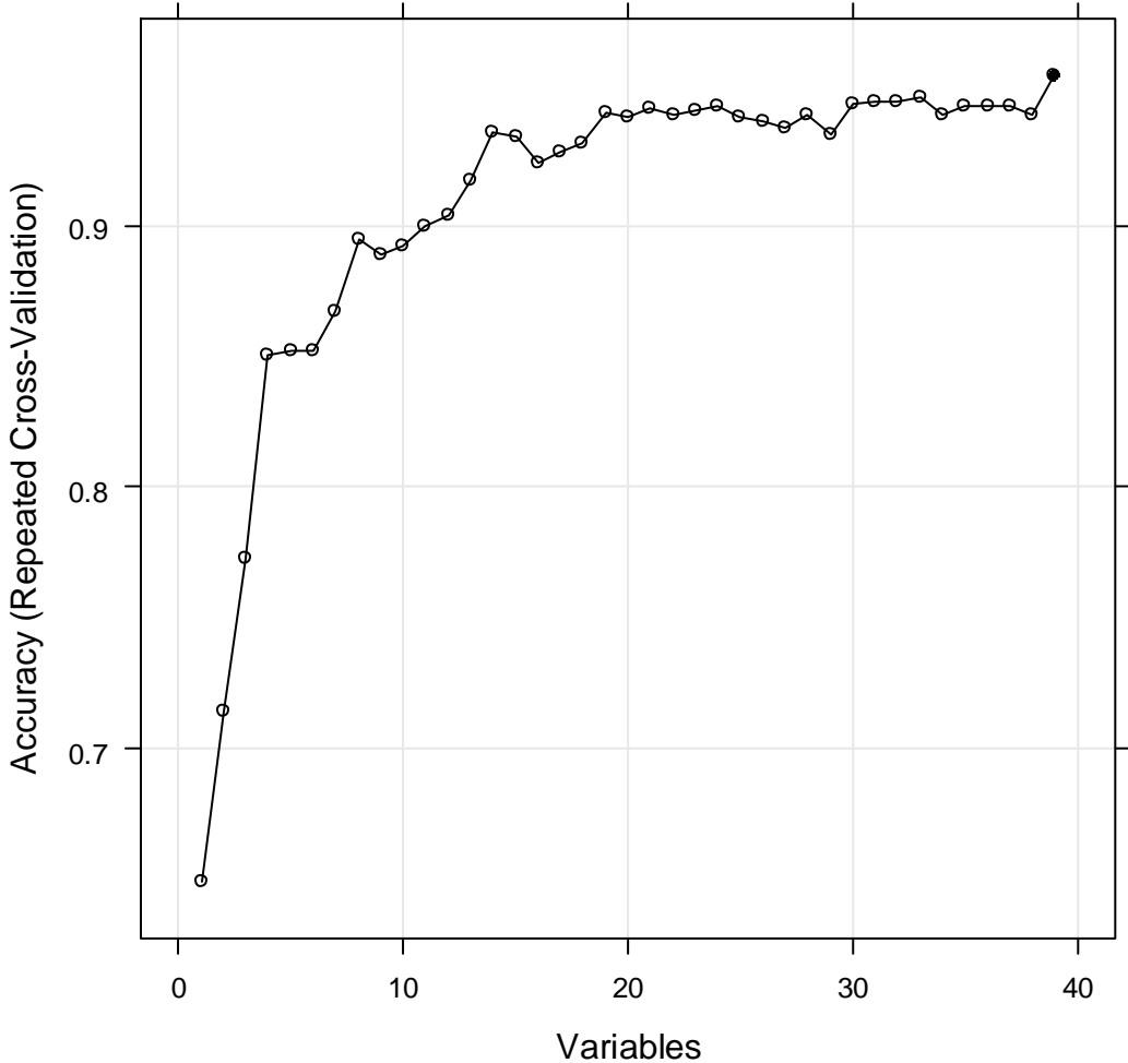
Figure 5.4 Performance of the RFE and Random Forests based on the ranks of the features (TEC dataset)
