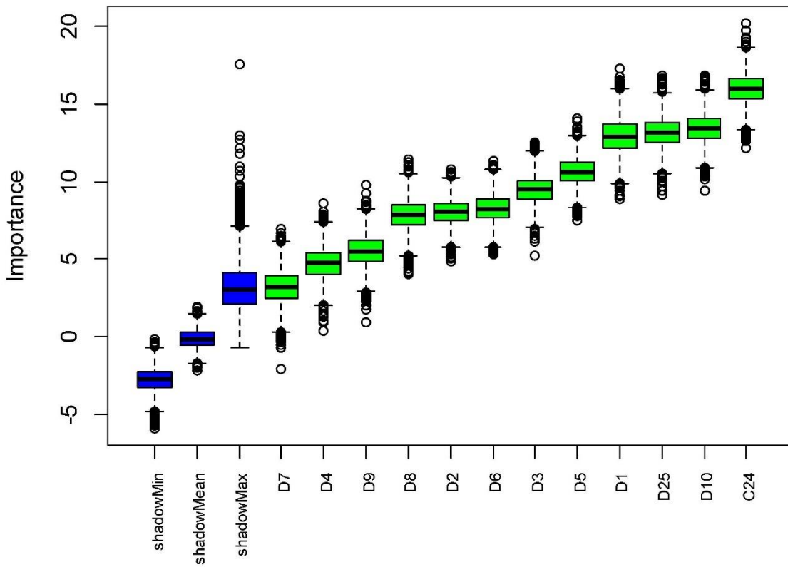
Figure 5.2 Importance of the features in the ECO dataset using the Boruta method
