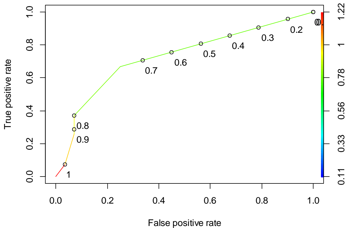
Figure F-27 The ROC curve of the PRL BSE-RPM (ECO dataset)
