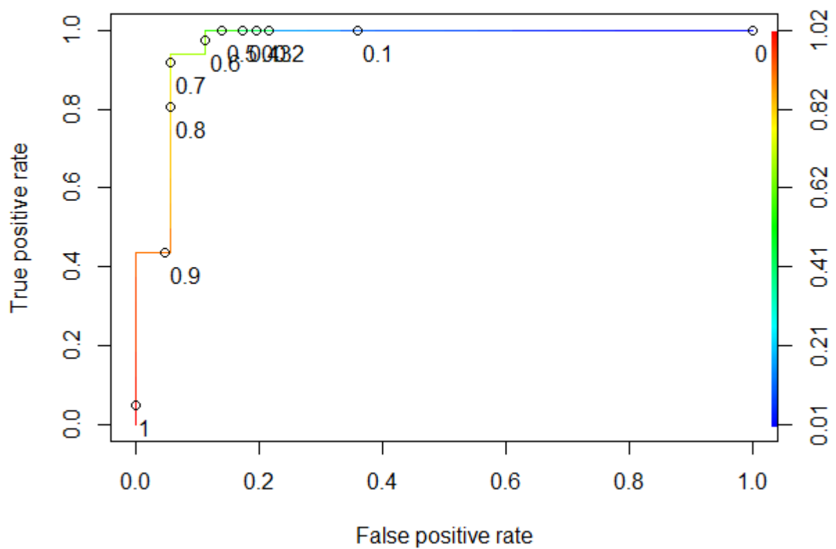
Figure F-42 The ROC curve of the SVM BSE-RPM (SOC dataset)
