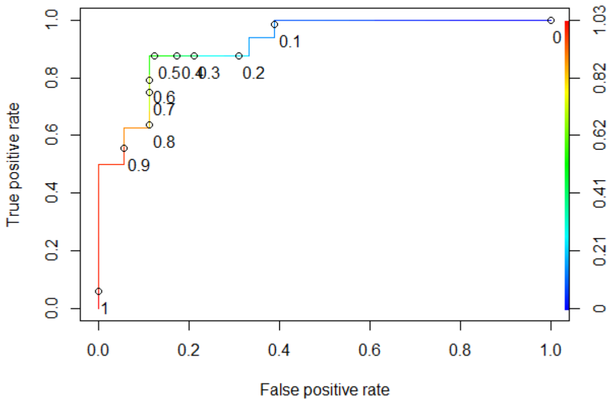
Figure F-39 The ROC curve of the ANN BSE-RPM (SOC dataset)
