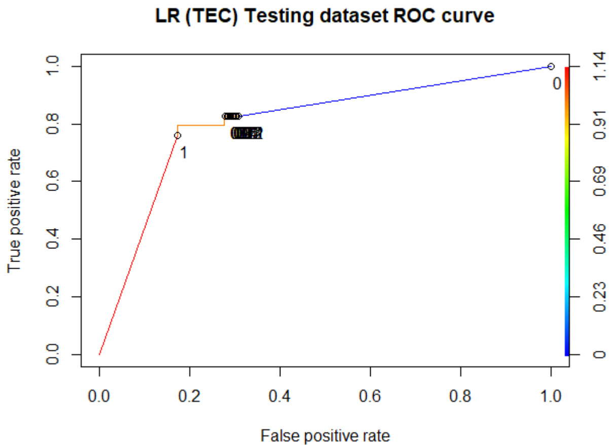
Figure F-2 The ROC curve of the LR BSE-RPM (TEC dataset)
