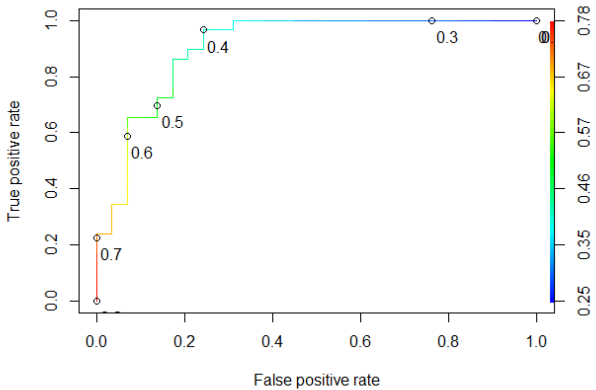
Figure F-12 The ROC curve of the GP BSE-RPM (TEC dataset)
