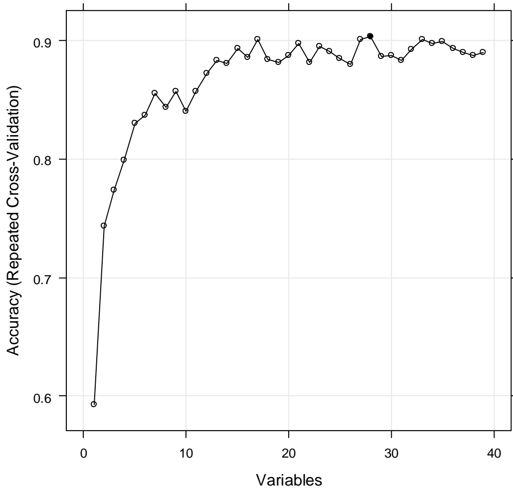
Figure 5.6 Performance of the RFE and Decision Trees (Bagging) based on the ranks of the features (TEC dataset)
