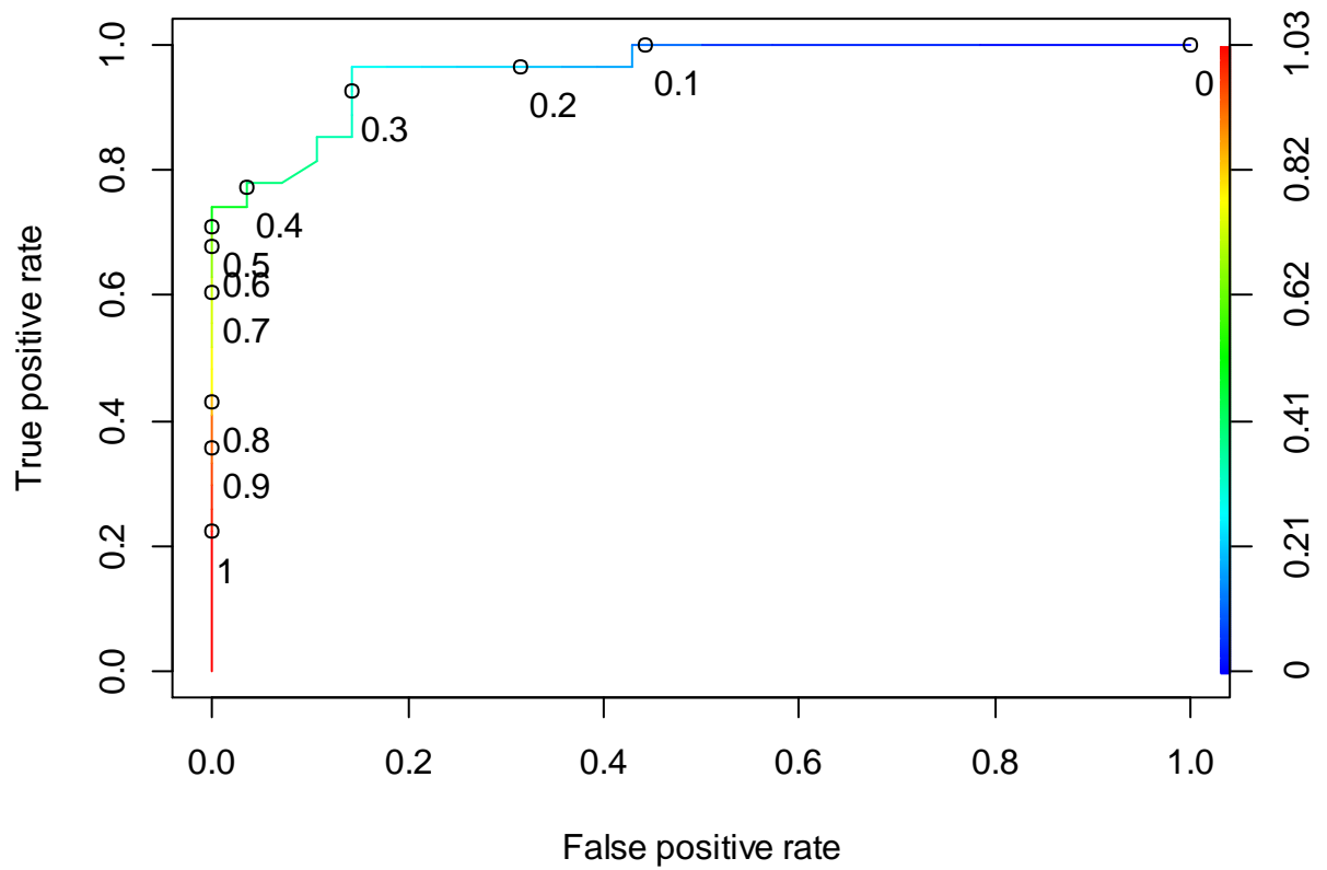
Figure F-15 The ROC curve of the KNN BSE-RPM (ECO dataset)
