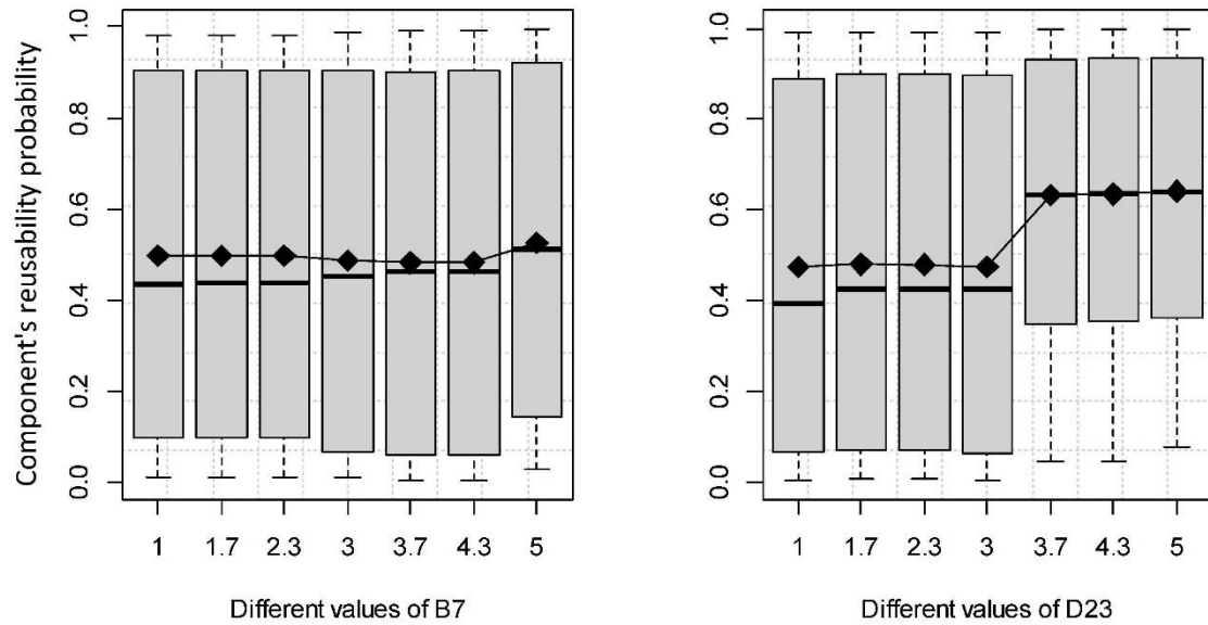
Figure 6.7 The VEC curves with box plots (to show the range of sensitivity at each point) to compare the impact of different values of B7 (left) and D23 (right) on the reusability probabilities of the elements (TEC-RF BSE-RPM)
