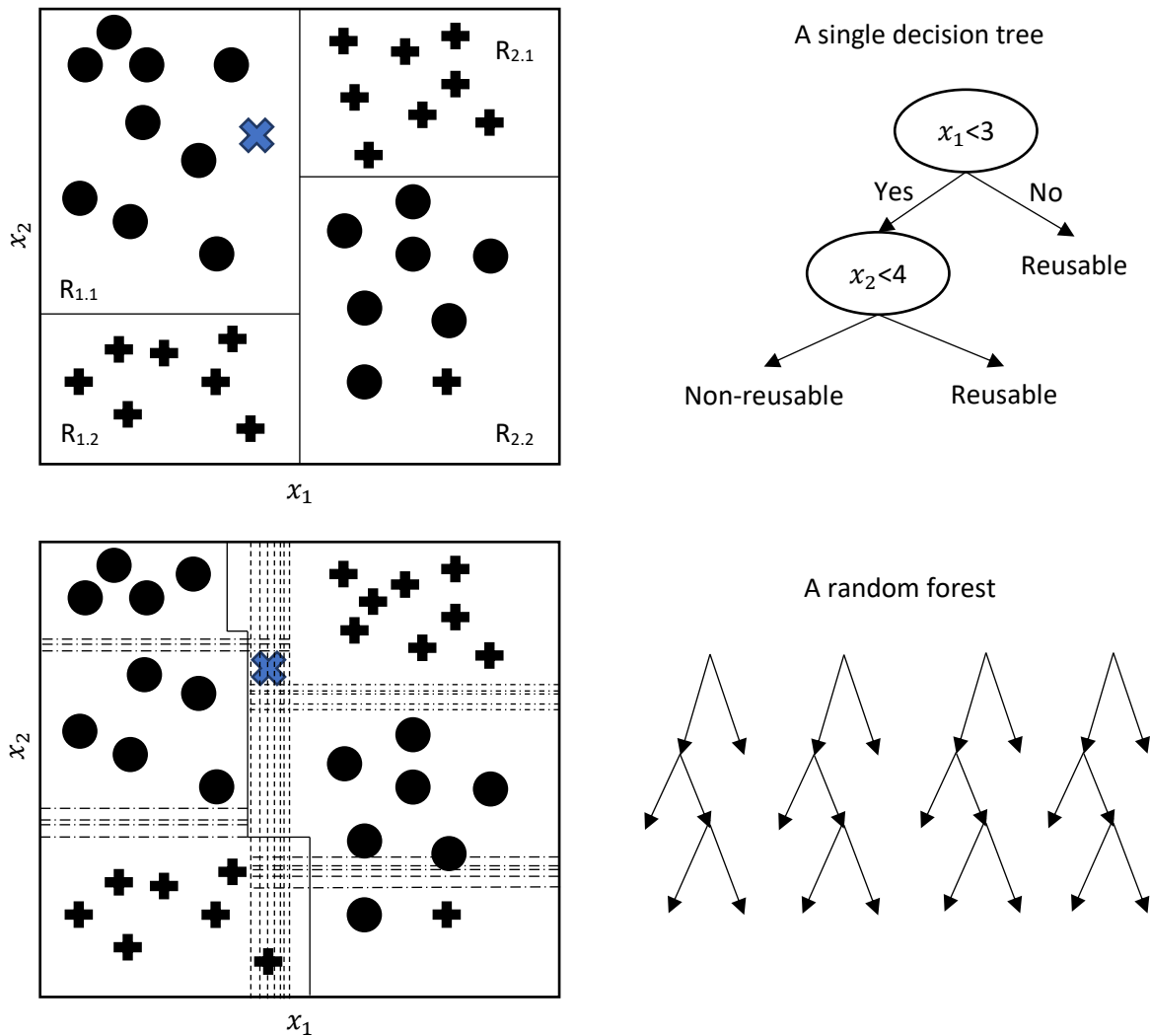
Figure 5.11 A simplified Random Forest. Top: A Decision Tree (top right) divides the feature space (top left). Bottom: A Random Forest which is a group of Decision Trees (bottom right) divide the feature space (bottom left). The cross is a new observation.
