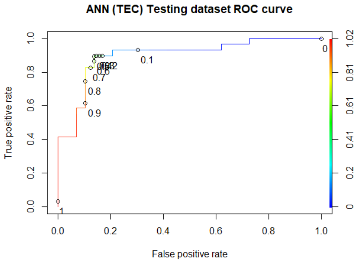
Figure F-11 The ROC curve of the ANN BSE-RPM (TEC dataset)
