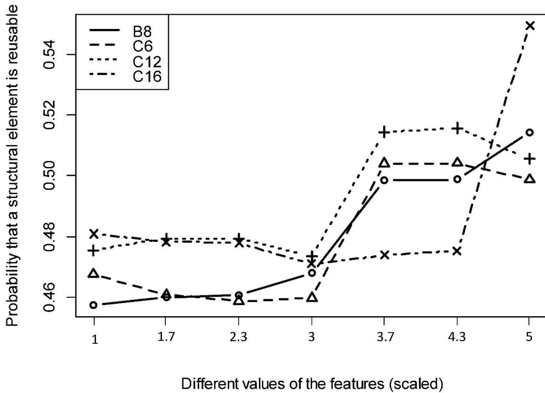
Figure 6.5 The impact of different values the features on the reusability probabilities of the elements (sensitivity analysis) for B8, C6, C12, and C16 (TEC-RF BSE-RPM)
