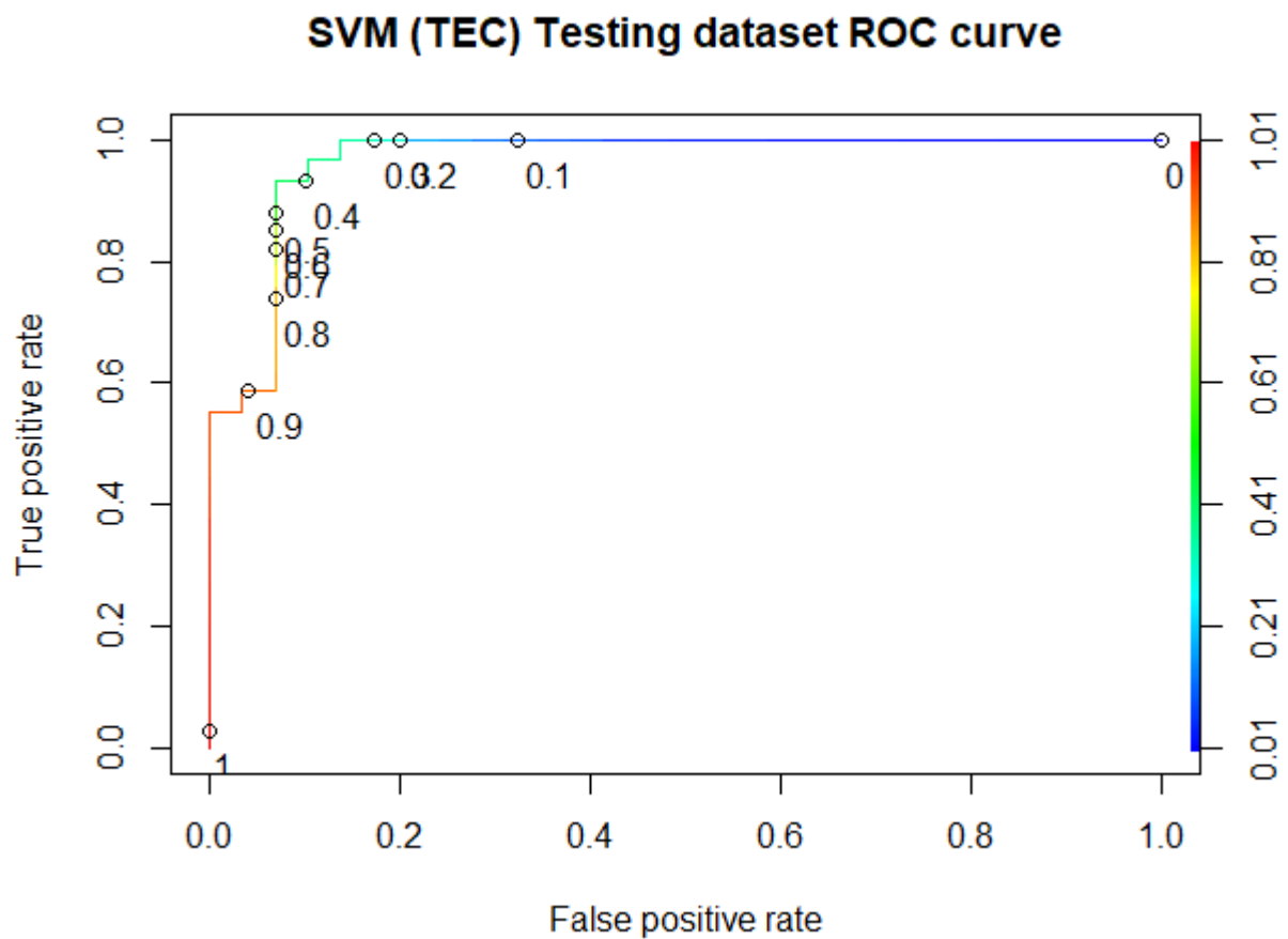
Figure F-14 The ROC curve of the SVM BSE-RPM (TEC dataset)
