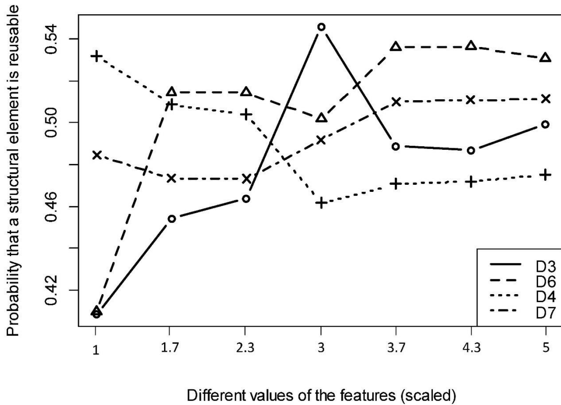
Figure 6.11 The impact of different values the features on the reusability probabilities of the elements (sensitivity analysis) for D3, D6, D4, and D7 (ECO-RF BSE-RPM)
