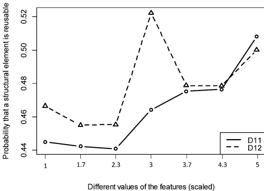
Figure 6.16 The impact of different values the features on the reusability probabilities of the elements (sensitivity analysis) for D11 and D12 (SOC-RF BSE-RPM)
