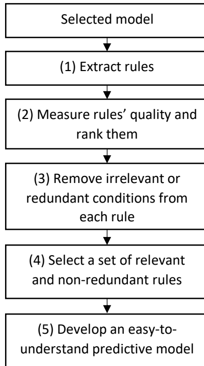
Figure 6.1 The process of developing the rules set from the selected BSE-RPMs (Deng 2014)
