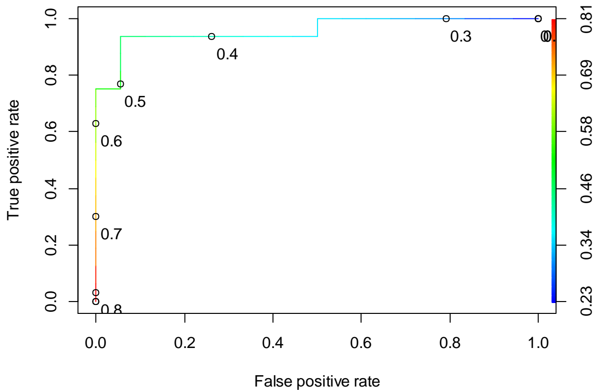
Figure F-40 The ROC curve of the GP BSE-RPM (SOC dataset)
