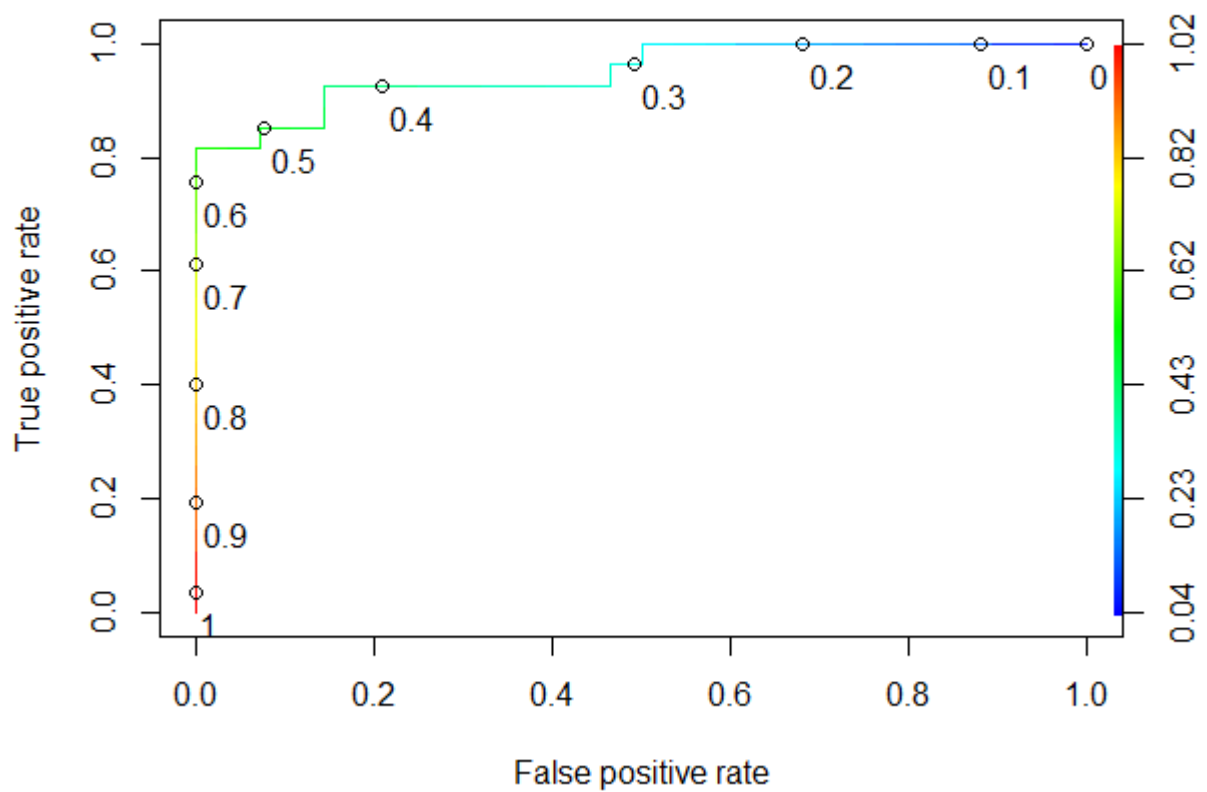
Figure F-28 The ROC curve of the SVM BSE-RPM (ECO dataset)
