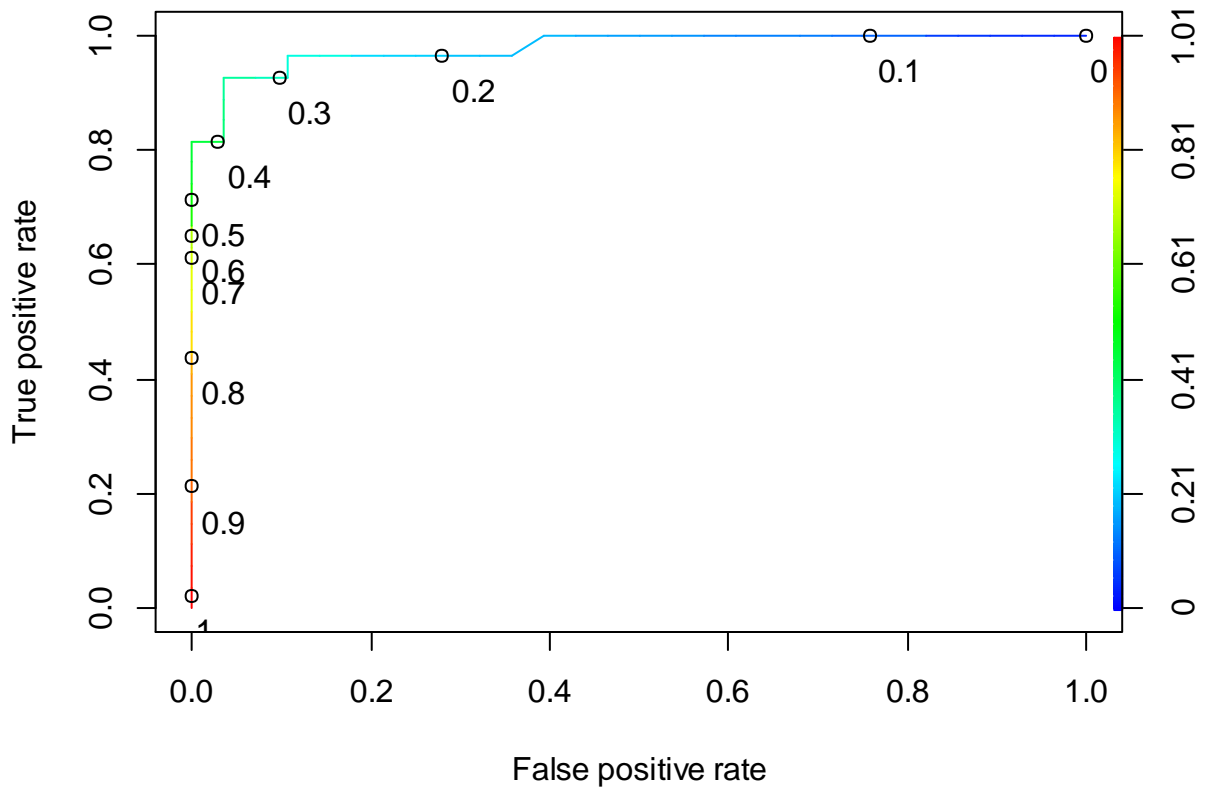
Figure F-22 The ROC curve of the RF BSE-RPM (ECO dataset)
