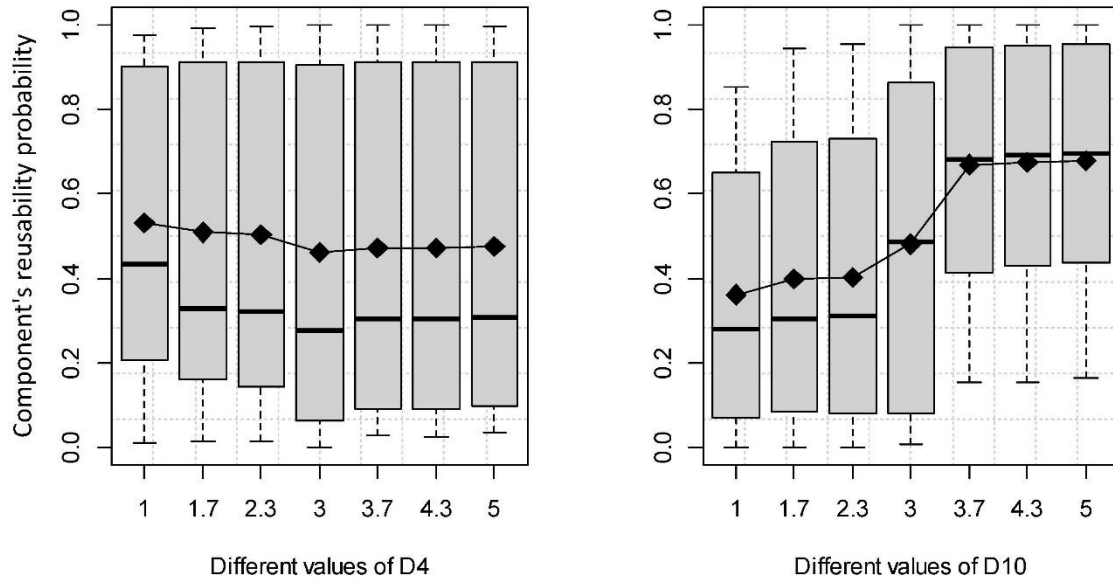
Figure 6.12 The VEC curves with box plots (to show the range of sensitivity at each point) to compare the impact of different values of D4 (left) and D10 (right) on the reusability probabilities of the elements (ECO-RF BSE-RPM)
