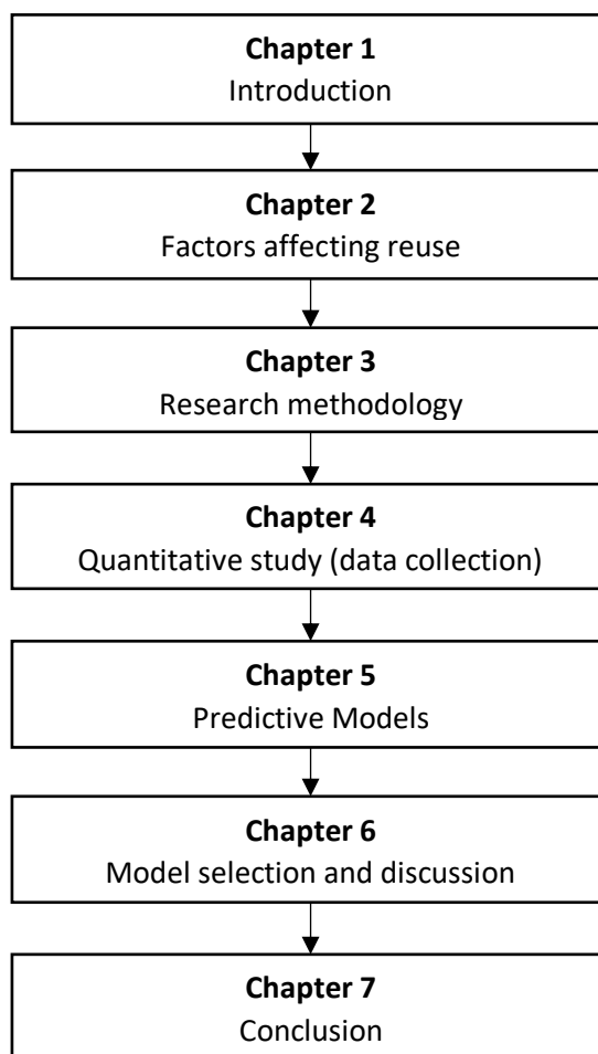
Figure 1.2 Thesis structure.
