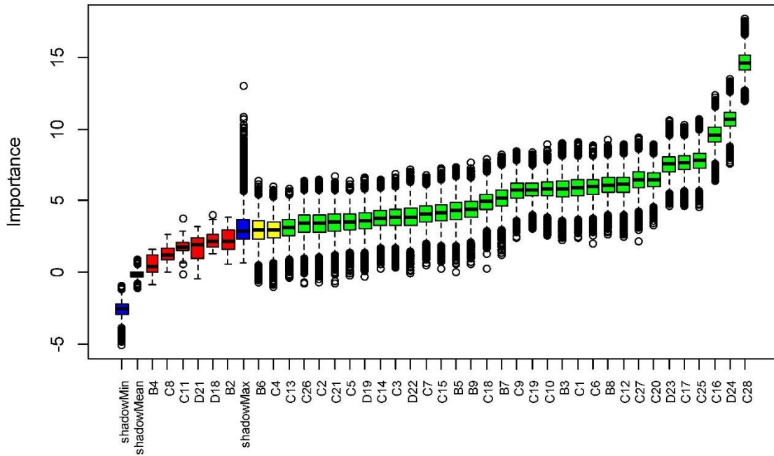
Figure 5.1 Importance of the features in the TEC dataset using the Boruta method
