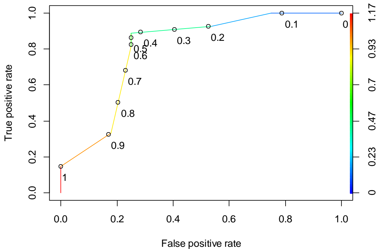
Figure F-20 The ROC curve of the DT BSE-RPM (ECO dataset)
