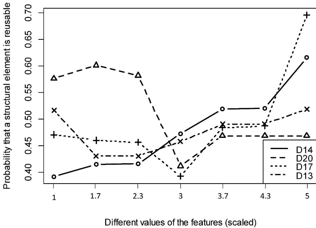
Figure 6.15 The impact of different values the features on the reusability probabilities of the elements (sensitivity analysis) for D14, D20, D17, and D13 (SOC-RF BSE-RPM)
