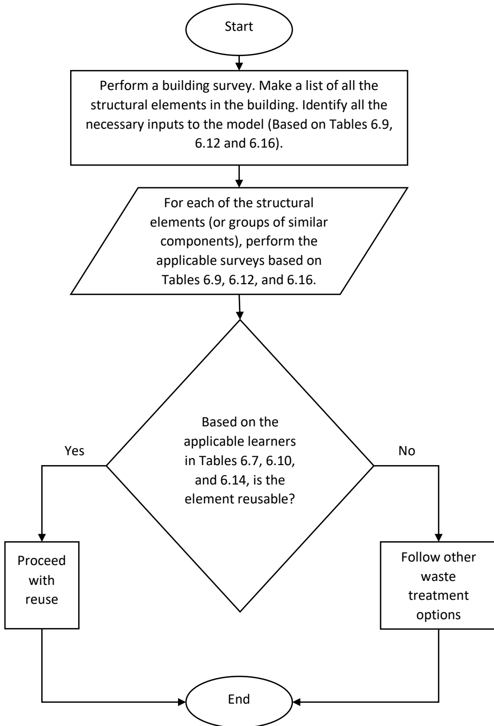
Figure 6.17 Instructions for using the learners developed in Tables 6.7, 6.10, and 6.14
