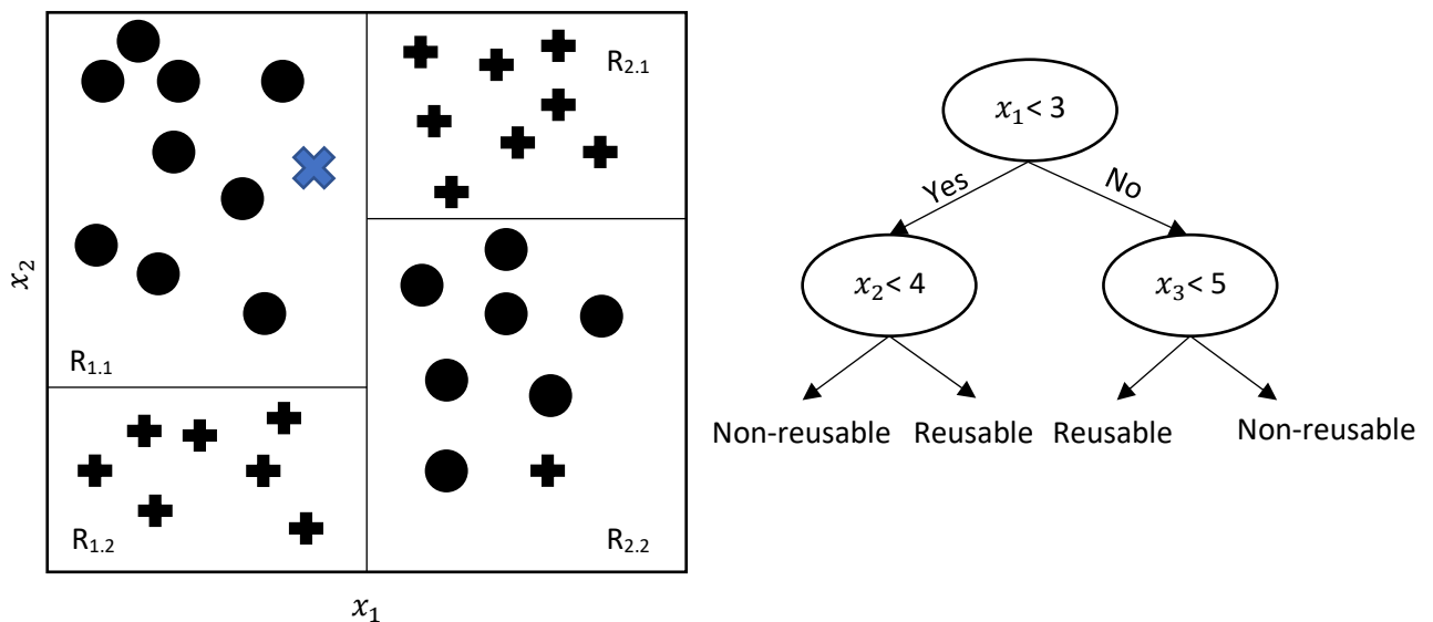
Figure 5.10 The Decision Trees (DT) method
