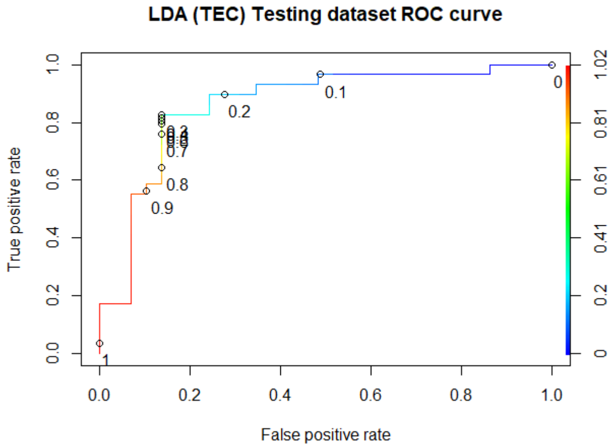
Figure F-3 The ROC curve of the LDA BSE-RPM (TEC dataset)
