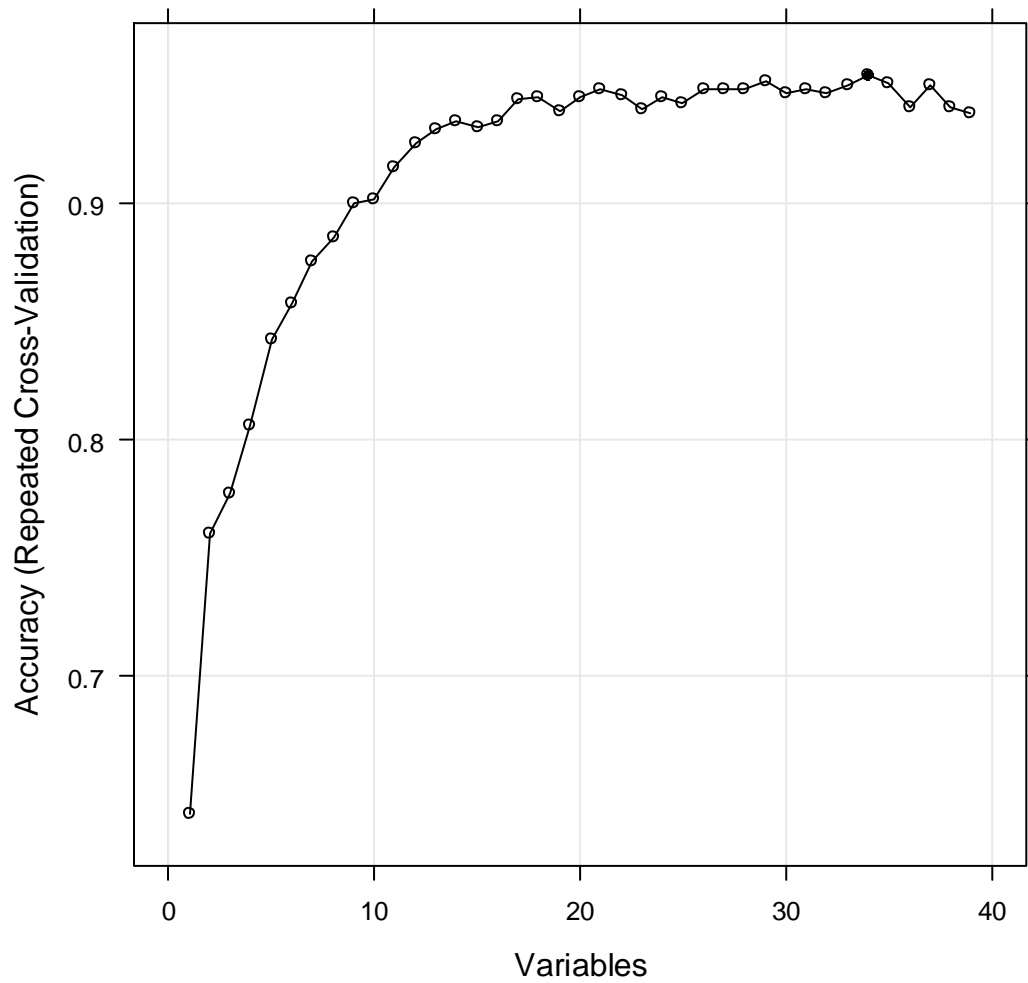
Figure 5.7 Performance of the RFE and Caret Function (Random Forests) based on the ranks of the features (TEC dataset)
