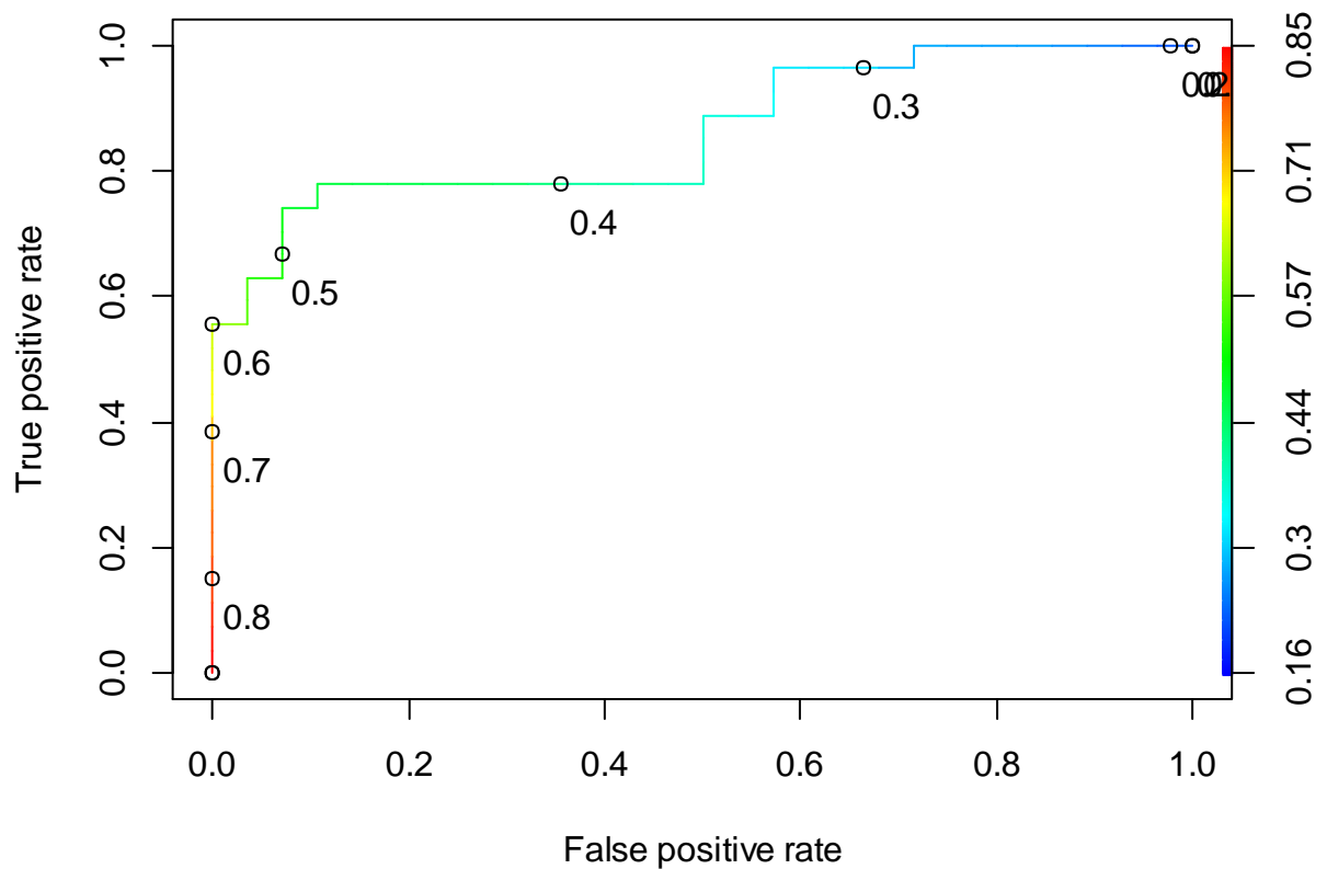
Figure F-26 The ROC curve of the GP BSE-RPM (ECO dataset)
