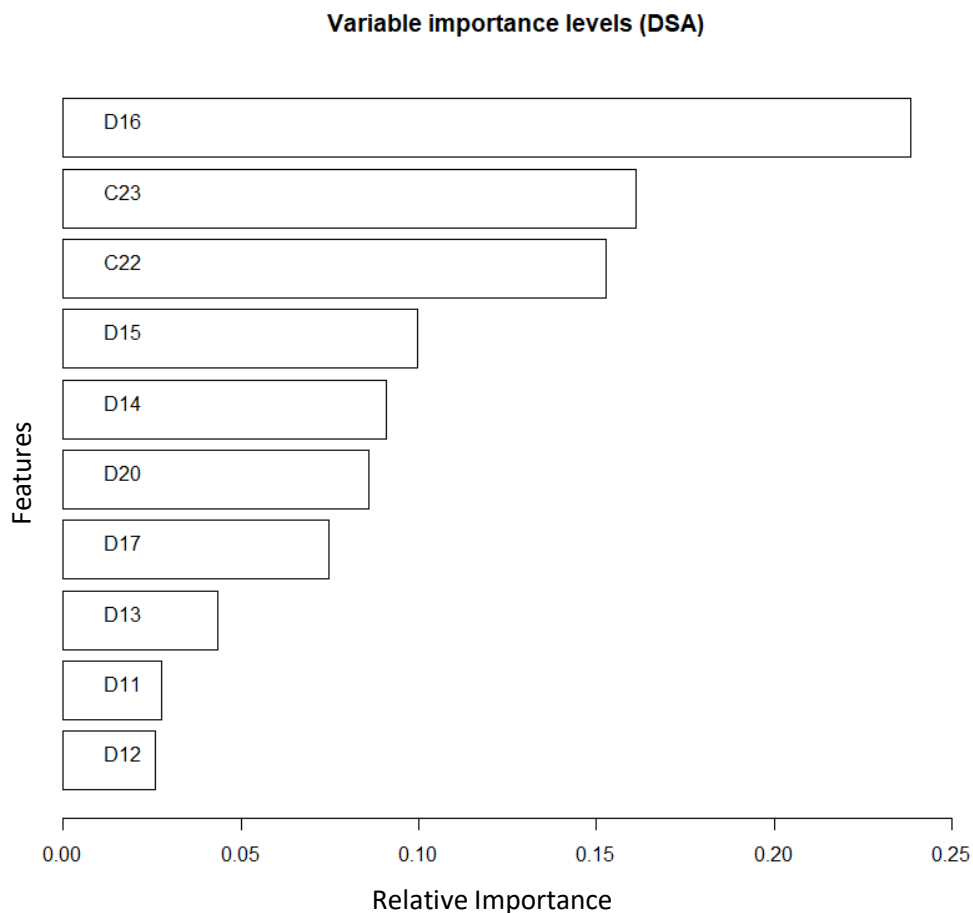
Figure 6.13 Bar plot with DSA and AAD relative feature importance for the ECO dataset based on the SOC-RF BSE-RPM
