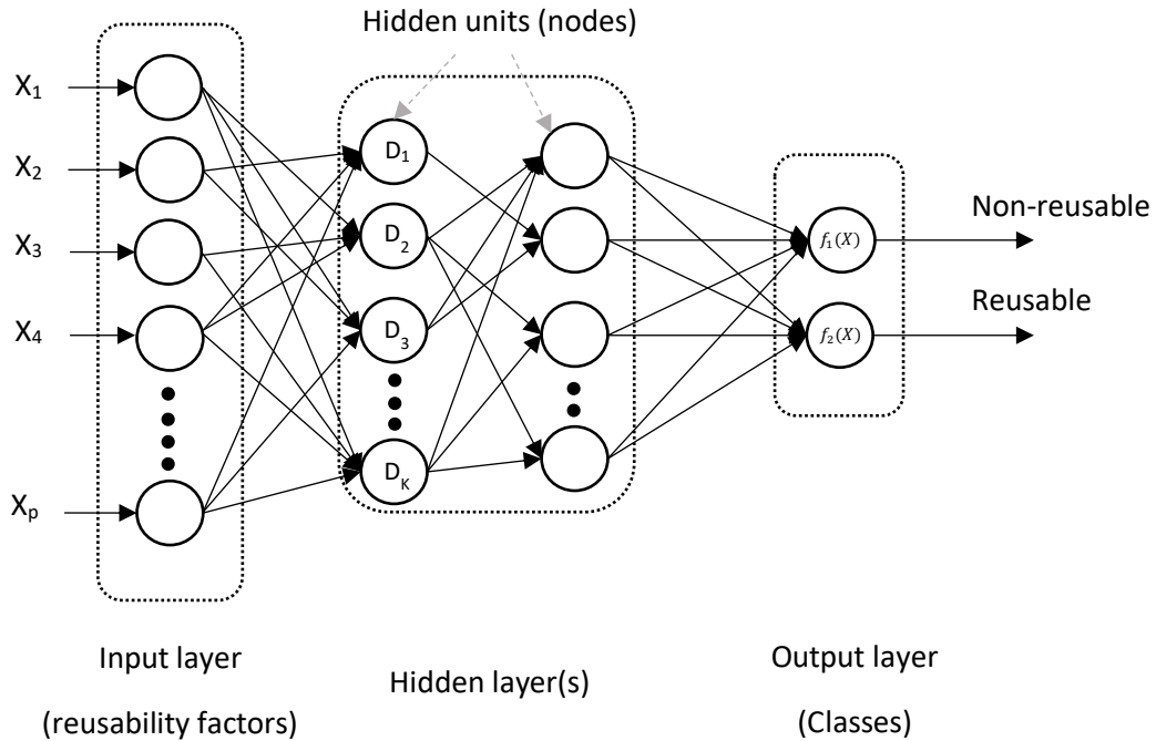
Figure 5.12 The Artificial Neural Networks (ANN) architecture (two hidden layers)
