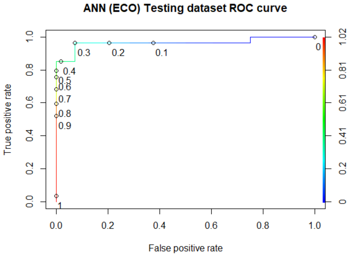
Figure F-25 The ROC curve of the ANN BSE-RPM (ECO dataset)
