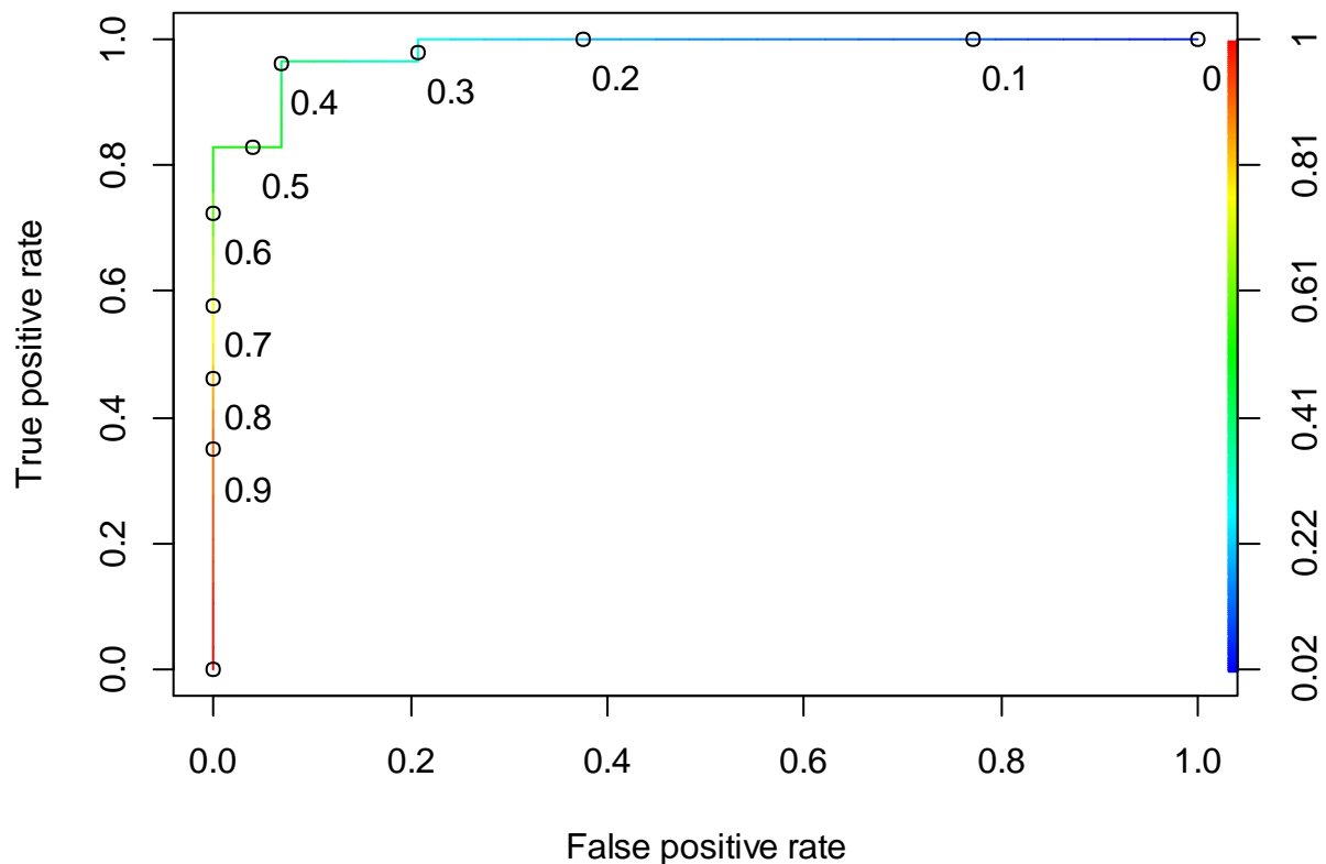
Figure 5.14 The ROC curve of the RF BSE-RPM (TEC dataset) (AUC = 0.98)
