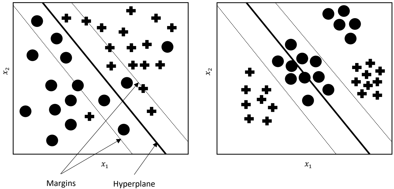
Figure 5.13 The Support Vector Classifier
