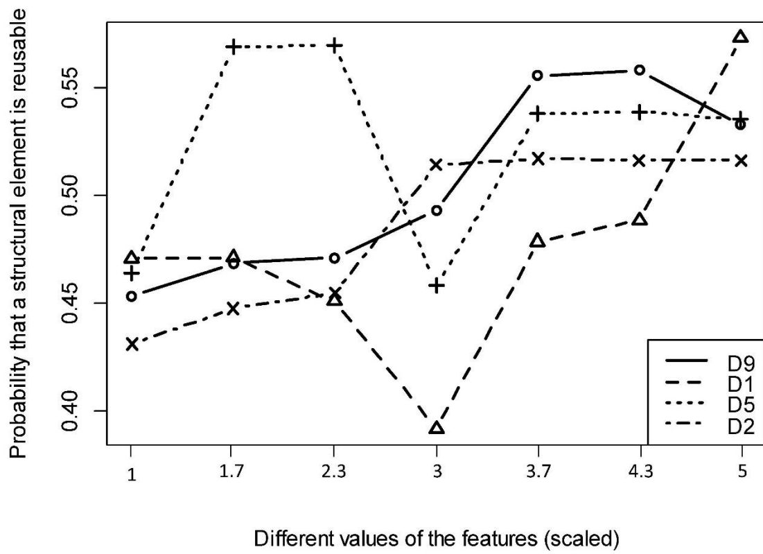
Figure 6.10 The impact of different values the features on the reusability probabilities of the elements (sensitivity analysis) for D9, D1, D5, and D2 (ECO-RF BSE-RPM)
