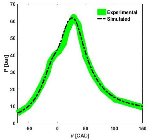
Figure 10: simulated in-cylinder pressure for gasoline-fueled EF7TC
