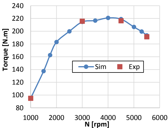
Figure 9: Simulated brake torque via experimental results for CNG fueled EF7TC
