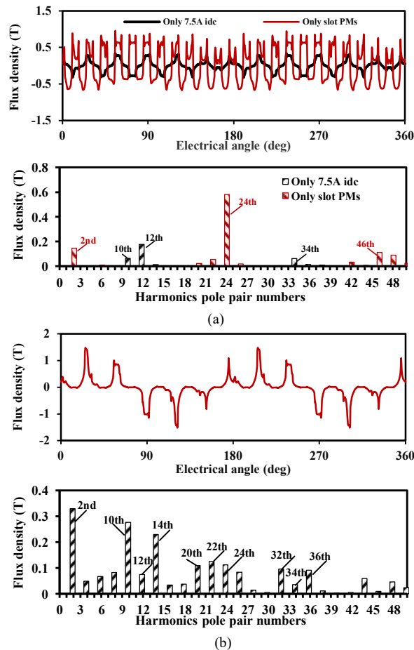
Fig. 4. Air gap flux density waveforms and harmonics distribution. (a) DC field or slot PMs excitation. (b) Armature excitation.
