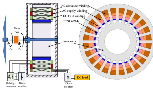
Fig. 1. Wind power generation system based on the proposed SPMa-HRG.
