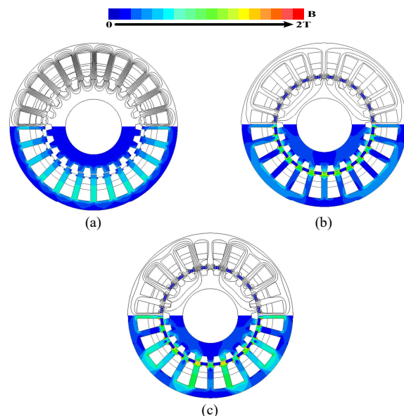
Fig. 3. No-load magnetic field distribution. (a) DC field excitation only. (b) Slot PMs excitation only. (c) Both DC field and slot PMs excitation.
