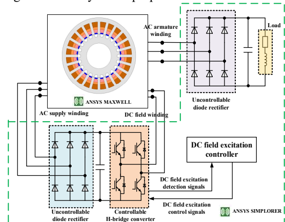
Fig. 8. Field-circuit coupled model for the proposed SPMa-HRG.
