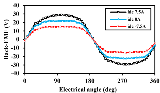
Fig. 10. Back-EMF waveforms with bidirectional DC field current.
