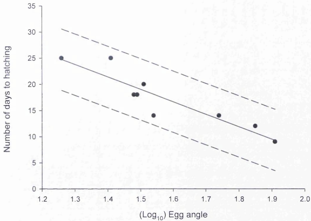
Figure 2.3 Relationship between the unsuspended egg angle and the number of days before the observed hatching date. The linear regression equation y = 54.56 - 23.68 \text{ Log}_{10}x describes the 'reference flotation model' that was used to obtain a measure of hatching date for breeding attempts where eggs were floated. The dotted lines represent the upper and lower 95% confidence limits for individual predictions.
