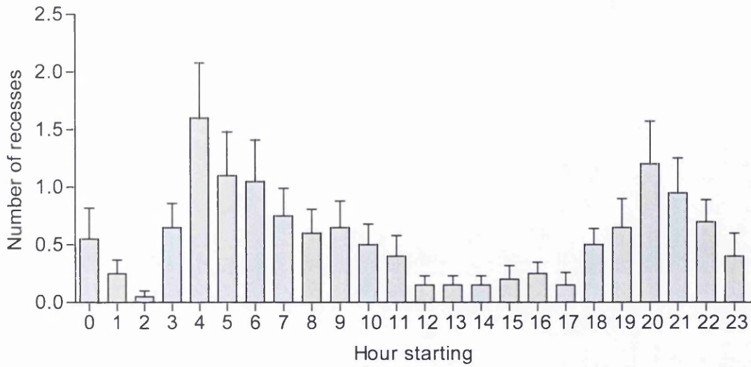
Figure 6.1 Number of incubation recesses through the day for red-throated diver, Mainland Shetland, Scotland, 2006-2007.
