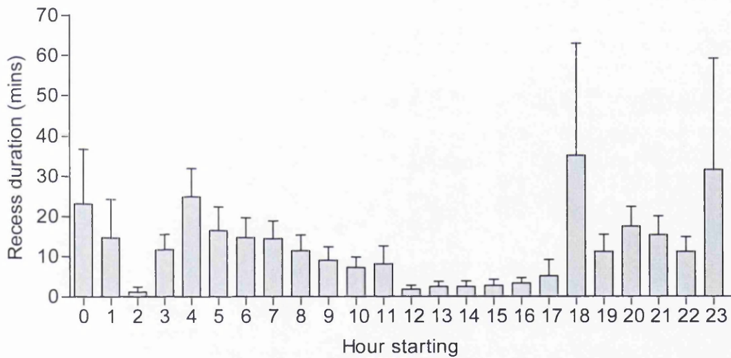
Figure 6.2 Duration of incubation recesses through the day for red-throated diver, Mainland Shetland, Scotland, 2006-2007.
