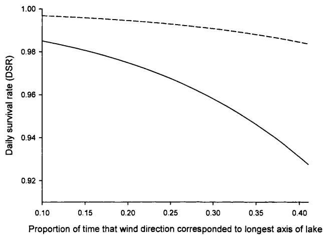
Figure 5.6 Daily survival rates (DSR) for red-throated diver estimated for the best supported model at the breeding lake and regional scales with an additive effect of the proportion of time that wind direction corresponded with the longest axis of the lake and lake elevation (model 2). Solid line represents a hypothetical nest at 10m a.s.l. and the dotted line a nest at 250m a.s.l. The model uses egg and chick stage survival information.
