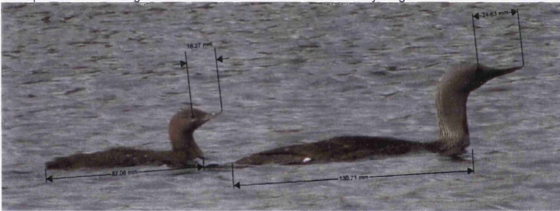
Figure 2.2 Measuring red-throated diver relative chick to adult size from photographs. In this example relative bill length is 16.27/24.63 = 0.66 and relative body length = 87.06 \times 130.71 = 0.67
