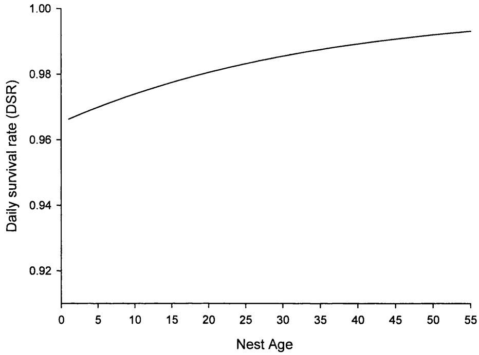
Figure 4.5 Daily survival rate (DSR) for red-throated diver estimated for the fourth best supported model with an individual effect of nest age (model 4). The model uses egg and chick stage survival information.
