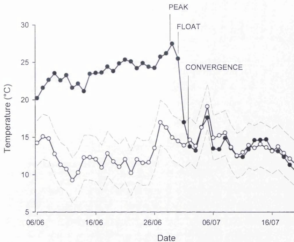
Figure 2.4 An example of a nest and ambient temperature record from 2008 showing mean daily nest temperatures for one nest (solid circles), and mean daily ambient temperature for the same period (open circles). The \pm 3^{\circ}\text{C} limits around the mean daily ambient temperature (dashed lines) is used to determine the date of convergence between nest and ambient temperatures. FLOAT = hatching date based on egg flotation; PEAK = hatching date predicted by the peak mean daily nest temperature model; CONVERGENCE = hatching date predicted by the convergence of nest and ambient temperature model.
