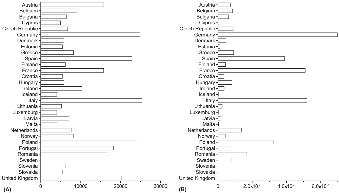
Fig. 1. Sample size and total weight for EHS 2. (A) Sample size (number of respondents). (B) Targeted population (sum of unit weights).
