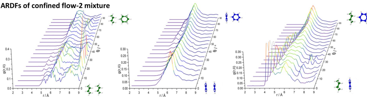
Fig. 6 From left to right, ARDF of like cyclohexane molecules, ARDF of like benzene molecules, ARDF of unlike hydrocarbon molecules in the, from top to bottom, 1:1 bulk mixture, flow 1 and flow
