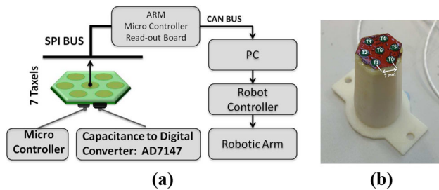
Fig. 2 a The CySkin technology architecture. The hexagonal patch is connected to an Intelligent Hub Board (IHB) that collect the tactile sensor data and send them to the PC through a CAN bus. b The sensorised probe coupled with the CySkin patch used for the experiments
