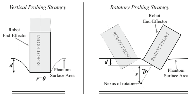
Fig. 3 Diagram of the two probing motions employed. The vertical probing motion is performed when r = 0 and is described by the parameter d . The rotatory motion is performed with r > 0 , and is fully described by both the d and r parameters
