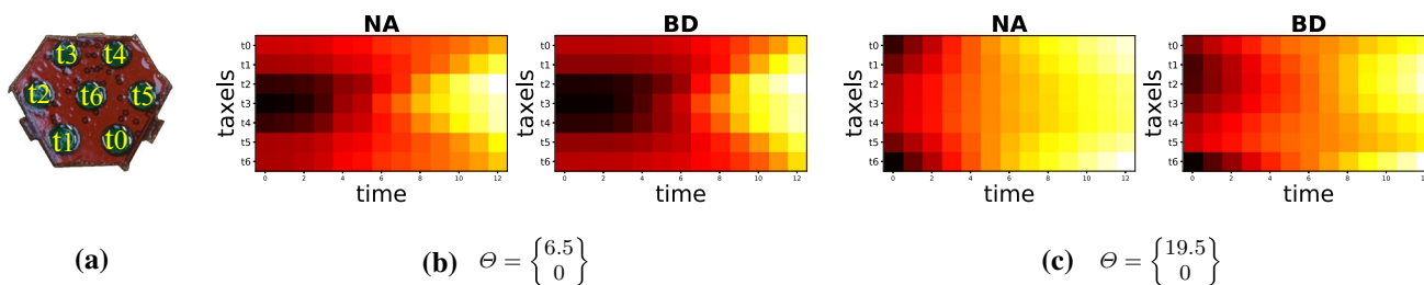
Fig. 6 Raw spatiotemporal tactile image sequences, as captured when probing Ph-2 vertically at varying depths, in an area containing no hand inclusion, and an area containing a 15 mm inclusion placed 20 mm deep.
