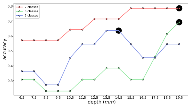
Fig. 18 The classification test accuracy of a multi-class SVM trained on a single sample for each inclusion type, when performing a vertical probing action at different depths, and over varying number of clusters. The highlighted black circles correspond to the maximal silhouette score computed through the proposed framework (see Fig. 13)
