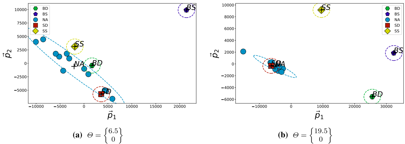
Fig. 14 The 2-dimensional projection of the tactile information generated from probing Ph-2 at varying depths. The ellipses correspond to the distributions of the clusters based on their true inclusion types, at a distance of 2 standard deviations from their respective cluster center
