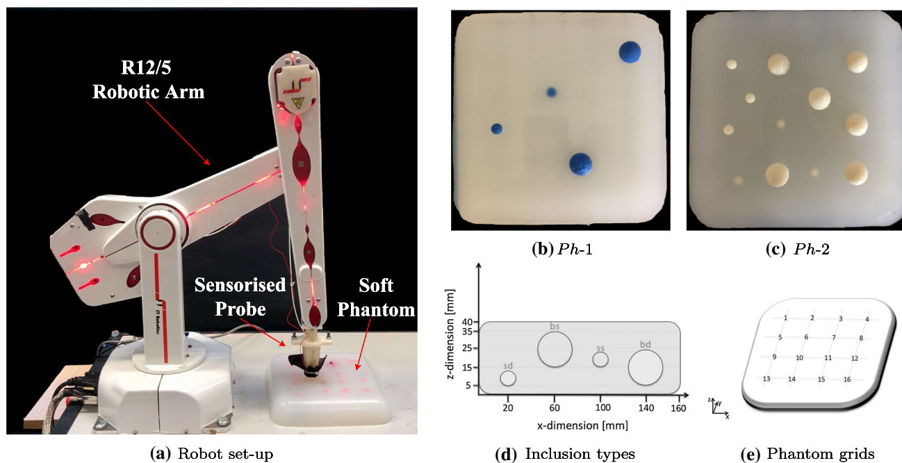
Fig. 1 The figure shows the robotic set-up for the experiments, including a the robot set up and b–e the phantoms developed and their properties
