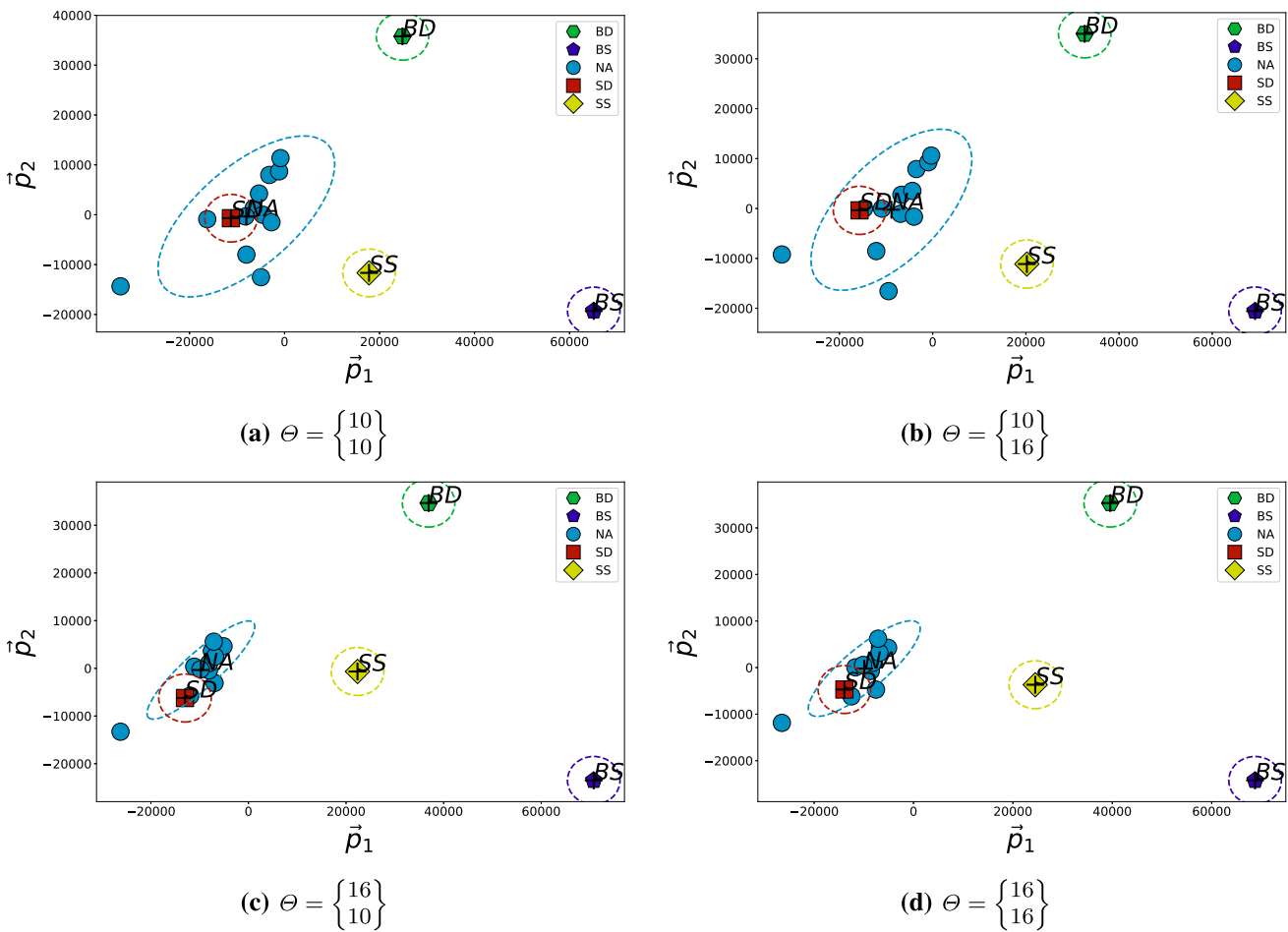
Fig. 15 The 2-dimensional projection of the tactile information generated from probing Ph-2 at varying depths and radii. The ellipses correspond to the distributions of the clusters based on their true inclusion types, at a distance of 2 standard deviations from their respective cluster center
