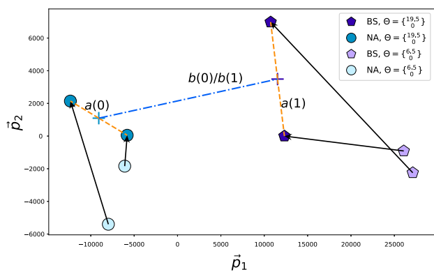
Fig. 10 The change in position for the 2D PCA projected NA and BS samples when probing the phantom vertically at a depth of 6.5 mm and 19.5 mm. The yellow and blue line show the two parameters on which the silhouette score is based, i.e. intra-cluster distance and nearest cluster distance respectively (Color figure online)
