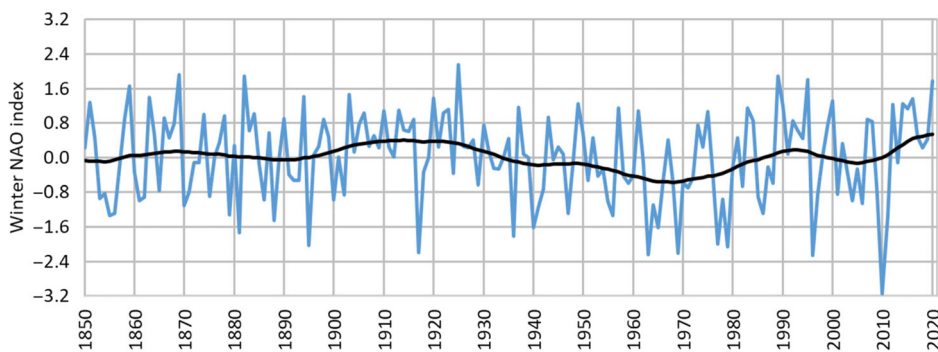
FIGURE 2 Winter NAO index based on standardized monthly mean pressure difference between stations in Gibraltar and south-west Iceland (see Annex 1 for details). Winter 2020 refers to the period December 2019–February 2020. Note that winter 2021 (December 2020–February 2021) will appear in State of the UK Climate 2021
