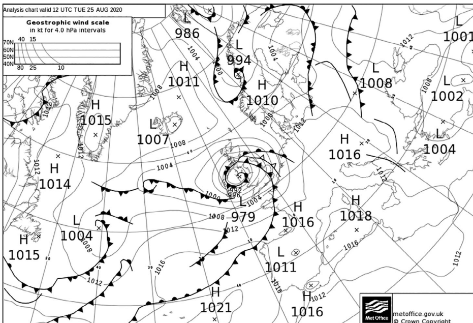
FIGURE 65 Analysis chart at 1200 UTC 25 August 2020
