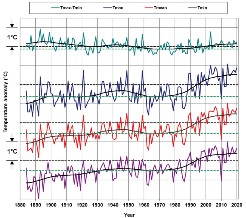
FIGURE 9 Annual T_{max} , T_{mean} and T_{min} ( ^{\circ}C ) for the UK, and T_{max} minus T_{min} , 1884–2020, expressed as anomalies relative to the 1981–2010 average. The hatched black line is the 1981–2010 long-term average. The lower hatched green line is the 1961–1990 long-term average. Light grey grid-lines represent anomalies of \pm 1^{\circ}C . The table provides average absolute values ( ^{\circ}C )
