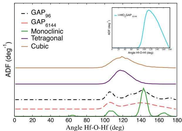
Fig. 5 Angle distribution functions (ADF) obtained from AIMD of pure phases of HfO 2 . GAP-predicted ADF for a-HfO 2 . The distributions have been shifted in vertical axes for clarity. The inset plots show the ADF from the GAP model for l-HfO 2 .
