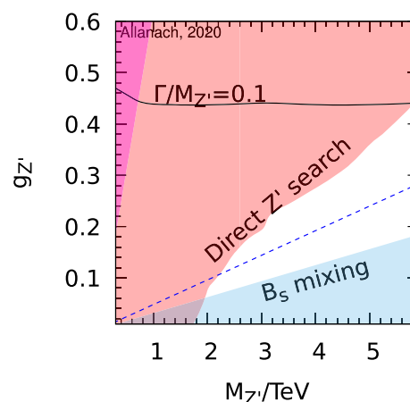
Fig. 8 Constraints upon (B_3 - L_2)eg for M_{Z'} > 300 GeV. \sin 2\theta_{sb} has been set as in (18) such that every point fits the NCBA's. The white region is currently allowed. The red and blue coloured regions show the 95% excluded regions from a 13 TeV 139 \text{ fb}^{-1} ATLAS Z' \rightarrow \mu^+ \mu^- search [77] and from B_s - \bar{B}_s mixing as in (20), respectively. The latter bound moves from the blue coloured region at lower C_9 = -0.65 to the region below the dashed line for central C_9 = -0.97 . The magenta region in the top left-hand corner shows the region ruled out by the neutrino trident process. The direct search bound is extrapolated above the solid curve and interpolated between ATLAS data below it, according to (28)
