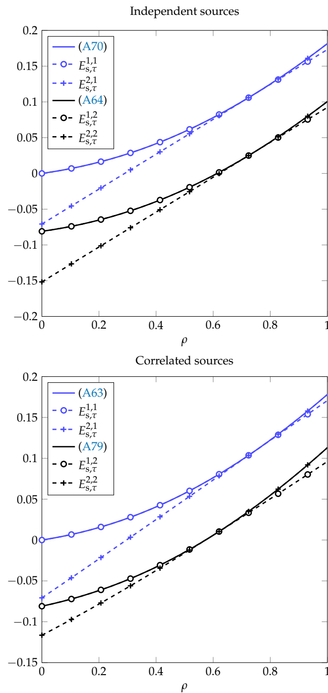
Figure A1. Example of the source functions E_{s,\tau}^{L,N} in Equation (A62) for independent and correlated sources and error type \tau \in \{1, 2\} .
