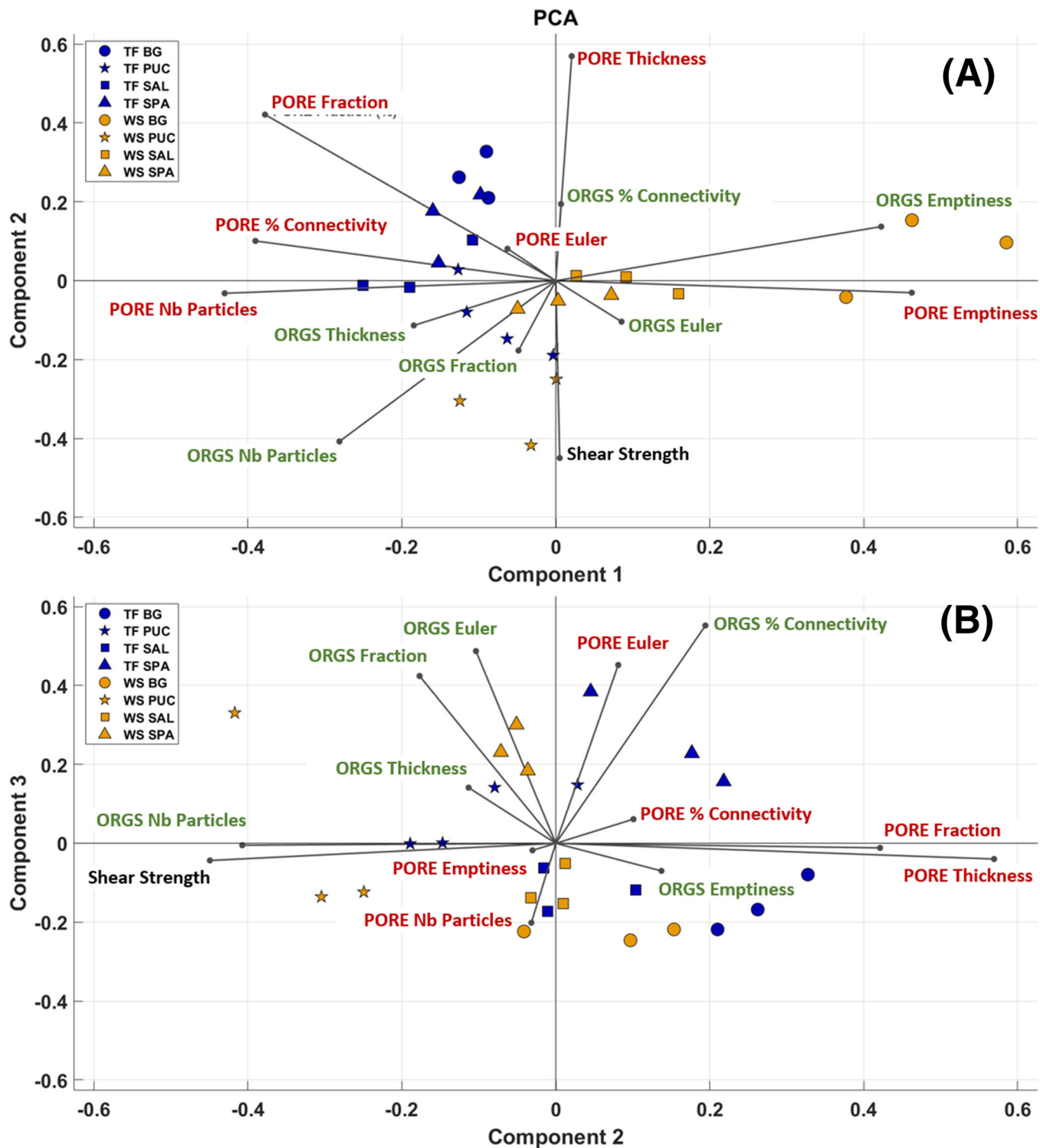
FIGURE 7 Biplot of the PCA: (A) PC 1 and 2; (B) PC 2 and 3. Pore parameters are represented in red, organic parameters in green and the shear strength in black
