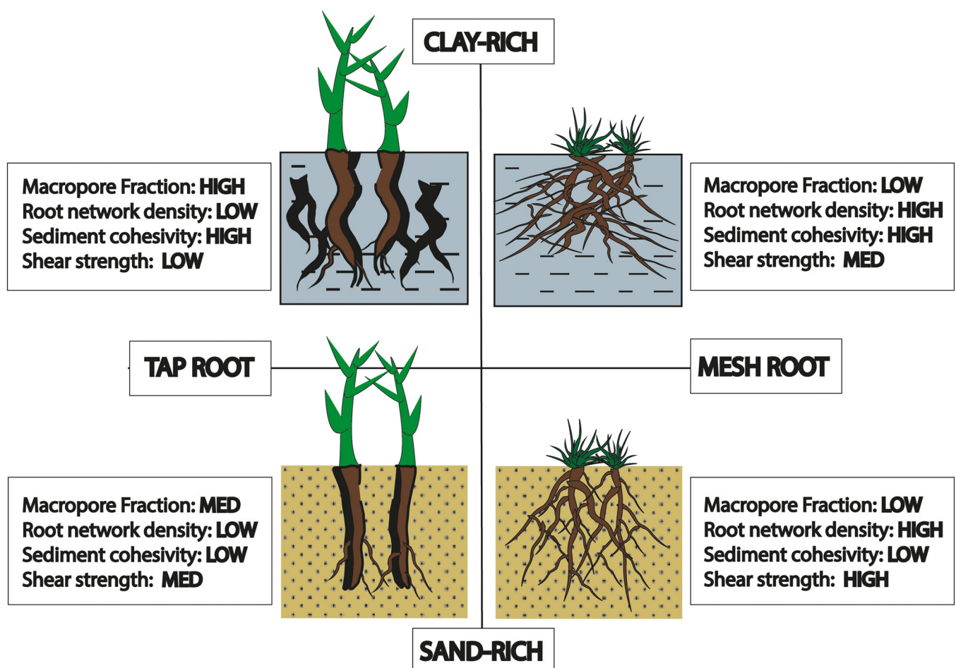
FIGURE 8 Schematic representation of root and macropore characteristics in different substrates and associated shear strength
