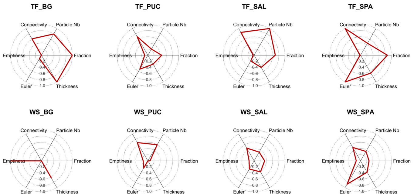
FIGURE 4 Spider plot representation of the topology of the macropores at all stations. Spider plot values have been normalized to the interval [0, 1]
