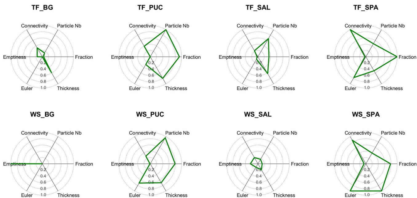
FIGURE 5 Spider plot representation of the topology of the organic matter elements at all stations. Spider plot values have been normalized to the interval [0, 1]
