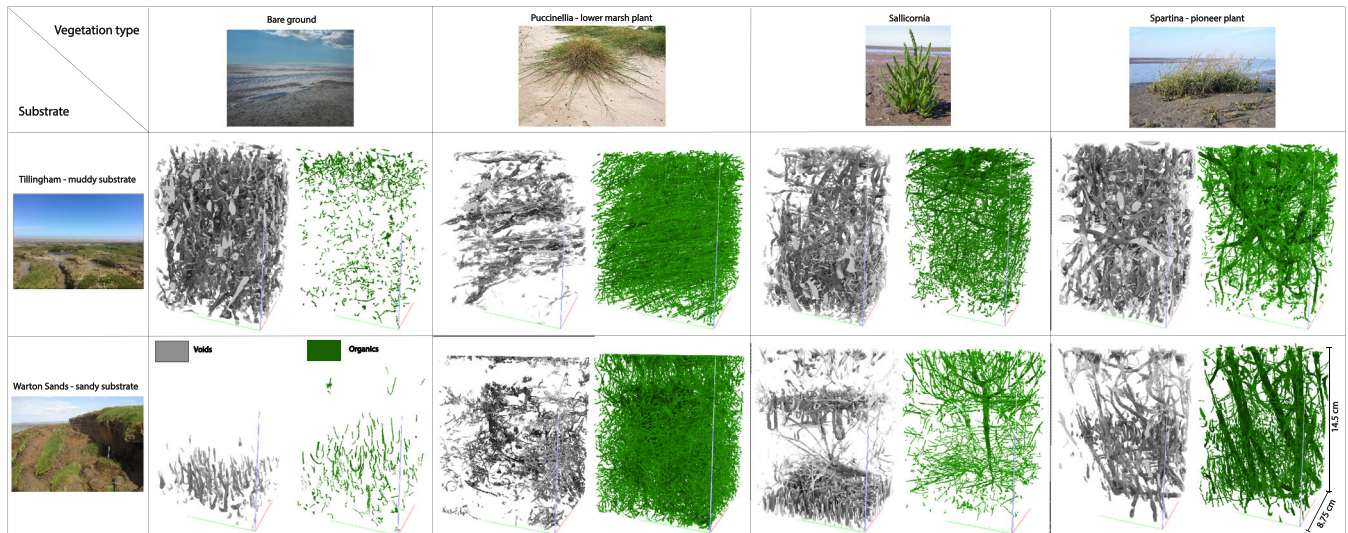
FIGURE 3 3D visualization of pores and organic matter elements for all stations. Sample size = 8.75 \times 8.75 \times 14.5 cm (see Figure A1 in the Appendix for a visualization of replicates)
