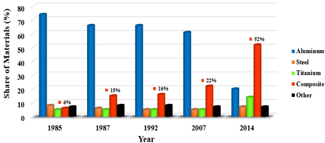
Figure 1. Used Materials in Aircraft Industry 1985-2014 [2].
