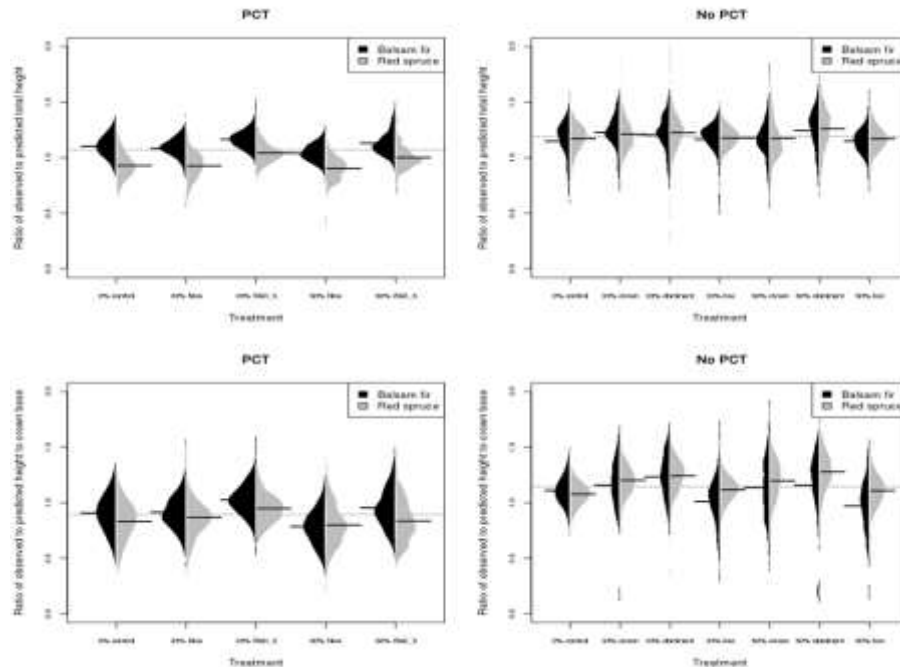
Figure 28 Ratio of observed to predicted height (top) and height to crown base (bottom) by PCT history, treatment type, and species for the CFRU Commercial Thinning Research Network. The predicted values were estimated using the regional equations of FVS- ACD.
