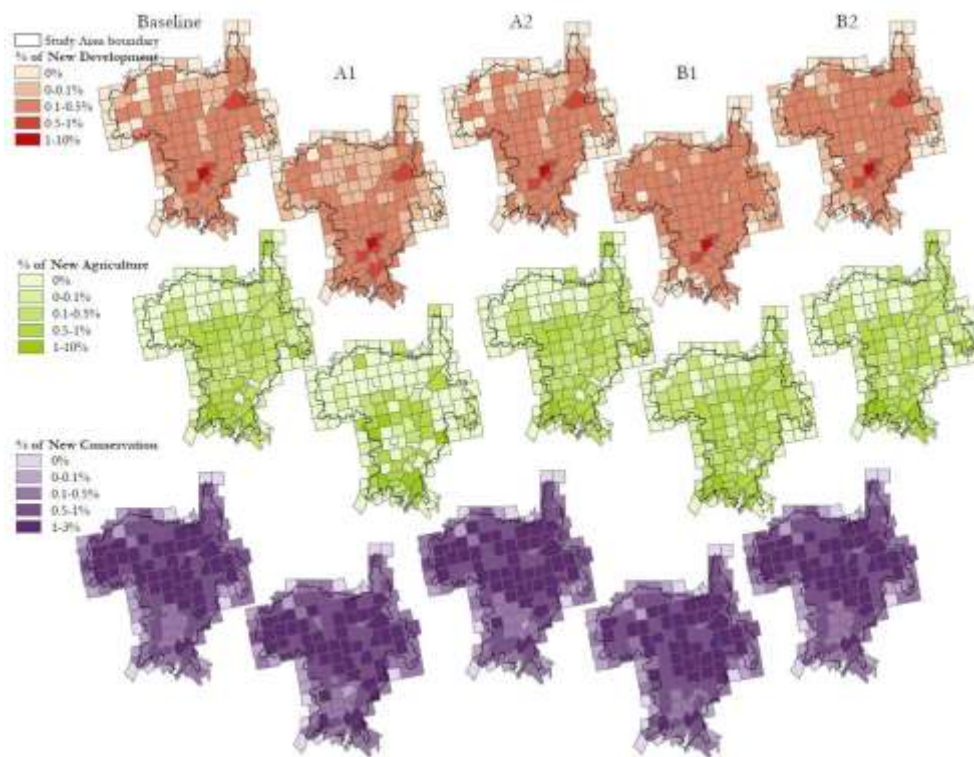
Figure 25 First phase of spatial analysis to determine extent of impact of development and changing land use on forest cover.
