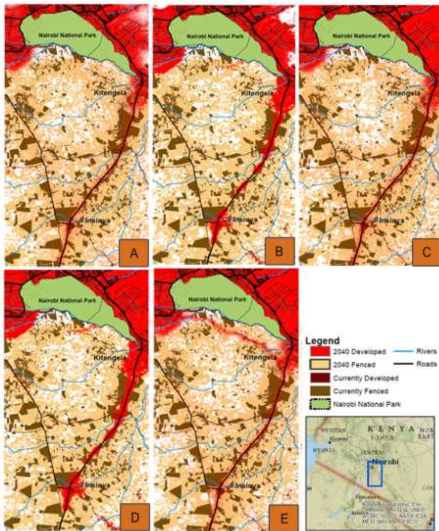
Figure 12 Nairobi Alternatives Futures Study development and fencing by 2040 in the region south of Nairobi National Park under five alternative futures scenarios. A: Current Trend; B: Trend with Smart Growth; C: Trend with Increased Development; D: Trend with Increased Smart Growth Development; E: Trend with Increased Development and Transportation
