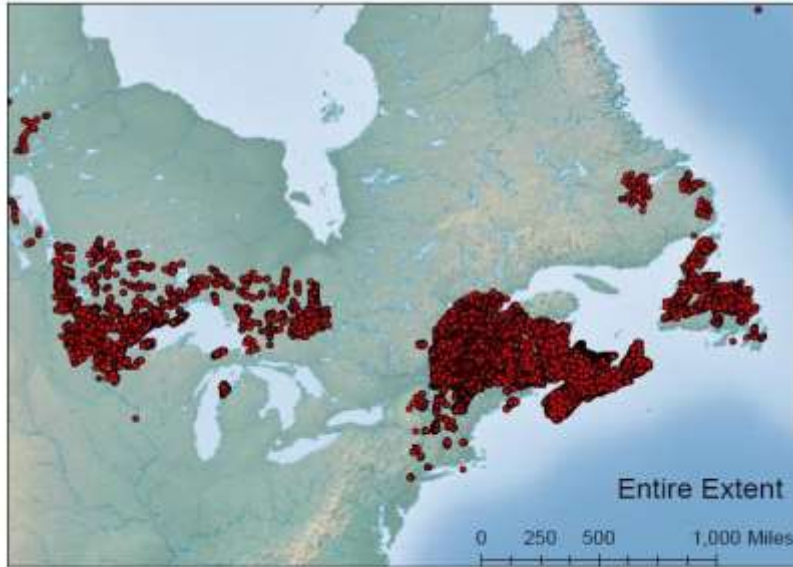
Figure 31 Compiled dataset of growth and yield plots.
