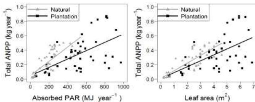
• Figure 20 Relationship between absorbed light (PAR) and total aboveground biomass growth, and leaf area and biomass growth of white spruce trees in plantations and in natural stands
