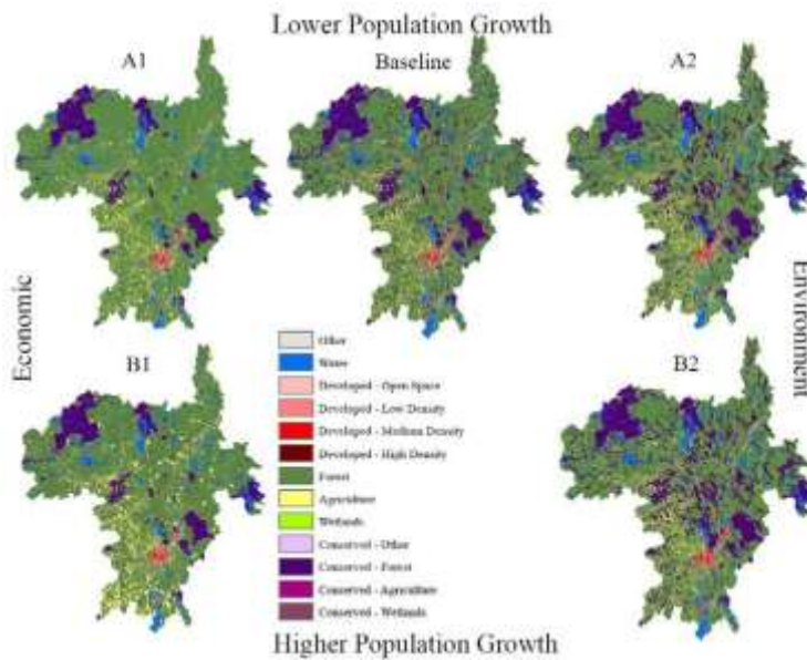
Figure 24. Scenario results for 2036 showing changes in land use categories.
