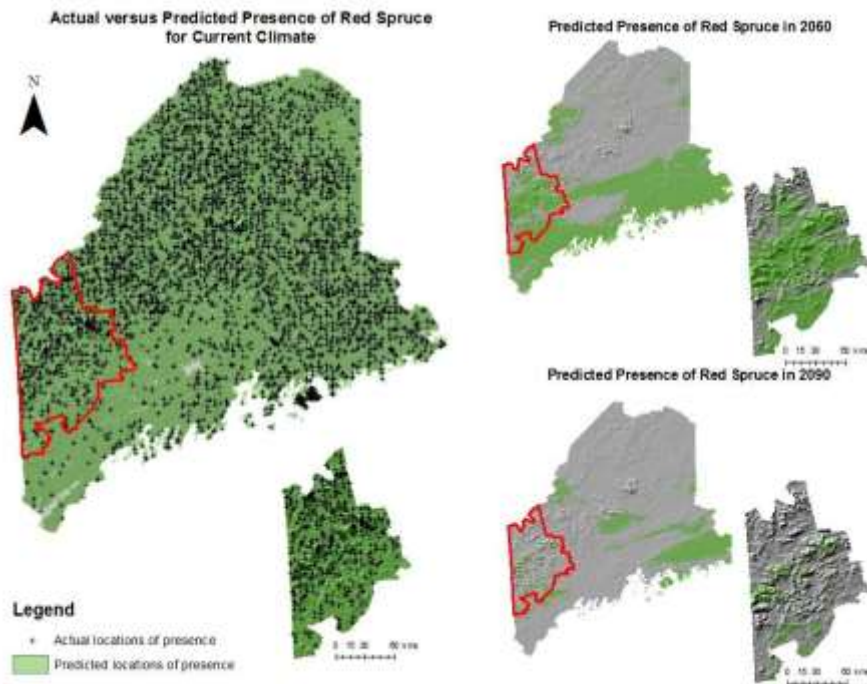
Figure 32 Predicted red spruce presence in present time, 2060, and 2090, at multiple scales. AUC for this model is .96. The Hadley Centre for Climate Prediction and Research B2 scenario was used for future predictions
