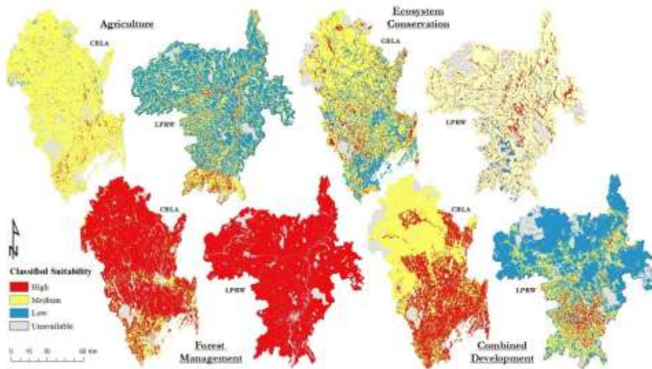
Figure 22 Complete suitability maps for both watersheds
