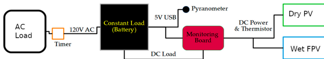
Figure 3. Wiring diagram for NanoDAQ monitoring board.
