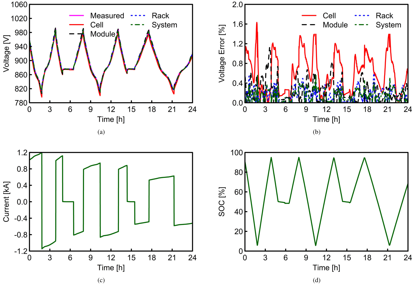
FIGURE 8. The BESS during dynamic charge and discharge between multiple SOC levels at 100%, 75% and 50% power rating (CycleB) showing: (a) The experimental and simulated battery system terminal voltage variation, (b) the percentage voltage error, (c) the discharge current, (d) and the SOC variation. The average error for the system and selected sub-components were considered to be within acceptable limits and the maximum percentage error was reported for the representative cell.
