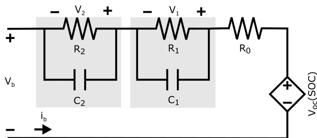
FIGURE 3. Equivalent circuit model for the battery system and its sub-components (racks, modules and cells) used for the study. Each parameter corresponds to the combination of cells connected in series and parallel.
