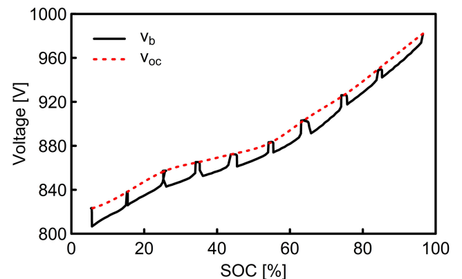
FIGURE 4. Battery system open circuit voltage. The BESS was pulse discharged (Cycle A), and the maximum dc terminal voltage ( v_b ) for defined SOC ranges when the output current approaches zero were used to estimate its open-circuit voltage ( v_{oc} ).
