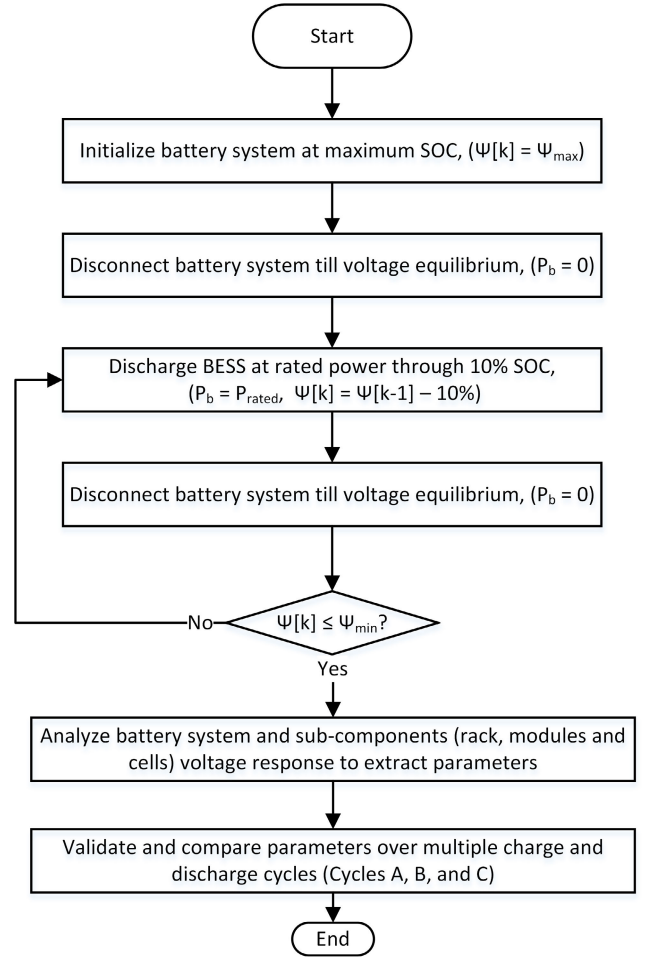
FIGURE 2. Flowchart for the experimental procedures employed in the proposed parameter extraction. The battery system is open-circuited or kept in the "float mode" in between tests in order to ensure voltage and chemical equilibrium among all cells.
