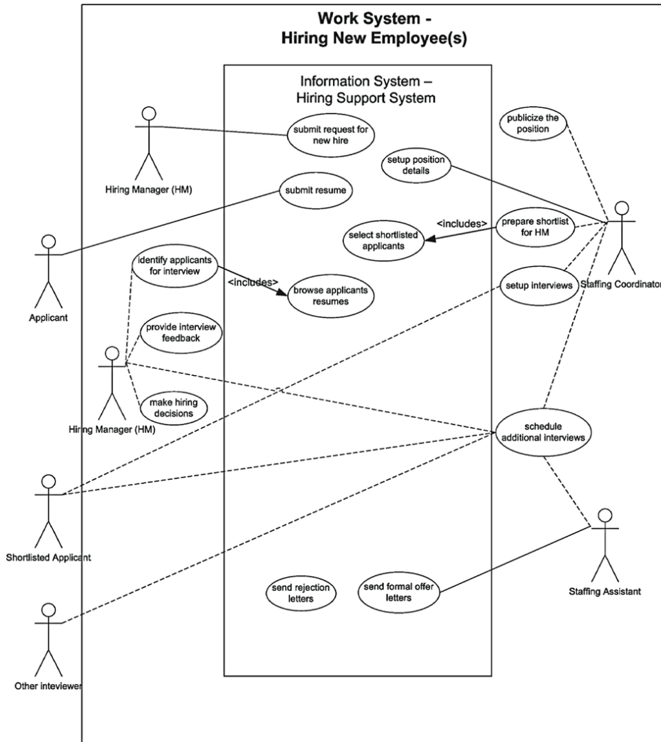
Figure 3. Example of an enhanced use case diagram
