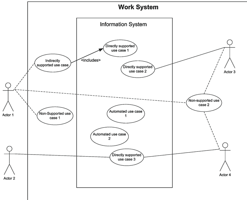
Figure 2. Enhanced use case diagram showing information system and work system boundaries
