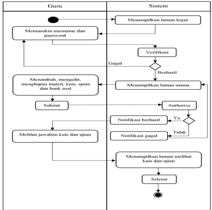
Gambar 4. Activity Diagram Guru
