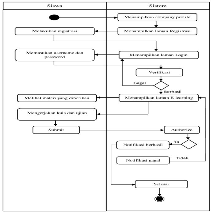
Gambar 5. Activity Diagram Siswa
