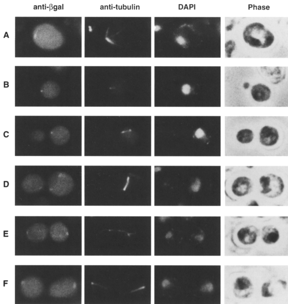
Figure 12. Localization of dhc1-β-galactosidase during the cell cycle. A wild-type strain containing plasmid pDLZ2 (lacZ fused at codon 3409 of DHC1, dhc1-2::lacZ ) was analyzed by indirect immunofluorescence. The panels moving left to right are cells stained with anti-β-gal, anti-tubulin, DAPI, and viewed by phase microscopy. Double labeled cells were visualized with FITC-labeled goat anti-mouse or anti-rabbit for β-gal and rhodamine conjugated goat anti-rat for tubulin staining. In single cells (A) and cells with small buds containing a pre-anaphase spindle (B and C) the hybrid protein is localized to a single dot at or near the spindle pole body proximal to the bud. As the spindle elongates (D) and the DNA separates (E) the hybrid protein is localized at or near both SPBs. At cytokinesis, the spot is observed at the periphery of the mother and daughter cells (F).
