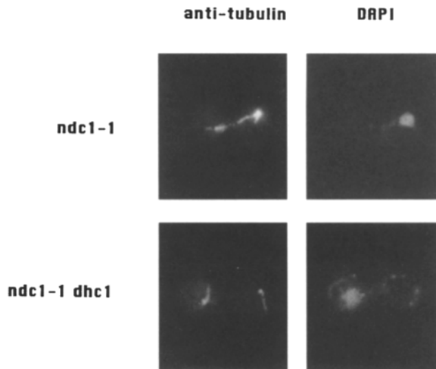
Figure 10. Spindle pole body migration in a ndc1-1 mutant. ndc1-1 and ndc1-1, dhc1Δ7 cells were grown to early logarithmic growth phase at 25°C before shifting to 14°C, the nonpermissive temperature for ndc1-1 , for 24 h. Cells arrest as large budded cells with a single nucleus. The cells were processed for immunofluorescence as described in the Materials and Methods. Left is the anti-tubulin immunofluorescence, right is DAPI staining. ( Top ) ndc1-1 . ( Bottom ) ndc1-1, dhc1Δ7 .
