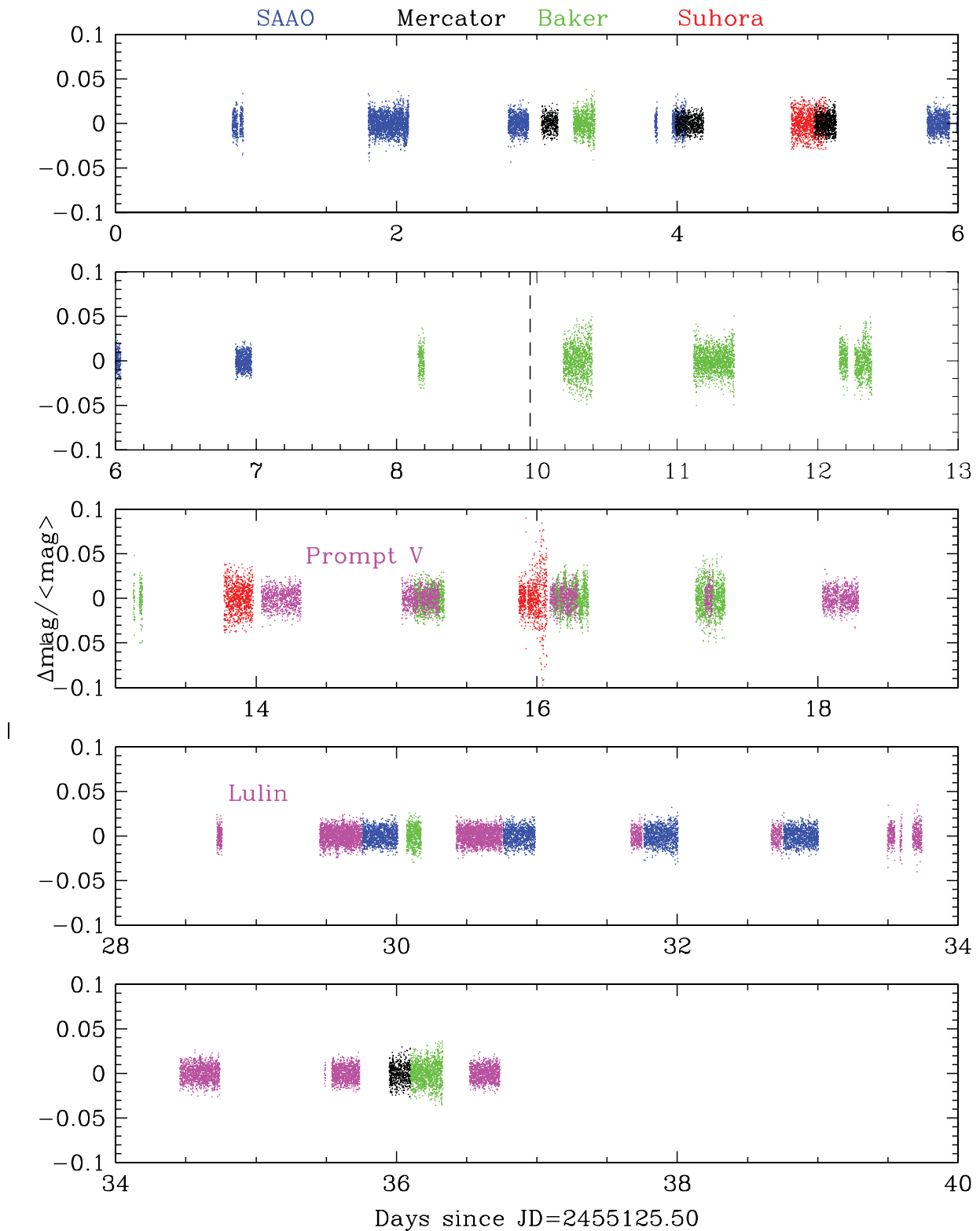
Figure 1. Light curves showing the 2009 data coverage. Each panel covers 6 d and the dashed vertical line indicates that day 9 was skipped as no data were collected. The top three panels are part 1 and the bottom two panels are part 2 of the campaign. Colour coded by observatory in the online version with the Prompt Observatory and Lulin Observatory sharing the same colour.
