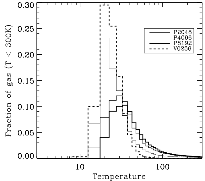
Figure 8. Fractional mass as a function of temperature in the cold phase (not limited to clumps). There is relatively more low-temperature ( T < 40 K) gas in model V0256 than in the PROTEUS models.
