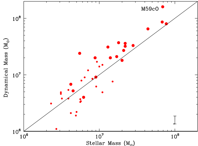
Figure 2. Dynamical vs stellar mass for the sample of Virgo, Fornax and CenA UCDs using data from Mieske et al. (2013). Larger circles denote objects with R_e > 10 pc. The diagonal solid line shows a 1:1 relation. A typical observational error bar is shown lower right. The Mieske et al. sample shows that below about 10^7 M_\odot UCDs scatter about the 1:1 relation, i.e. they are consistent with the total (dynamical) mass being due purely to stars. However, above this mass UCDs have systematically higher dynamical-to-stellar mass ratios. The larger-sized UCDs tend to also be those with the largest stellar masses. The massive UCD M59c0 is labelled.
