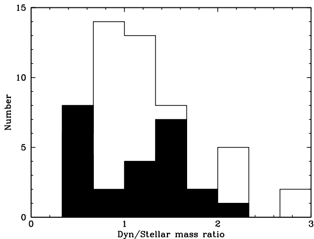
Figure 5. Histogram of dynamical-to-stellar mass ratio for low-mass ( < 10^7 M_{\odot} ) UCDs. The Mieske et al. (2013) sample (from Figure 2), shown as a filled histogram, shows a bimodal nature to the mass ratios. However, our enlarged sample (from Figure 3), shown by an open histogram, does not.
