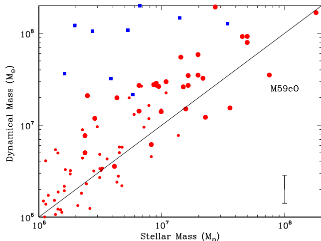
Figure 3. Dynamical vs stellar mass for the enlarged and revised sample of UCDs. Red circles denote UCDs, with larger circles for objects with R_e > 10 pc. Blue squares denote Local Group dSph galaxies. The diagonal solid line shows a 1:1 relation. A typical observational error bar is shown lower right. Excluding the dSph galaxies, our enlarged sample of UCDs shows the trend for elevated mass ratios as seen in the smaller Mieske et al. (2013) sample (Fig. 2), but does not support their claim for a bimodality in the mass ratios. The dynamical mass of M59cO is lower compared to the Mieske et al. sample due to the smaller velocity dispersion measured by N14.
