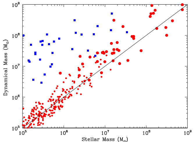
Figure 4. Dynamical vs stellar mass for the enlarged sample of UCDs and GCs. Red circles denote GCs and UCDs, with larger circles for objects with R_e > 10 pc. Blue squares denote Local Group dSph galaxies. The diagonal solid line shows a 1:1 relation. Globular clusters, with stellar masses typically less than 10^6 M_\odot , scatter evenly about the 1:1 relation indicating that their total (dynamical) mass is consistent with their stellar mass.
