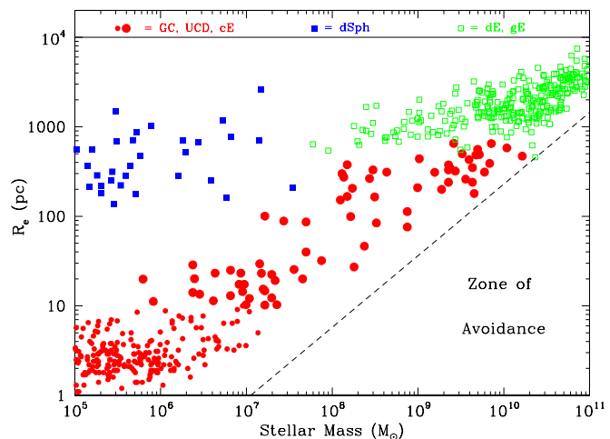
Figure 1. Size vs stellar mass for the entire sample of old, pressure supported systems with available central velocity dispersions. Blue squares denote Local Group dSph galaxies, and green open squares denote dE and gE galaxies. Red circles denote GCs, UCDs and cEs, with larger circles for objects with R_e > 10 pc. The diagonal dashed line demarks the constant surface density edge of the Zone of Avoidance, i.e. a high density region of parameter space that appears to be unoccupied. There is some overlap in size-mass parameter space between the traditional classification of different types of object.
