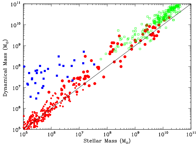
Figure 6. Dynamical vs stellar mass for the enlarged sample of GCs, UCDs, cEs and galaxies. Red circles denote GCs, UCDs and cEs, with larger circles for objects with R_e > 10 pc. Blue squares denote Local Group dSph galaxies, and green open squares denote dE and gE galaxies. The diagonal solid line shows a 1:1 relation. Although most UCDs/cEs with stellar masses around a few 10^8 M_{\odot} show systematically elevated mass ratios, the ratio returns to near unity for the most massive UCDs/cEs.
