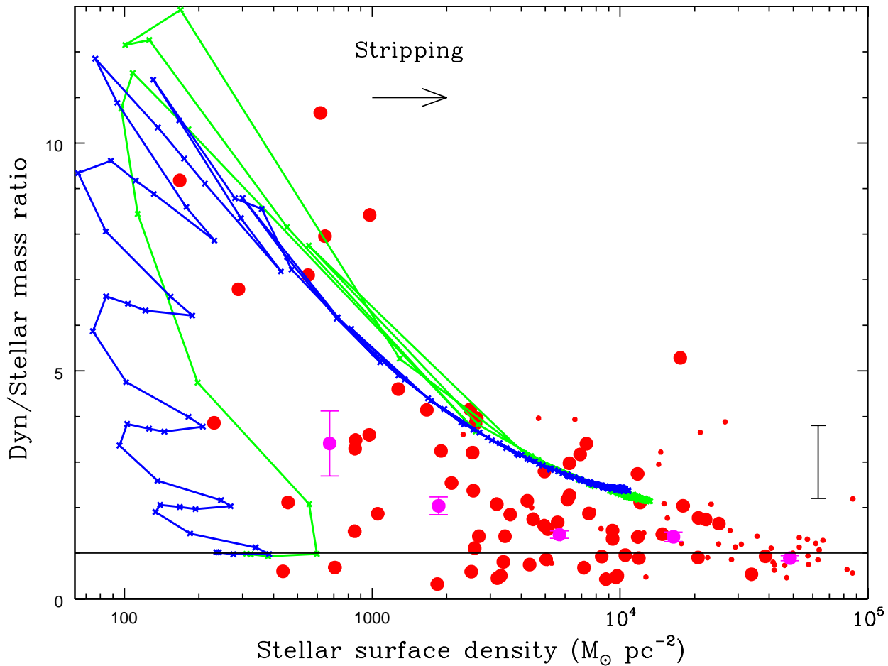
Figure 8. Dynamical-to-stellar mass ratio vs stellar surface density. Red circles show individual UCDs and cEs only, with larger circles for objects with R_e > 10 pc. Large magenta circles show the mean mass ratio (in bins of 0.5 dex) with errors on the mean. The solid black line shows the 1:1 relation of the mass ratio. A typical error bar for the whole sample is shown in the lower right. There is a general trend for decreasing mass ratios in the higher density systems. The blue and green tracks show the effects of tidal stripping on the mass ratio in 25 Myr steps for two dE progenitors (the tracks have been normalised to a mass ratio of unity at the start of the simulation, with \sigma_0 assumed to be constant) from the models of Pfeffer & Baumgardt (2013). The arrow shows the general direction of stripping. The stripping tracks show that the progenitors start with a relatively low average density but after a few hundred Myr the remnants become more dense as the nuclei increasingly dominate and the mass ratios get smaller as the stripping progresses.
